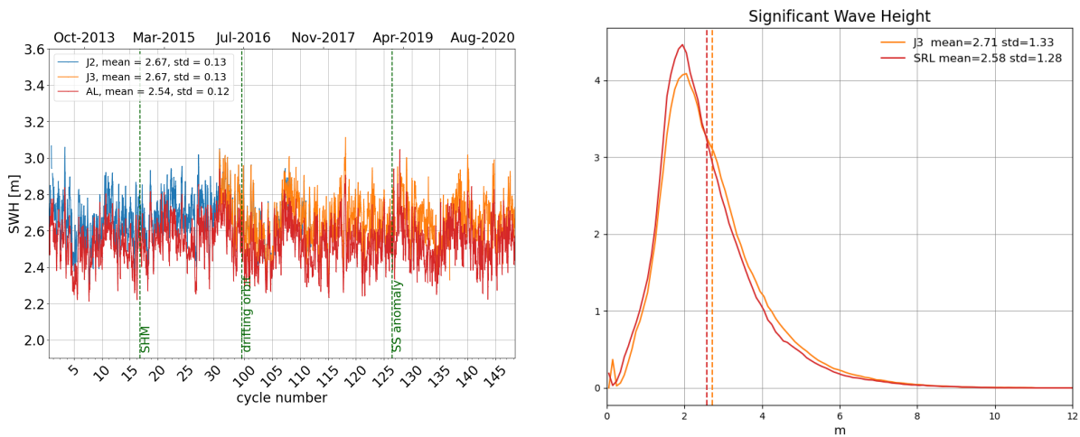
Figure 6: Daily monitoring of significant wave height for AltiKa (Ka-band) Jason-2 and Jason-3 (Ku-band) on the left and histogram for cycle 148 on the right (limited to 66^\circ latitude).
