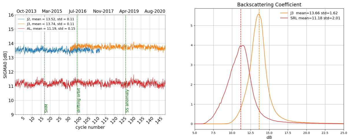
Figure 7: Daily monitoring of backscattering coefficient for Saral/AltiKa, Jason-2 and Jason-3 on the left and histogram for cycle 148 on the right (limited to 66° latitude).
