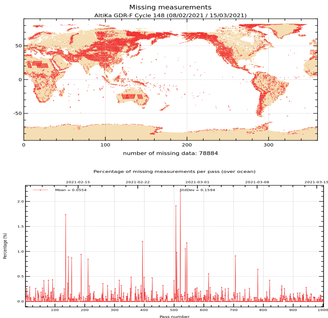
Figure 1: Map of missing measurements for cycle 148 on top. Monitoring of percentage of missing ocean measurements per pass on bottom.
