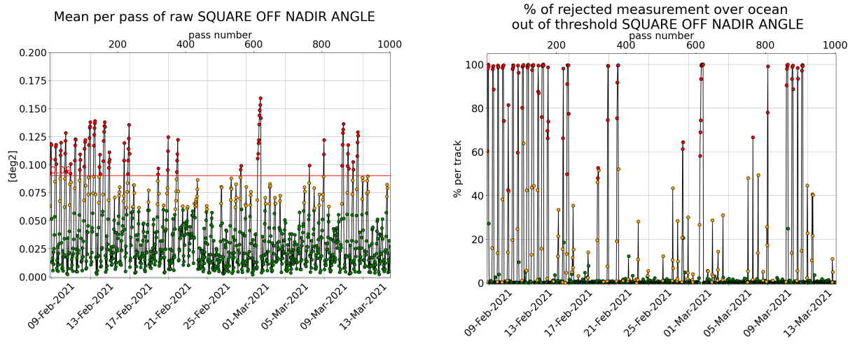
Figure 3: [left] Mispointing cycle 148, [right] Percentage of rejected measurement by threshold on square off-nadir angle.
