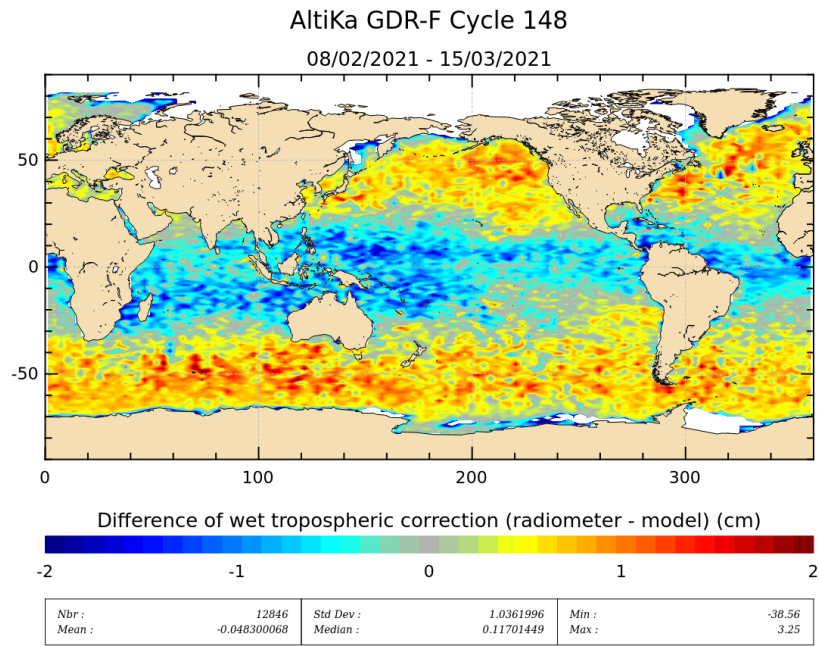
Figure 11: Mean of wet troposphere correction difference (Radiometer-ECMWF model) for cycle 148.
