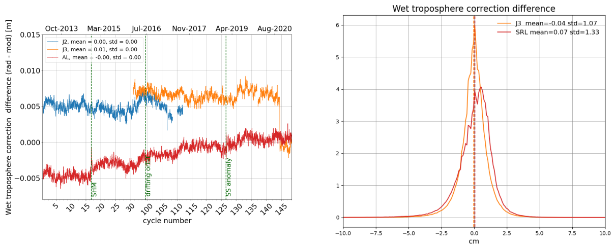
Figure 12: Daily monitoring of wet troposphere differences (Radiometer-ECMWF model) for Saral/AltiKa Jason-2 and Jason-3 (left) and histogram on the right (limited to 66° latitude) for cycle 148 .
