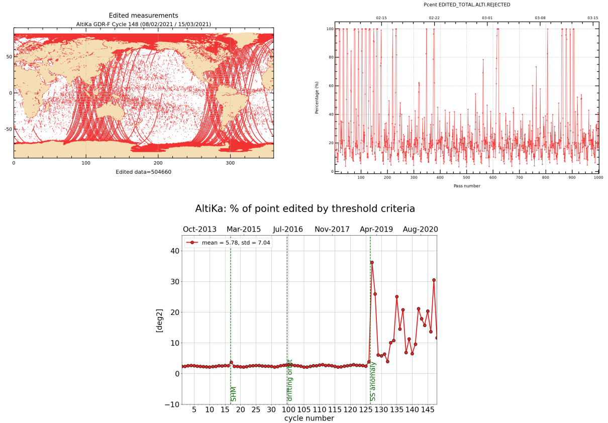
Figure 2: Rejected measurements on thresholds criteria : Cycle 148, map and monitoring of % of rejected measurements per track (top), whole time serie / % of rejected measurements per cycle (bottom).
