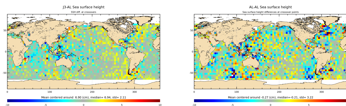
Figure 14: Mean of multi-mission SSH and mono-mission SSH differences at crossovers for cycle 148.
