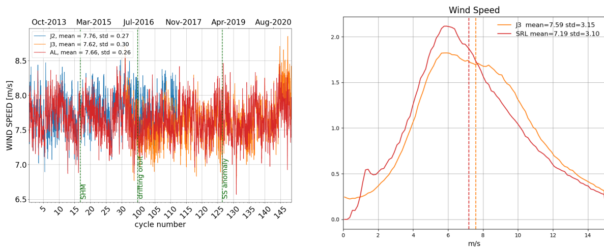
Figure 10: Daily monitoring of altimeter wind speed for Saral/AltiKa, Jason-2 and Jason-3 on the left and histogram for cycle 148 on the right (limited to 66° latitude).
