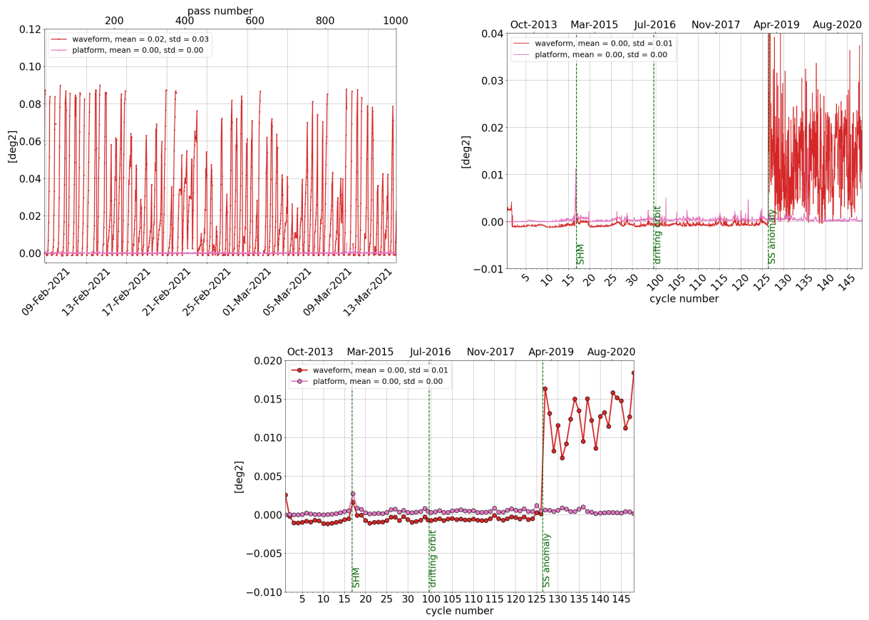
Figure 13: Monitoring per pass for cycle 148 (left), daily monitoring(right) and cyclic monitoring (bottom) of SARAL/AltiKa's mispointing angle: comparison between the one derived from waveform retracking and the one measured by platform startrackers.
