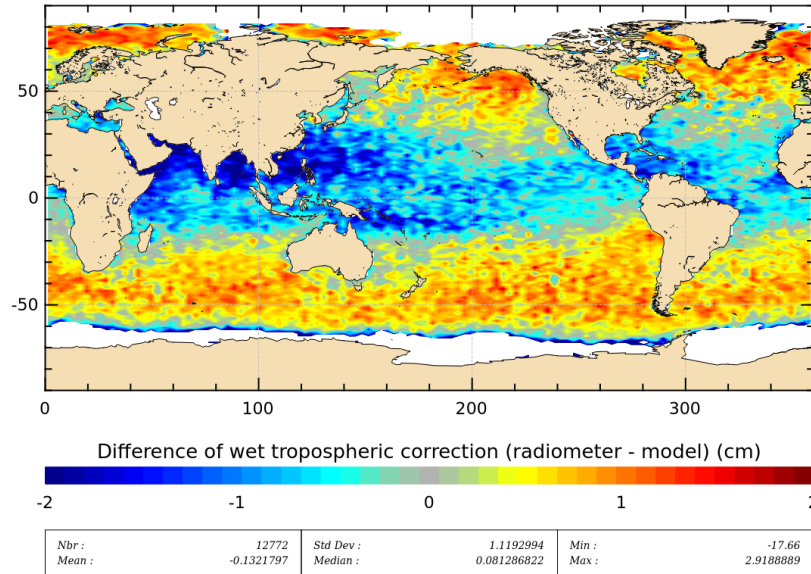
Figure 11: Mean of wet troposphere correction difference (Radiometer-ECMWF model) for cycle 152.
