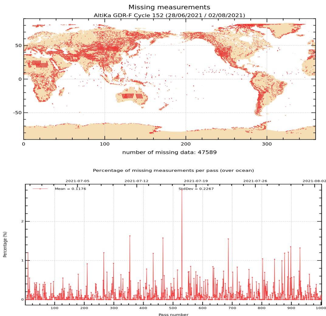
Figure 1: Map of missing measurements for cycle 152 on top. Monitoring of percentage of missing ocean measurements per pass on bottom.
