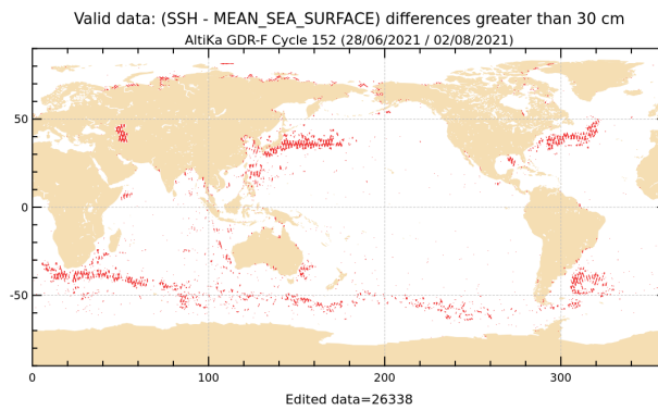
Figure 20: SLA higher than 30 cm for cycle 152.
