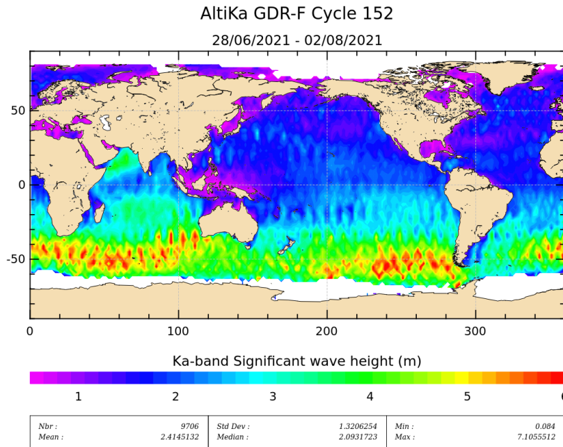
Figure 5: Significant wave height for cycle 152.
