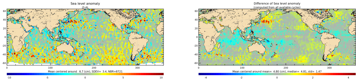
Figure 21: Jason-3 – Saral/AltiKa SLA differences for cycle 152 (left) and averaged over the whole Saral/AltiKa period (right).
