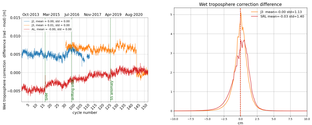
Figure 12: Daily monitoring of wet troposphere differences (Radiometer-ECMWF model) for Saral/AltiKa Jason-2 and Jason-3 (left) and histogram on the right (limited to 66° latitude) for cycle 152 .
