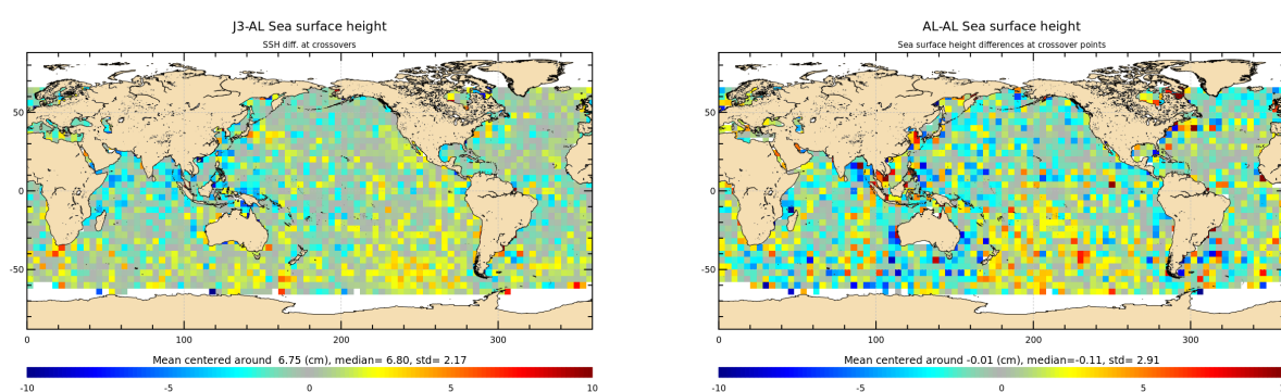
Figure 14: Mean of multi-mission SSH and mono-mission SSH differences at crossovers for cycle 152.
