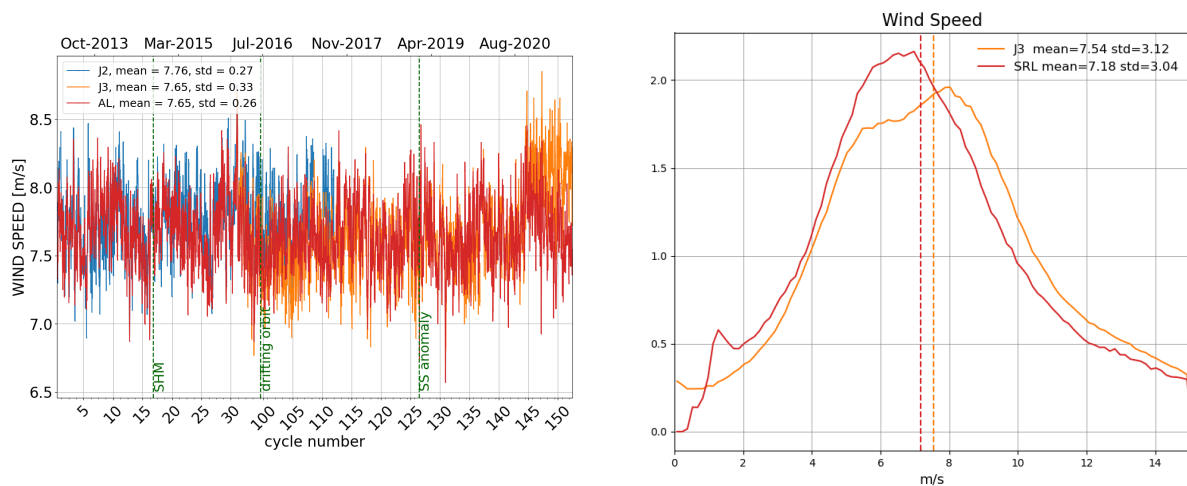
Figure 10: Daily monitoring of altimeter wind speed for Saral/AltiKa, Jason-2 and Jason-3 on the left and histogram for cycle 152 on the right (limited to 66° latitude).
