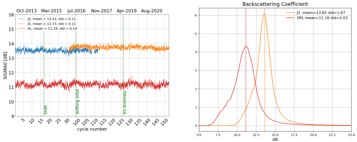
Figure 7: Daily monitoring of backscattering coefficient for Saral/AltiKa, Jason-2 and Jason-3 on the left and histogram for cycle 152 on the right (limited to 66° latitude).
