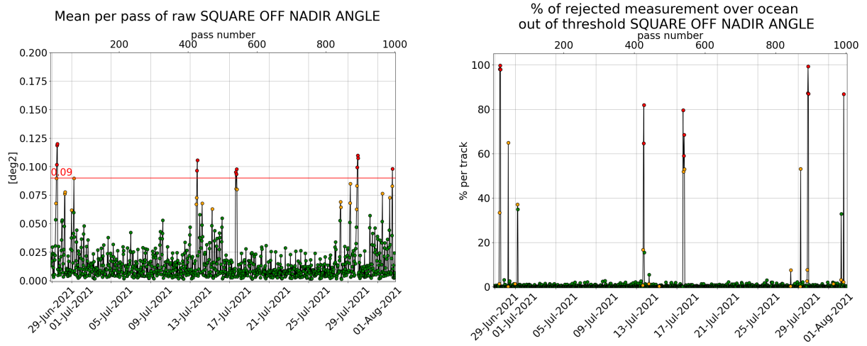
Figure 3: [left] Mispointing cycle 152, [right] Percentage of rejected measurement by threshold on square off-nadir angle.
