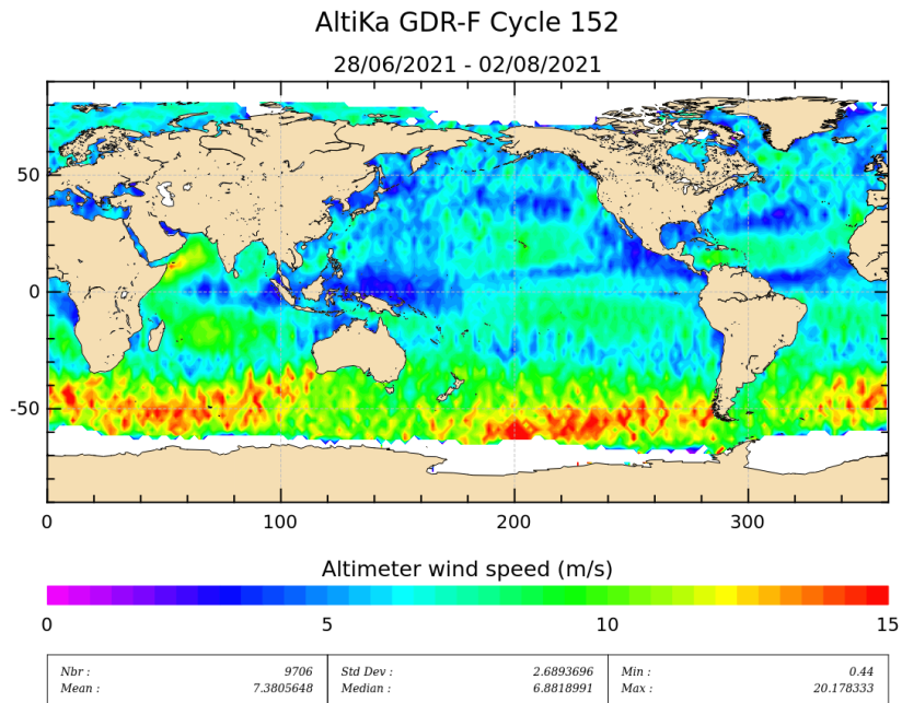
Figure 9: Altimeter wind speed for cycle 152.
