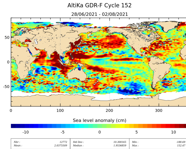
Figure 19: Sea level anomaly relative to MSS for cycle 152.
