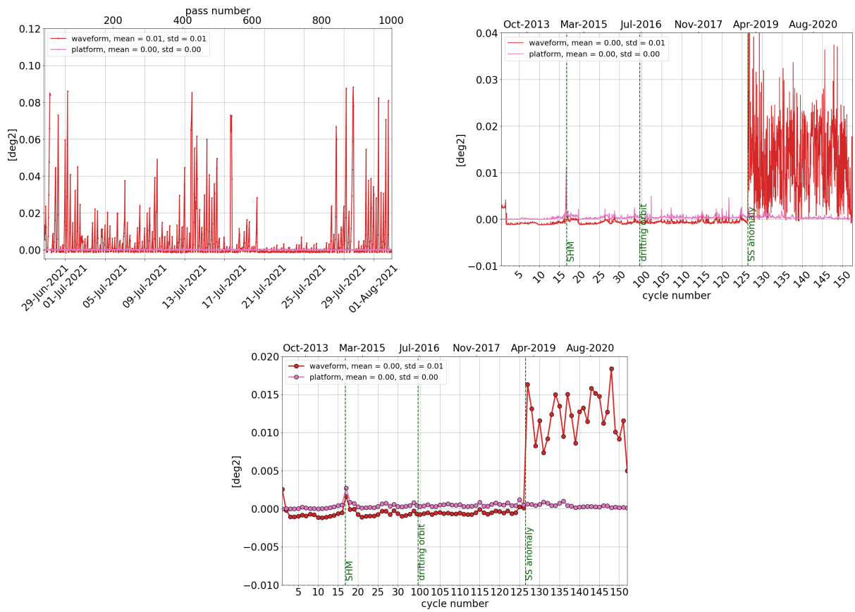
Figure 13: Monitoring per pass for cycle 152 (left), daily monitoring(right) and cyclic monitoring (bottom) of SARAL/AltiKa's mispointing angle: comparison between the one derived from waveform retracking and the one measured by platform startrackers.
