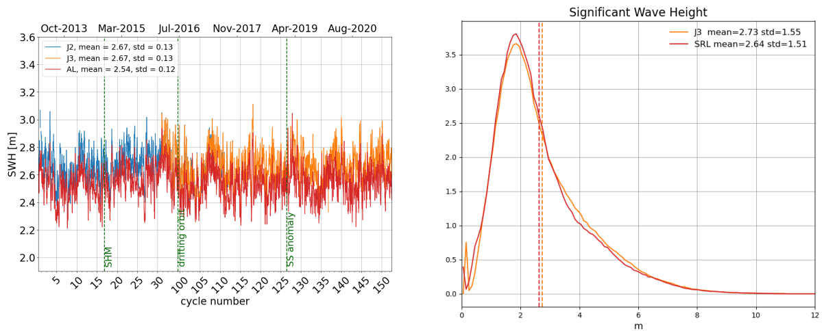
Figure 6: Daily monitoring of significant wave height for AltiKa (Ka-band) Jason-2 and Jason-3 (Ku-band) on the left and histogram for cycle 152 on the right (limited to 66^\circ latitude).
