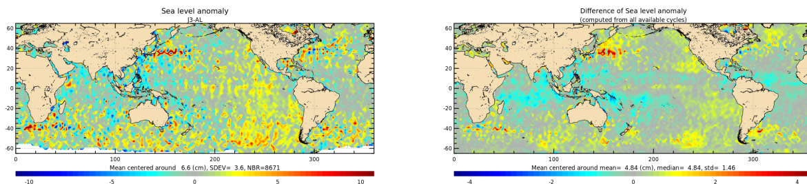
Figure 21: Jason-3 – Saral/AltiKa SLA differences for cycle 153 (left) and averaged over the whole Saral/AltiKa period (right).
