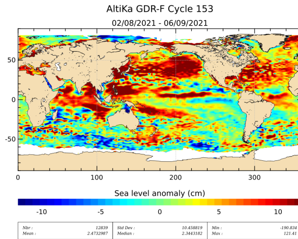
Figure 19: Sea level anomaly relative to MSS for cycle 153.
