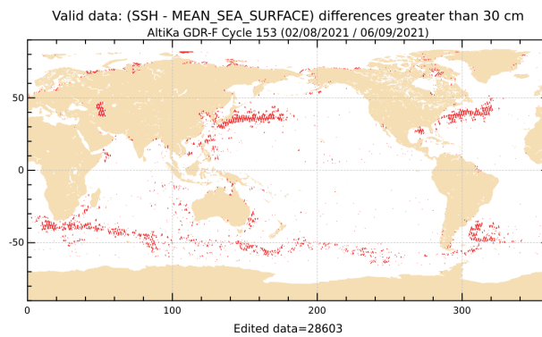
Figure 20: SLA higher than 30 cm for cycle 153.
