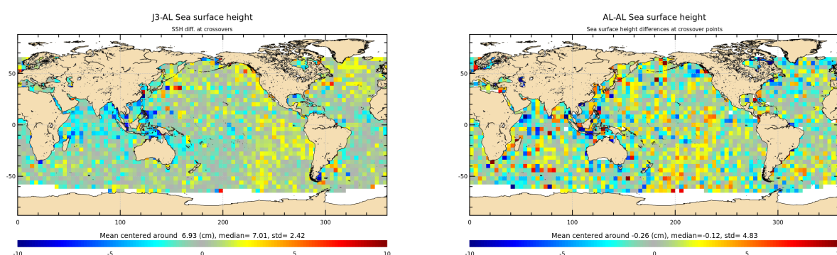
Figure 14: Mean of multi-mission SSH and mono-mission SSH differences at crossovers for cycle 155.
