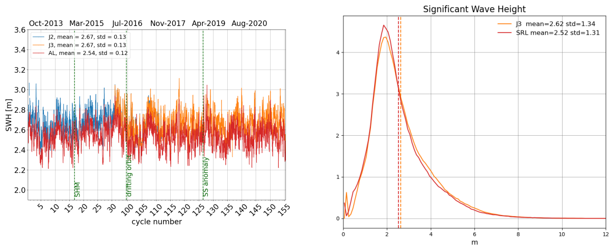
Figure 6: Daily monitoring of significant wave height for AltiKa (Ka-band) Jason-2 and Jason-3 (Ku-band) on the left and histogram for cycle 155 on the right (limited to 66° latitude).
