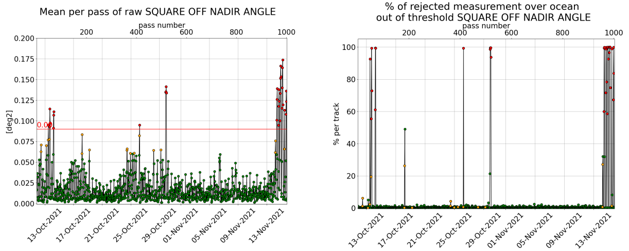
Figure 3: [left] Mispointing cycle 155, [right] Percentage of rejected measurement by threshold on square off-nadir angle.
