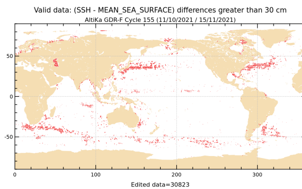
Figure 20: SLA higher than 30 cm for cycle 155.
