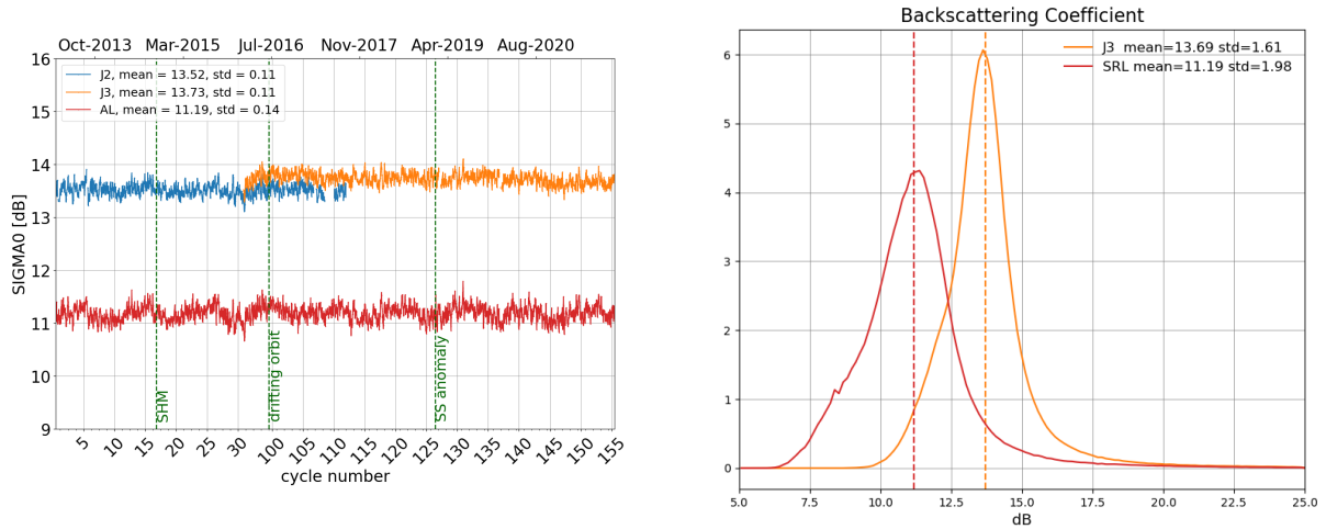
Figure 7: Daily monitoring of backscattering coefficient for Saral/AltiKa, Jason-2 and Jason-3 on the left and histogram for cycle 155 on the right (limited to 66° latitude).
