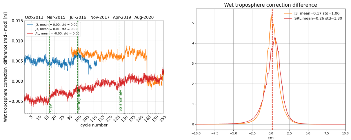
Figure 12: Daily monitoring of wet troposphere differences (Radiometer-ECMWF model) for Saral/AltiKa Jason-2 and Jason-3 (left) and histogram on the right (limited to 66° latitude) for cycle 155 .
