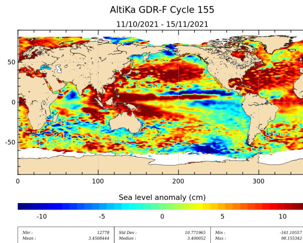
Figure 19: Sea level anomaly relative to MSS for cycle 155.
