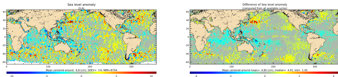
Figure 21: Jason-3 – Saral/AltiKa SLA differences for cycle 155 (left) and averaged over the whole Saral/AltiKa period (right).
