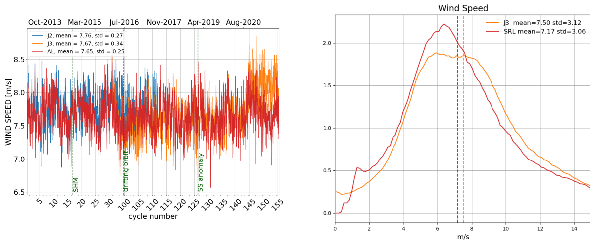
Figure 10: Daily monitoring of altimeter wind speed for Saral/AltiKa, Jason-2 and Jason-3 on the left and histogram for cycle 155 on the right (limited to 66° latitude).
