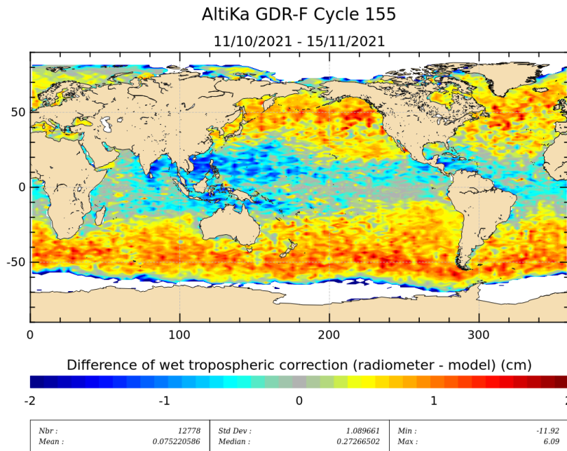
Figure 11: Mean of wet troposphere correction difference (Radiometer-ECMWF model) for cycle 155.
