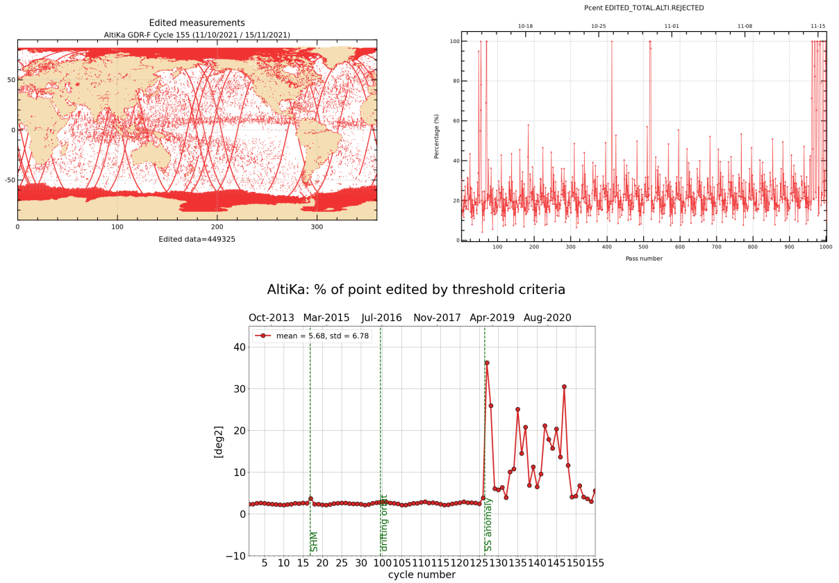
Figure 2: Rejected measurements on thresholds criteria : Cycle 155, map and monitoring of % of rejected measurements per track (top), whole time serie / % of rejected measurements per cycle (bottom).
