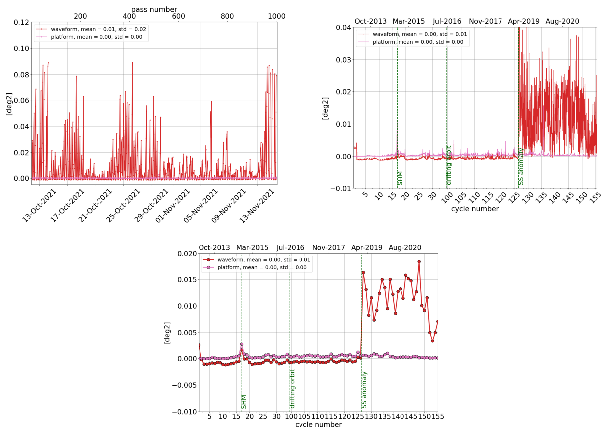
Figure 13: Monitoring per pass for cycle 155 (left), daily monitoring (right) and cyclic monitoring (bottom) of SARAL/AltiKa's mispointing angle: comparison between the one derived from waveform retracking and the one measured by platform startrackers.
