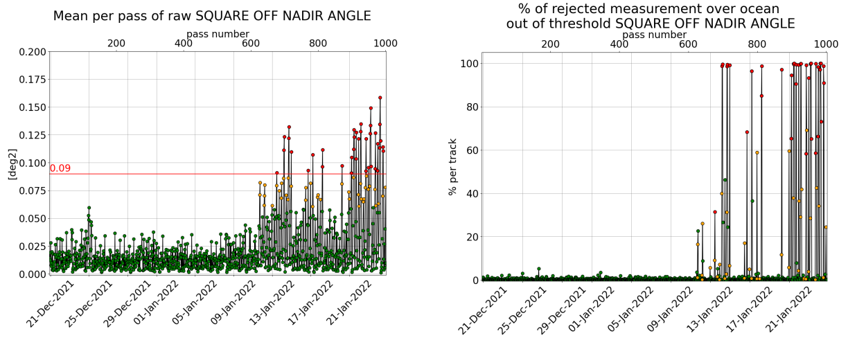
Figure 3: [left] Mispointing cycle 157, [right] Percentage of rejected measurement by threshold on square off-nadir angle.
