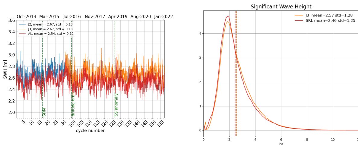
Figure 6: Daily monitoring of significant wave height for AltiKa (Ka-band) Jason-2 and Jason-3 (Ku-band) on the left and histogram for cycle 157 on the right (limited to 66^\circ latitude).
