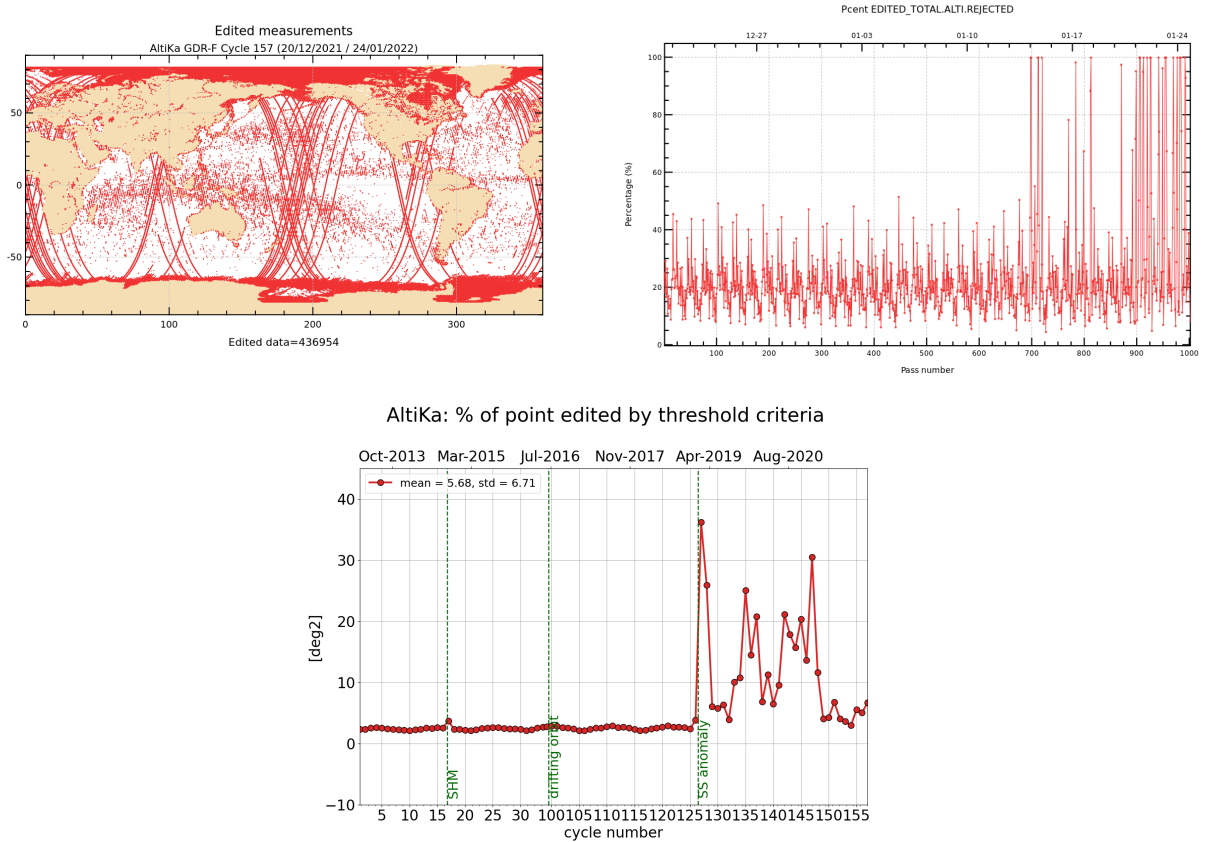
Figure 2: Rejected measurements on thresholds criteria : Cycle 157, map and monitoring of % of rejected measurements per track (top), whole time serie / % of rejected measurements per cycle (bottom).
