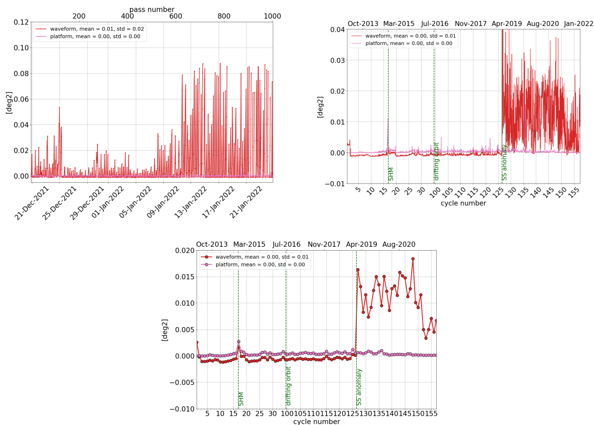
Figure 13: Monitoring per pass for cycle 157 (left), daily monitoring (right) and cyclic monitoring (bottom) of SARAL/AltiKa's mispointing angle: comparison between the one derived from waveform retracking and the one measured by platform startrackers.
