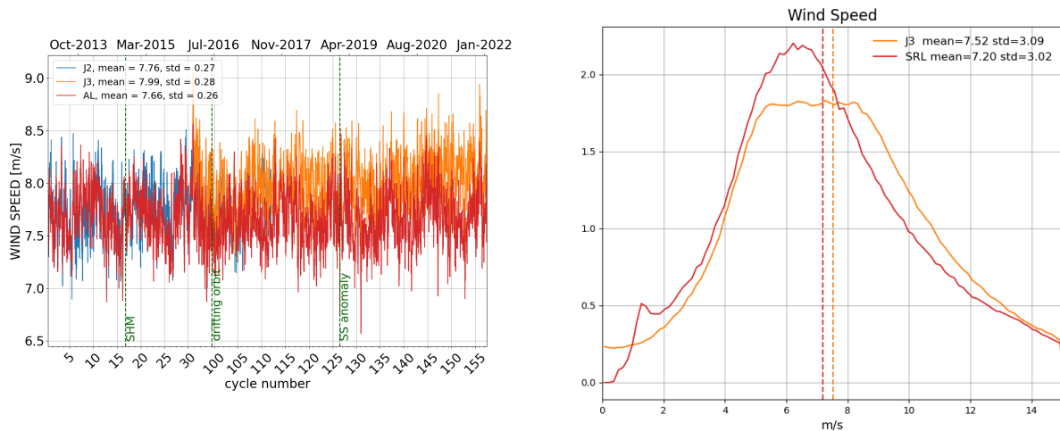
Figure 10: Daily monitoring of altimeter wind speed for Saral/AltiKa, Jason-2 and Jason-3 on the left and histogram for cycle 157 on the right (limited to 66° latitude).
