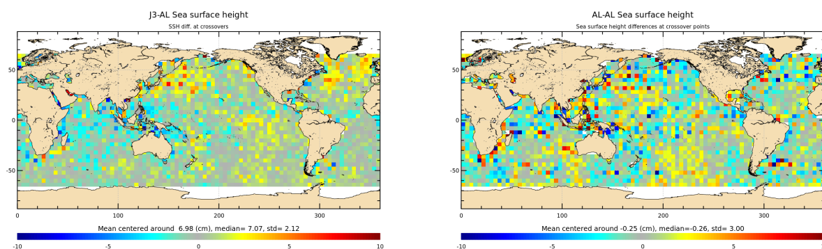
Figure 14: Mean of multi-mission SSH and mono-mission SSH differences at crossovers for cycle 157.
