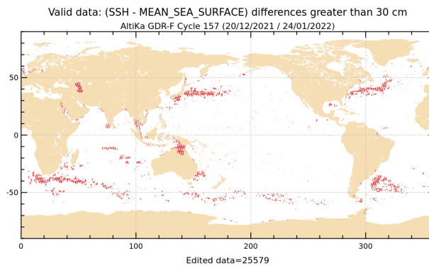
Figure 20: SLA higher than 30 cm for cycle 157.
