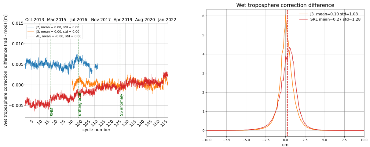
Figure 12: Daily monitoring of wet troposphere differences (Radiometer-ECMWF model) for Saral/AltiKa Jason-2 and Jason-3 (left) and histogram on the right (limited to 66° latitude) for cycle 157 .
