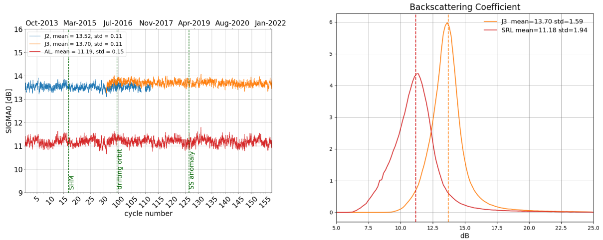
Figure 7: Daily monitoring of backscattering coefficient for Saral/AltiKa, Jason-2 and Jason-3 on the left and histogram for cycle 157 on the right (limited to 66° latitude).
