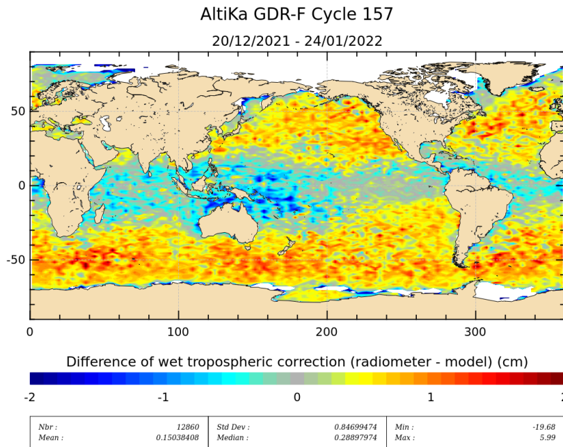
Figure 11: Mean of wet troposphere correction difference (Radiometer-ECMWF model) for cycle 157.
