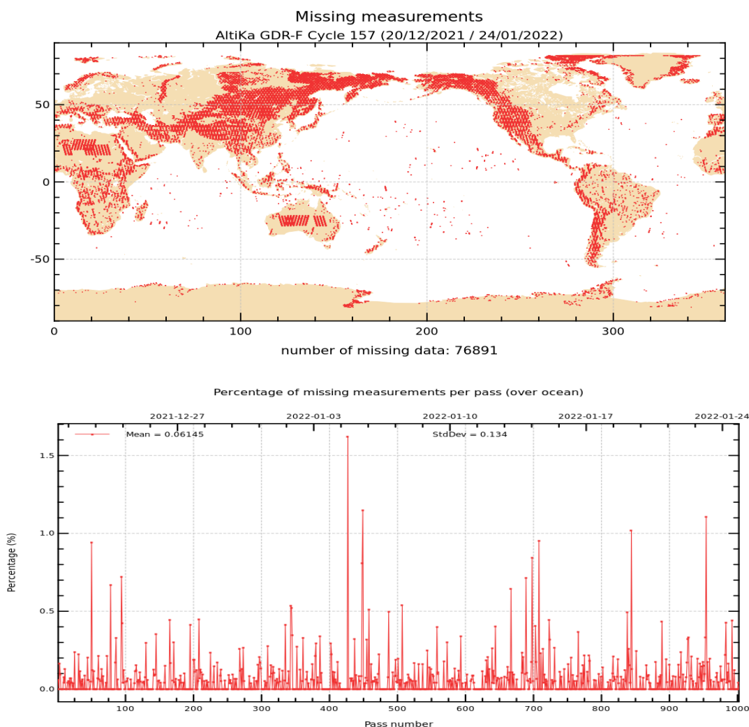
Figure 1: Map of missing measurements for cycle 157 on top. Monitoring of percentage of missing ocean measurements per pass on bottom.
