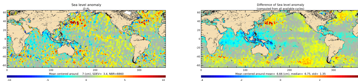
Figure 21: Jason-3 – Saral/AltiKa SLA differences for cycle 157 (left) and averaged over the whole Saral/AltiKa period (right).
