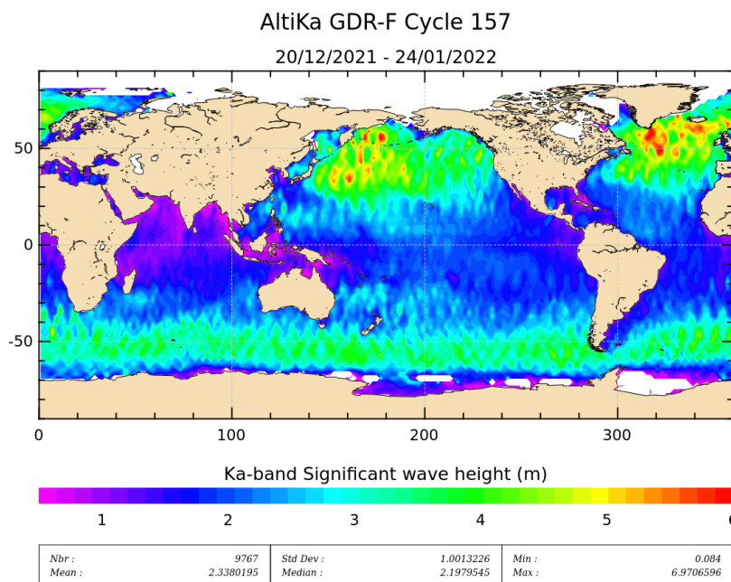
Figure 5: Significant wave height for cycle 157.
