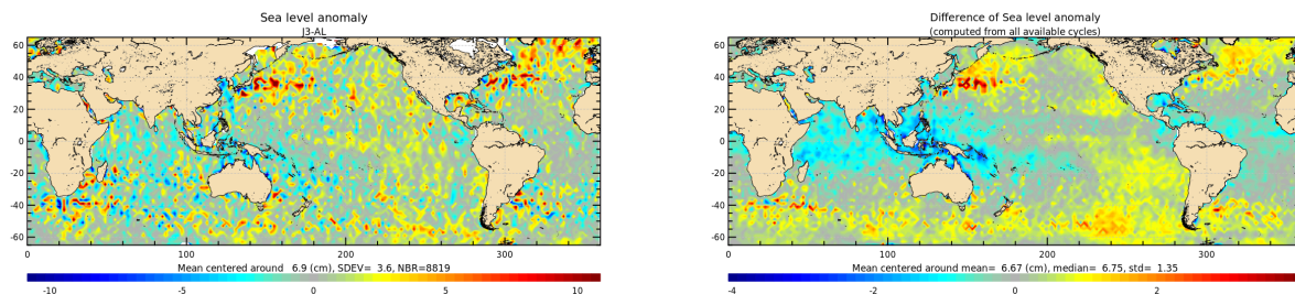
Figure 22: Jason-3 – Saral/AltiKa SLA differences for cycle 158 (left) and averaged over the whole Saral/AltiKa period (right).
