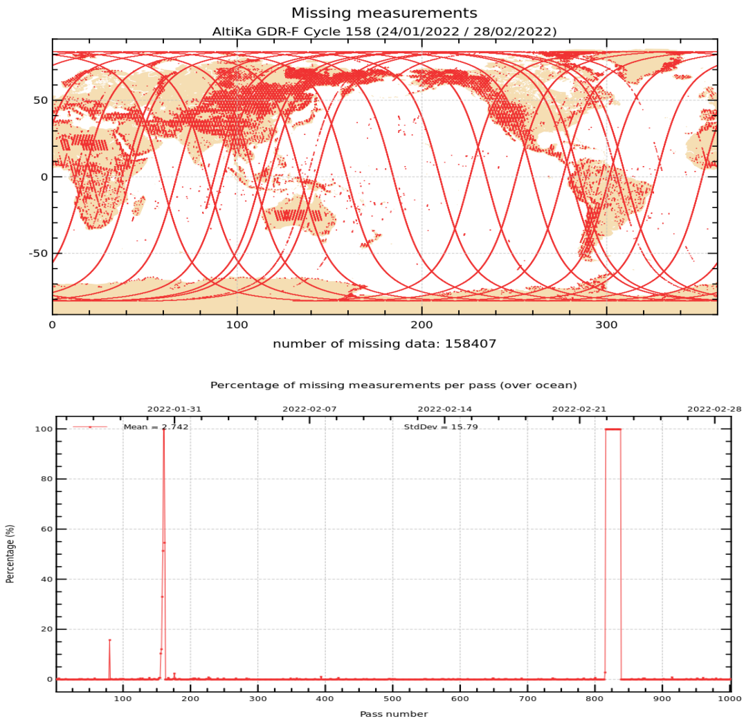
Figure 1: Map of missing measurements for cycle 158 on top. Monitoring of percentage of missing ocean measurements per pass on bottom.
