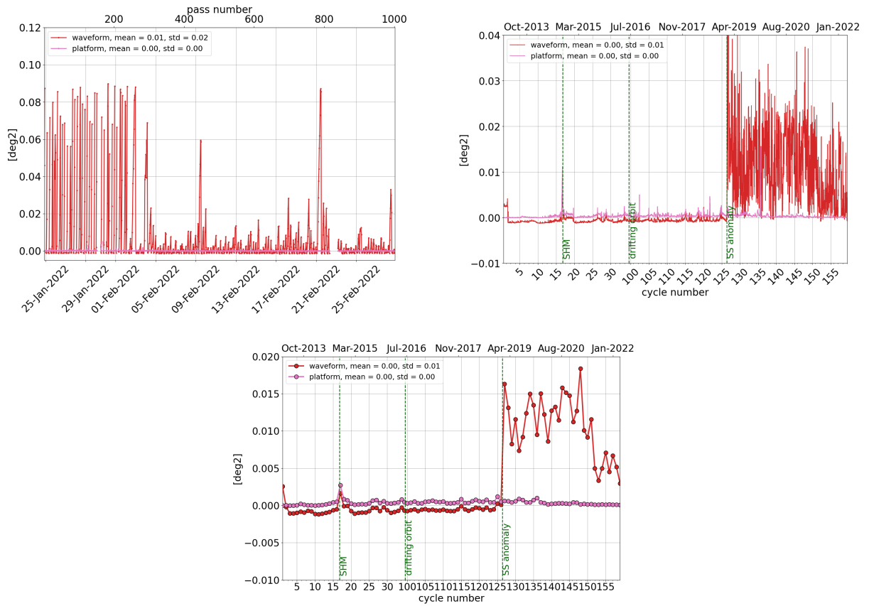
Figure 14: Monitoring per pass for cycle 158 (left), daily monitoring (right) and cyclic monitoring (bottom) of SARAL/AltiKa's mispointing angle: comparison between the one derived from waveform retracking and the one measured by platform startrackers.
