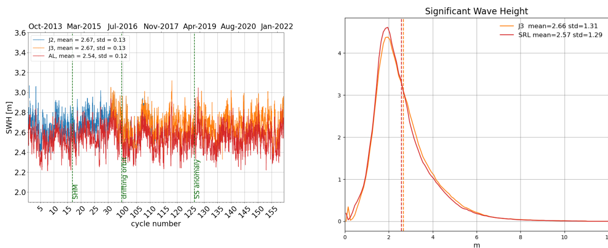
Figure 7: Daily monitoring of significant wave height for AltiKa (Ka-band) Jason-2 and Jason-3 (Ku-band) on the left and histogram for cycle 158 on the right (limited to 66^\circ latitude).
