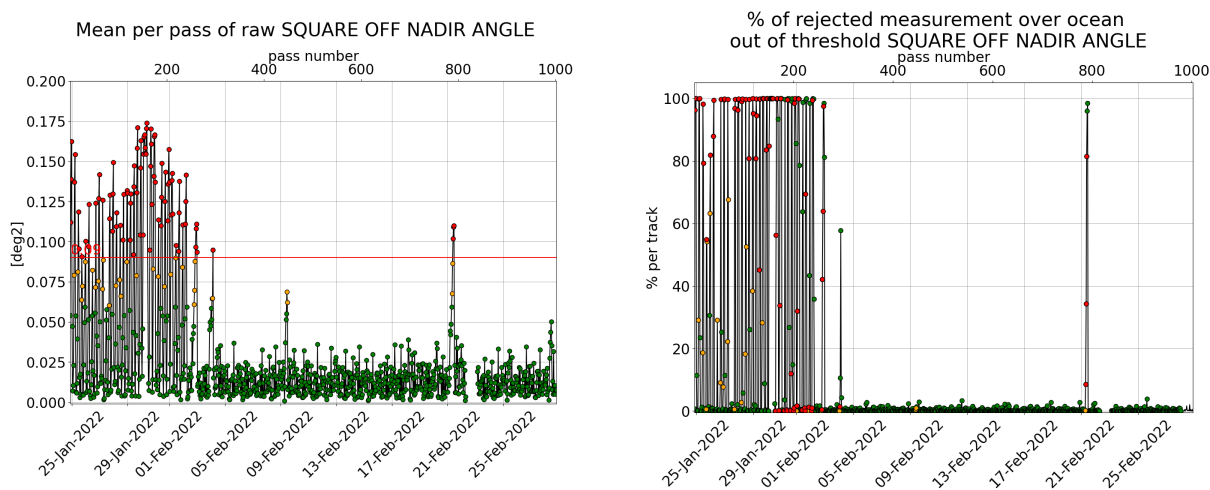
Figure 3: [left] Mispointing cycle 158, [right] Percentage of rejected measurement by threshold on square off-nadir angle.
