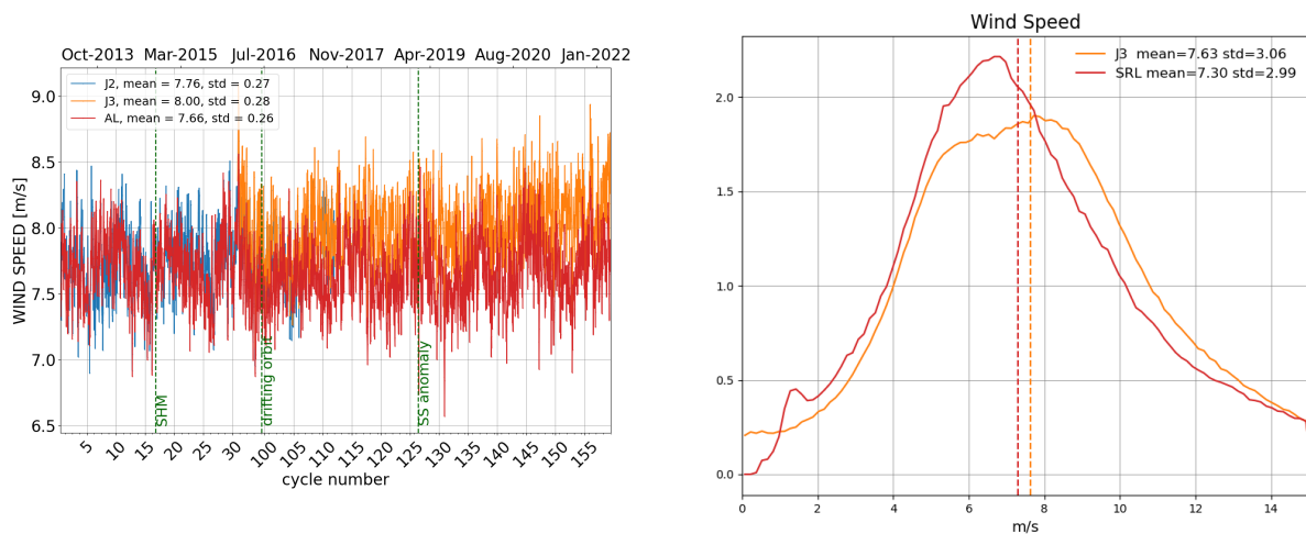
Figure 11: Daily monitoring of altimeter wind speed for Saral/AltiKa, Jason-2 and Jason-3 on the left and histogram for cycle 158 on the right (limited to 66° latitude).
