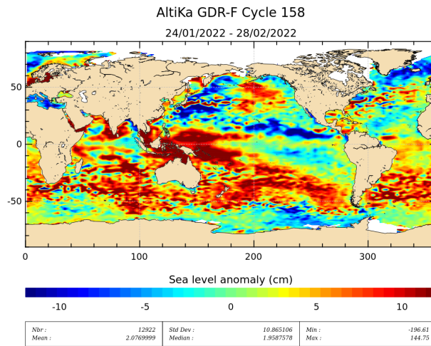
Figure 20: Sea level anomaly relative to MSS for cycle 158.
