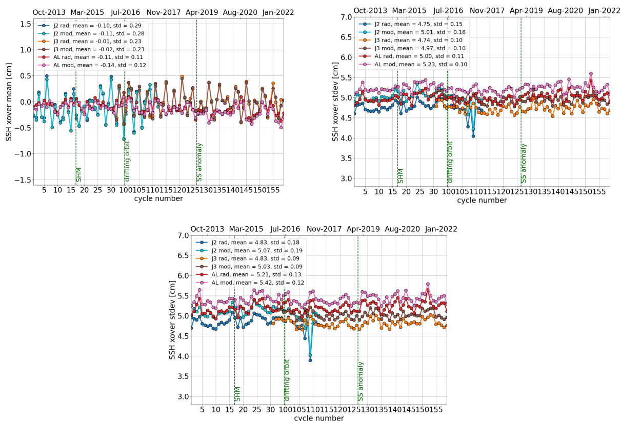
Figure 16: Cyclic monitoring of mean (left) and standard deviation of SSH differences at crossovers using only the geographical selection criteria (right) and both geographical selection and latitude weighting (bottom).
