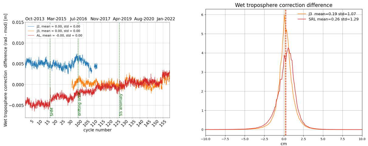
Figure 13: Daily monitoring of wet troposphere differences (Radiometer-ECMWF model) for Saral/AltiKa Jason-2 and Jason-3 (left) and histogram on the right (limited to 66° latitude) for cycle 158 .
