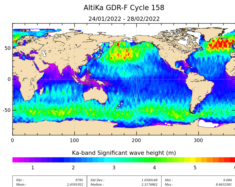
Figure 6: Significant wave height for cycle 158.
