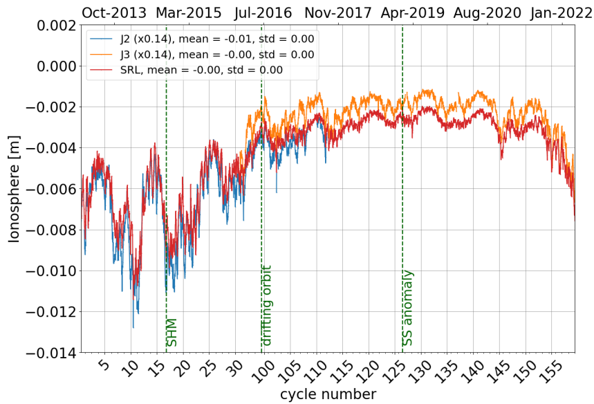
Figure 9: Daily monitoring of dual-frequency ionosphere correction for Jason-2 Jason-3 and GIM ionosphere correction for Saral/AltiKa.
