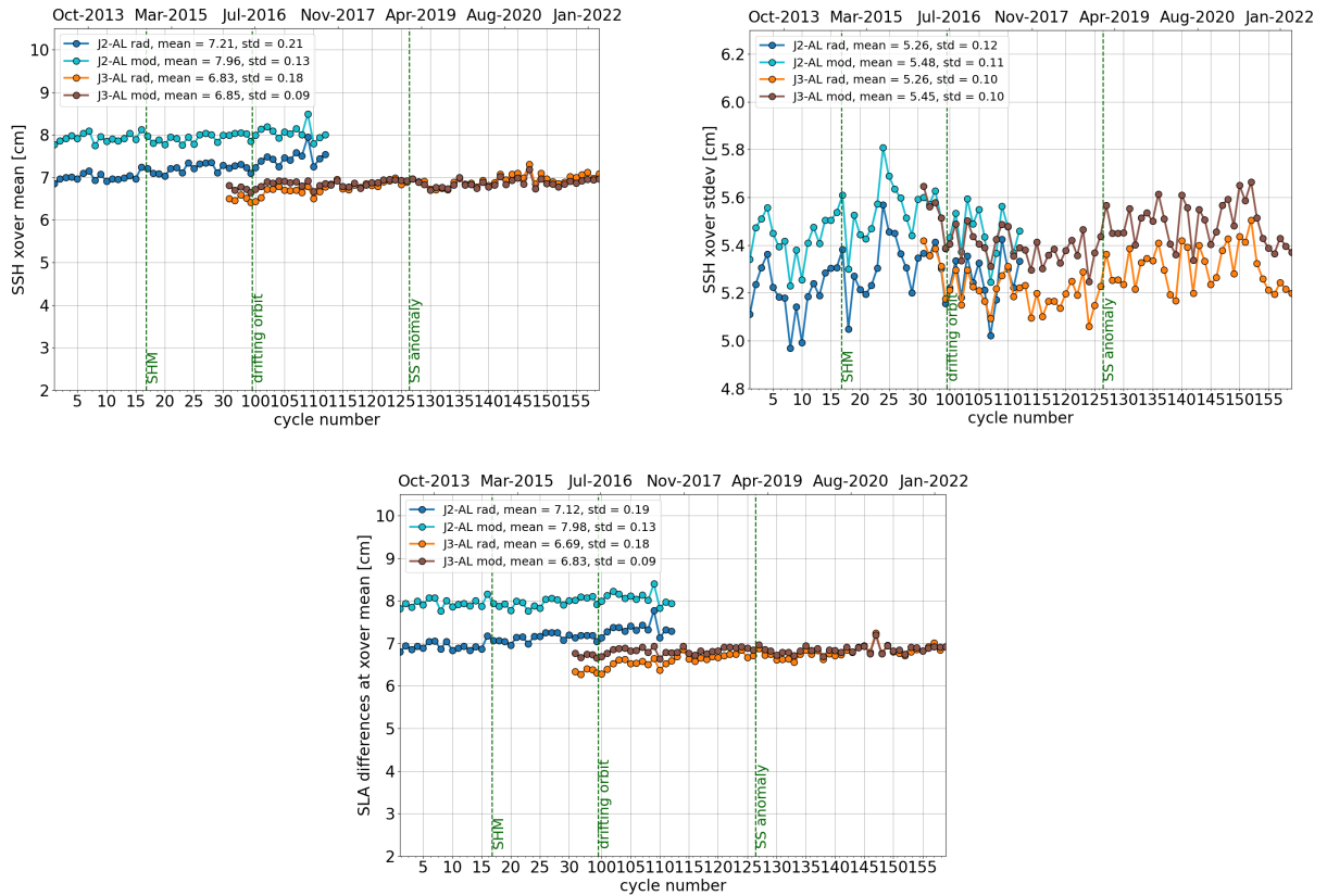
Figure 17: Cyclic monitoring of mean (left) and standard deviation (right) of Jason-2 / AltiKa & Jason-3 / AltiKa SSH differences at crossovers using geographical selections. Box-averaged SLA differences at crossovers (bottom).
