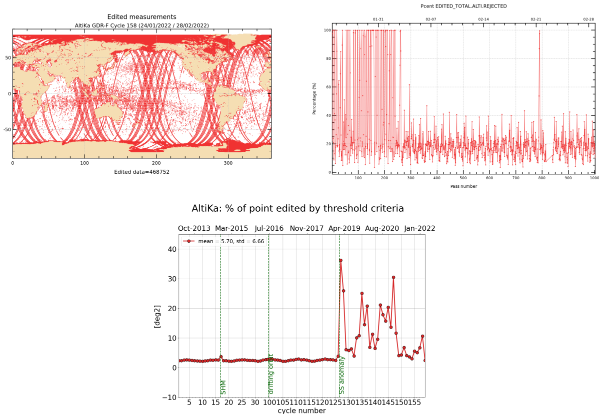
Figure 2: Rejected measurements on thresholds criteria : Cycle 158, map and monitoring of % of rejected measurements per track (top), whole time serie / % of rejected measurements per cycle (bottom).
