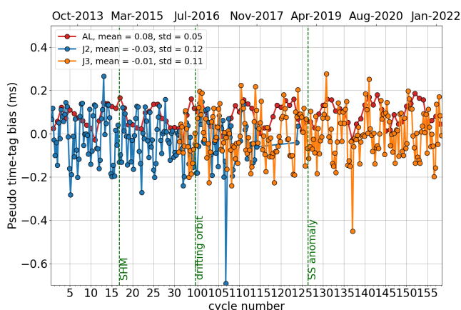
Figure 18: Cyclic monitoring of pseudo time tag bias for Saral/AltiKa.
