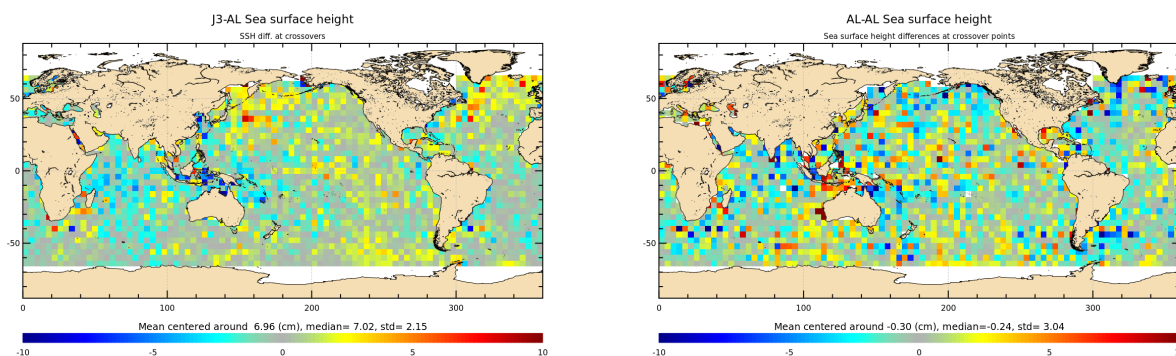
Figure 15: Mean of multi-mission SSH and mono-mission SSH differences at crossovers for cycle 158.
