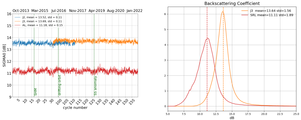
Figure 8: Daily monitoring of backscattering coefficient for Saral/AltiKa, Jason-2 and Jason-3 on the left and histogram for cycle 158 on the right (limited to 66° latitude).
