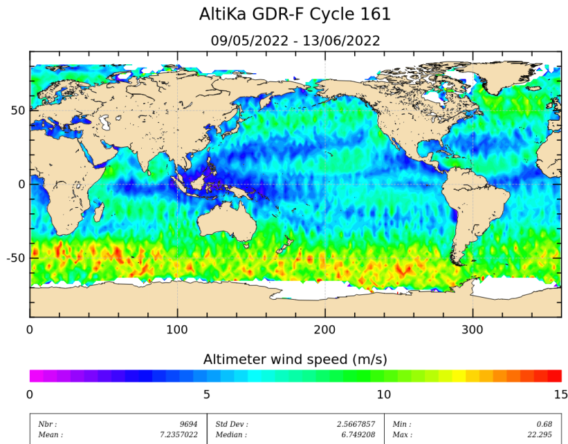
Figure 9: Altimeter wind speed for cycle 161.
