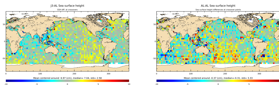
Figure 14: Mean of multi-mission SSH and mono-mission SSH differences at crossovers for cycle 161.
