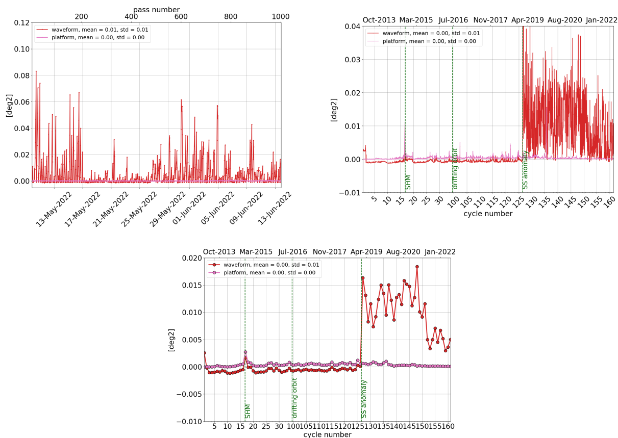
Figure 13: Monitoring per pass for cycle 161 (left), daily monitoring(right) and cyclic monitoring (bottom) of SARAL/AltiKa's mispointing angle: comparison between the one derived from waveform retracking and the one measured by platform startrackers.
