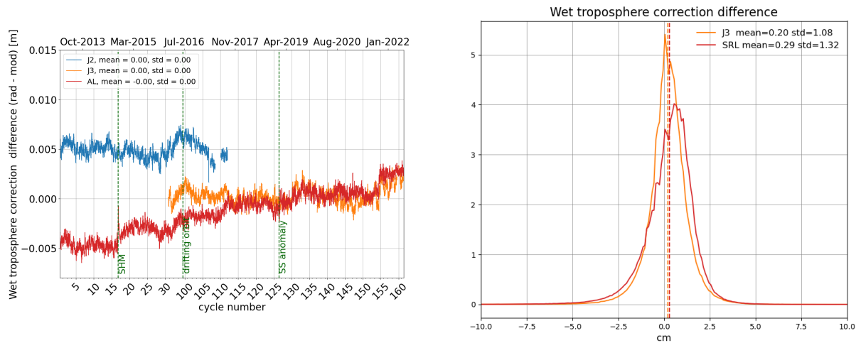
Figure 12: Daily monitoring of wet troposphere differences (Radiometer-ECMWF model) for Saral/AltiKa Jason-2 and Jason-3 (left) and histogram on the right (limited to 66° latitude) for cycle 161 .
