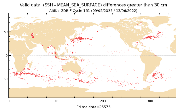
Figure 20: SLA higher than 30 cm for cycle 161.
