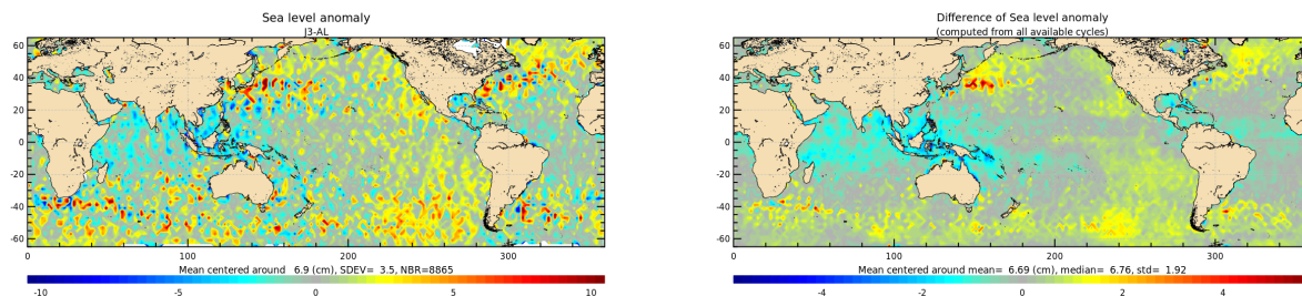
Figure 21: Jason-3 – Saral/AltiKa SLA differences for cycle 161 (left) and averaged over the whole Saral/AltiKa period (right).
