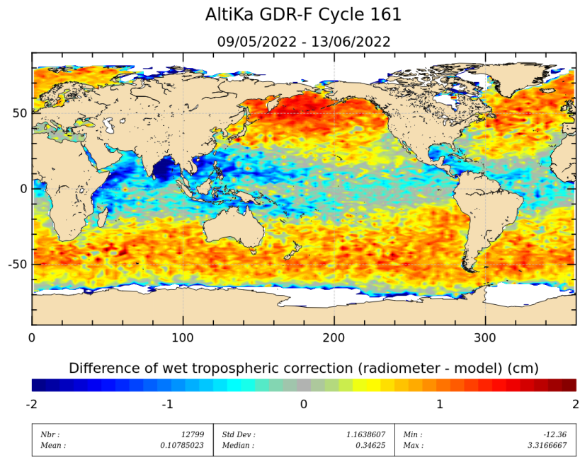
Figure 11: Mean of wet troposphere correction difference (Radiometer-ECMWF model) for cycle 161.
