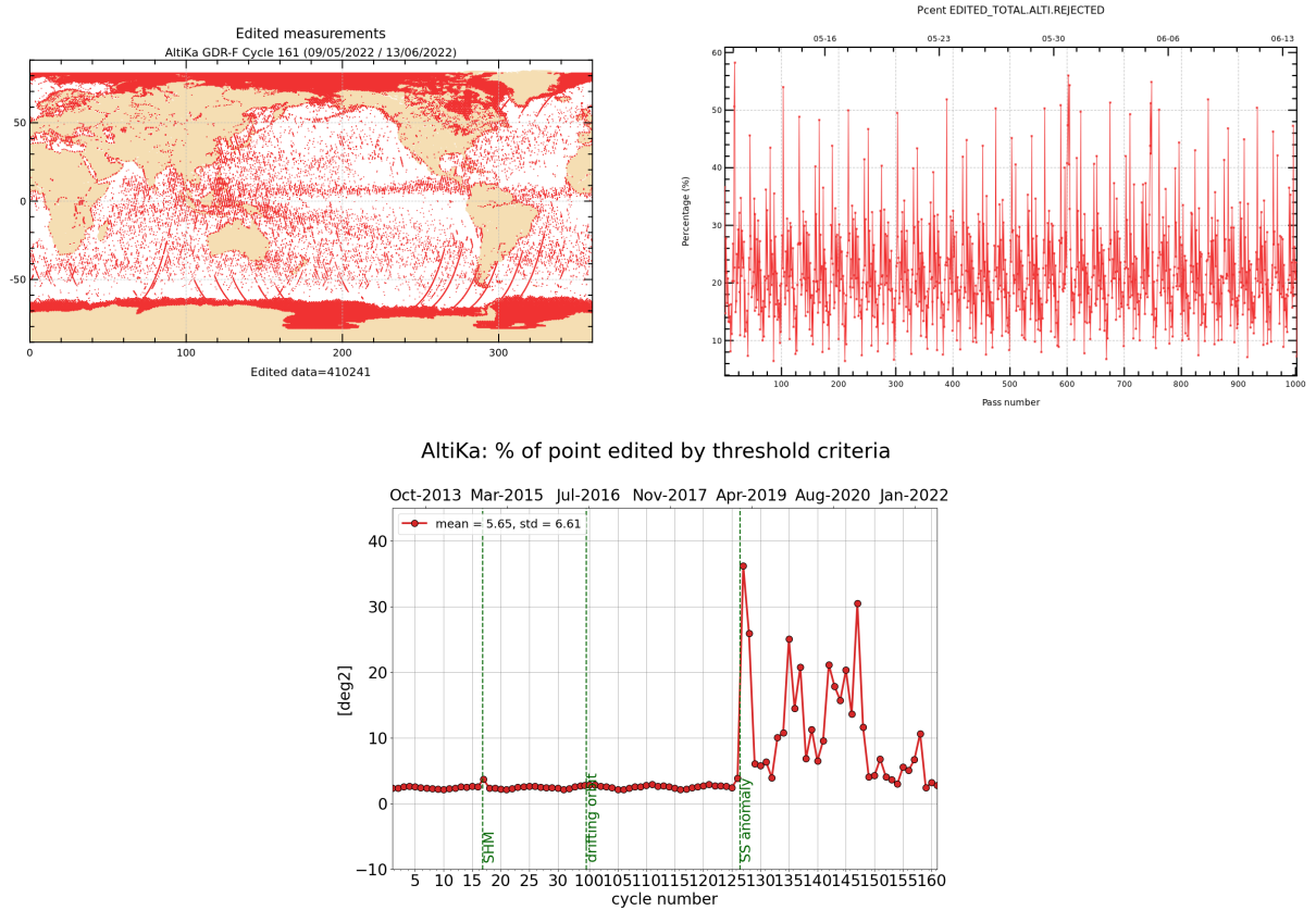
Figure 2: Rejected measurements on thresholds criteria : Cycle 161, map and monitoring of % of rejected measurements per track (top), whole time serie / % of rejected measurements per cycle (bottom).
