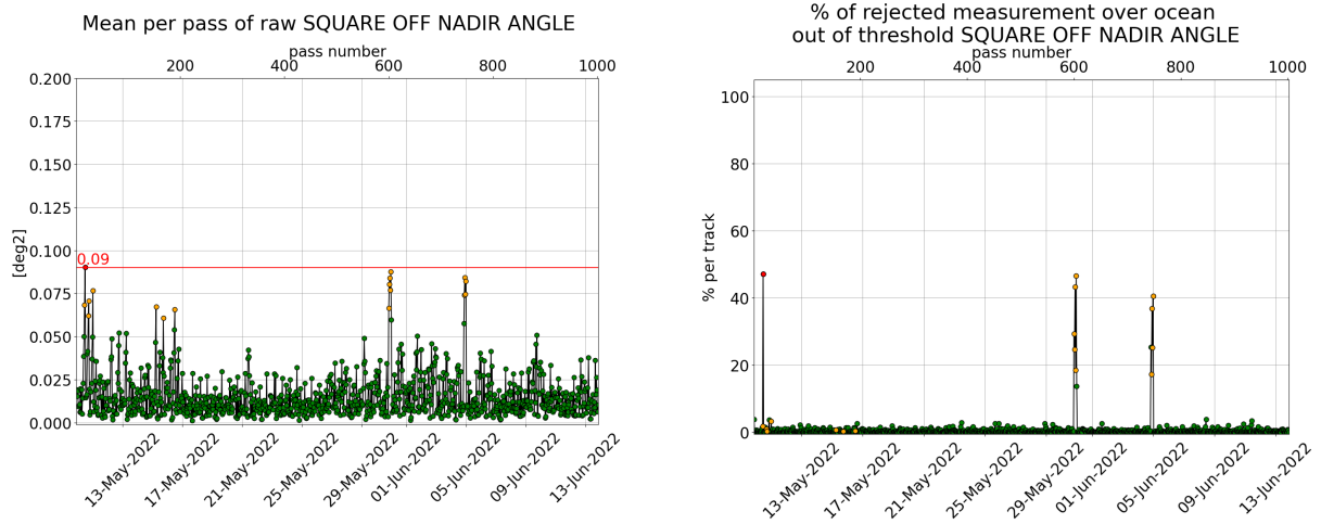
Figure 3: [left] Mispointing cycle 161, [right] Percentage of rejected measurement by threshold on square off-nadir angle.
