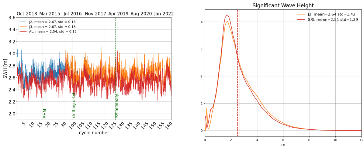
Figure 6: Daily monitoring of significant wave height for AltiKa (Ka-band) Jason-2 and Jason-3 (Ku-band) on the left and histogram for cycle 161 on the right (limited to 66^\circ latitude).
