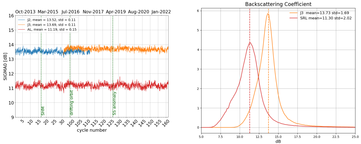
Figure 7: Daily monitoring of backscattering coefficient for Saral/AltiKa, Jason-2 and Jason-3 on the left and histogram for cycle 161 on the right (limited to 66° latitude).
