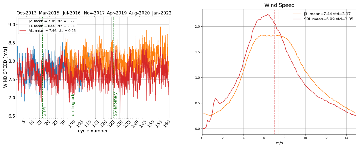
Figure 10: Daily monitoring of altimeter wind speed for Saral/AltiKa, Jason-2 and Jason-3 on the left and histogram for cycle 161 on the right (limited to 66° latitude).
