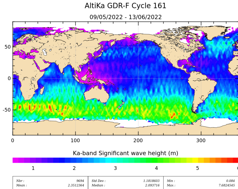
Figure 5: Significant wave height for cycle 161.
