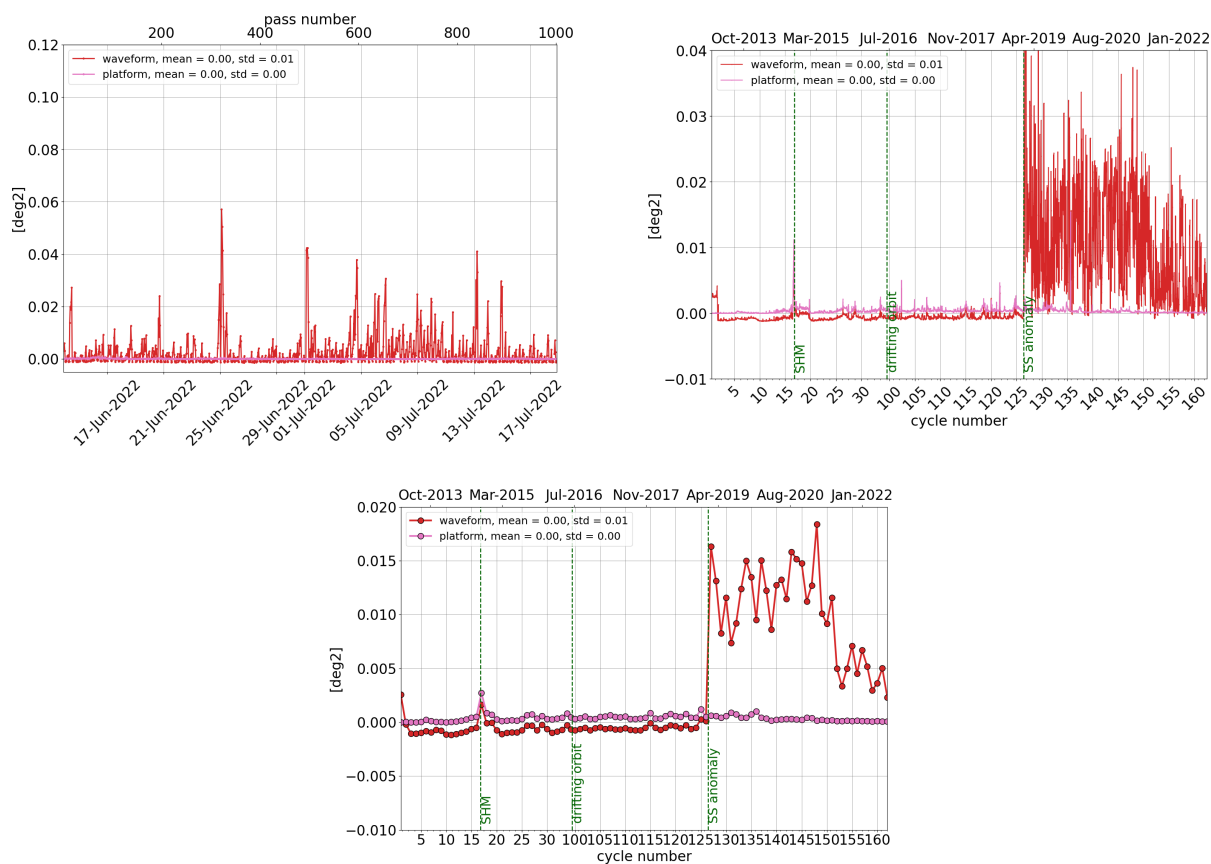
Figure 14: Monitoring per pass for cycle 162 (left), daily monitoring(right) and cyclic monitoring (bottom) of SARAL/AltiKa's mispointing angle: comparison between the one derived from waveform retracking and the one measured by platform startrackers.
