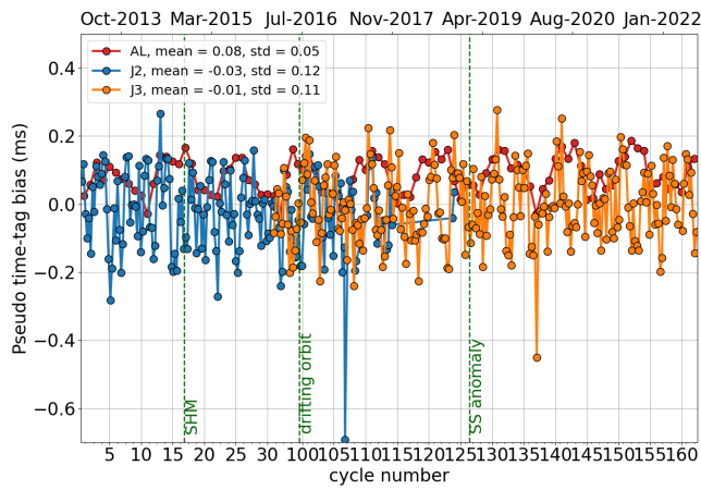
Figure 18: Cyclic monitoring of pseudo time tag bias for Saral/AltiKa.
