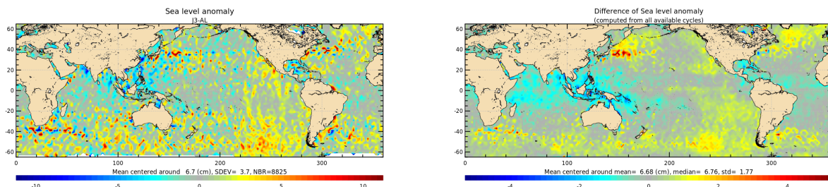
Figure 22: Jason-3 – Saral/AltiKa SLA differences for cycle 162 (left) and averaged over the whole Saral/AltiKa period (right).
