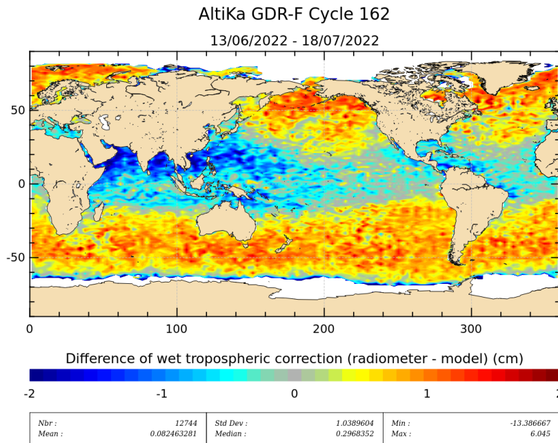
Figure 12: Mean of wet troposphere correction difference (Radiometer-ECMWF model) for cycle 162.
