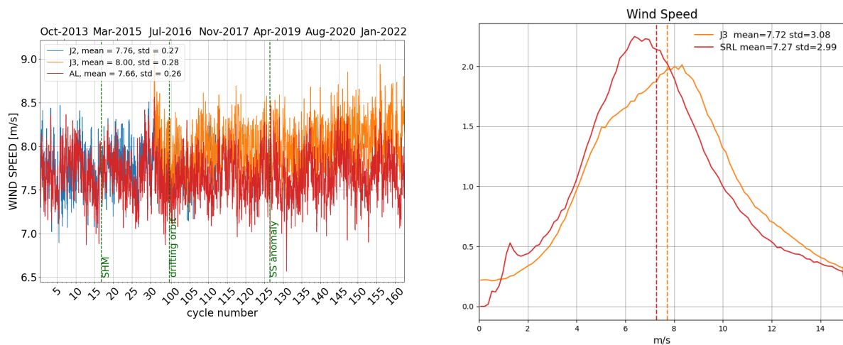
Figure 11: Daily monitoring of altimeter wind speed for Saral/AltiKa, Jason-2 and Jason-3 on the left and histogram for cycle 162 on the right (limited to 66° latitude).
