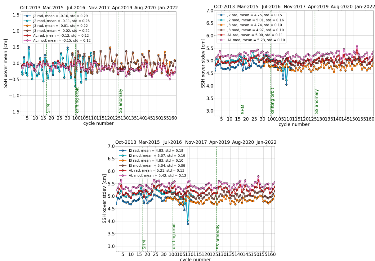
Figure 16: Cyclic monitoring of mean (left) and standard deviation of SSH differences at crossovers using only the geographical selection criteria (right) and both geographical selection and latitude weighting (bottom).
