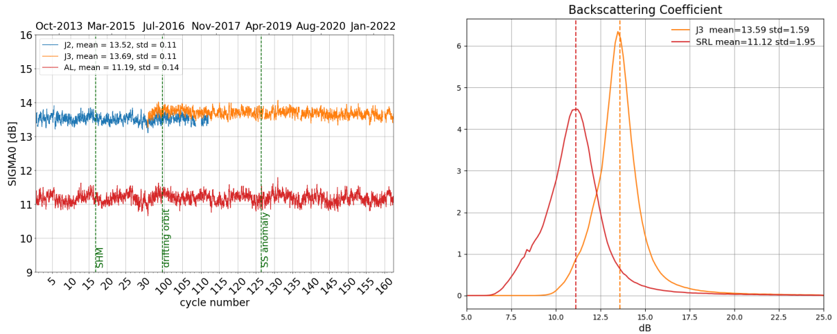
Figure 8: Daily monitoring of backscattering coefficient for Saral/AltiKa, Jason-2 and Jason-3 on the left and histogram for cycle 162 on the right (limited to 66° latitude).
