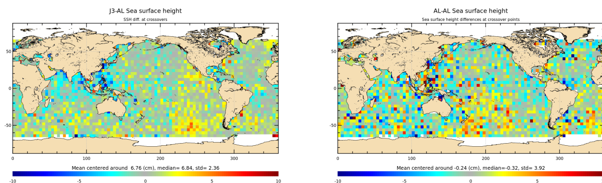
Figure 15: Mean of multi-mission SSH and mono-mission SSH differences at crossovers for cycle 162.
