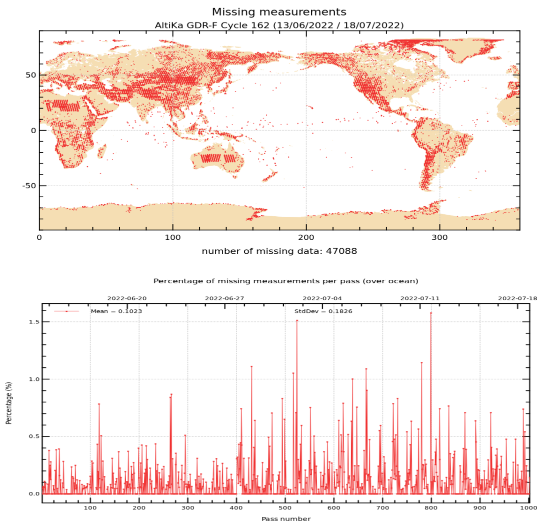
Figure 1: Map of missing measurements for cycle 162 on top. Monitoring of percentage of missing ocean measurements per pass on bottom.
