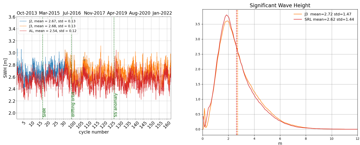
Figure 7: Daily monitoring of significant wave height for AltiKa (Ka-band) Jason-2 and Jason-3 (Ku-band) on the left and histogram for cycle 162 on the right (limited to 66° latitude).
