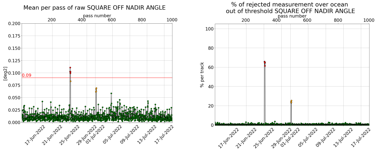
Figure 3: [left] Mispointing cycle 162, [right] Percentage of rejected measurement by threshold on square off-nadir angle.
