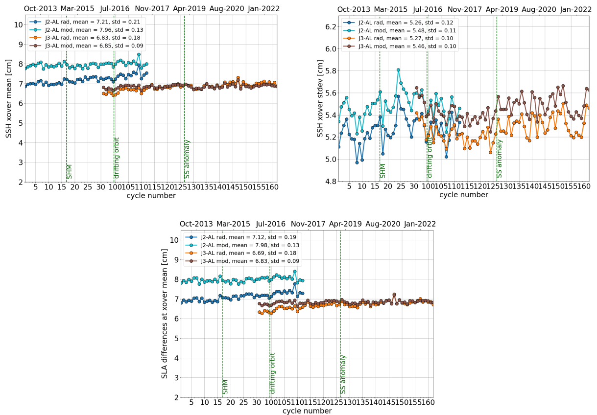
Figure 17: Cyclic monitoring of mean (left) and standard deviation (right) of Jason-2 / AltiKa & Jason-3 / AltiKa SSH differences at crossovers using geographical selections. Box-averaged SLA differences at crossovers (bottom).
