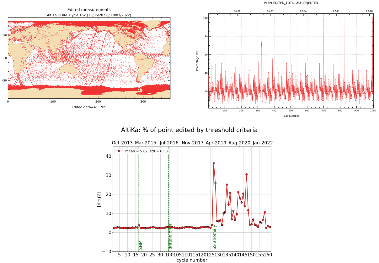
Figure 2: Rejected measurements on thresholds criteria : Cycle 162, map and monitoring of % of rejected measurements per track (top), whole time serie / % of rejected measurements per cycle (bottom).
