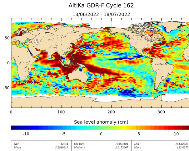
Figure 20: Sea level anomaly relative to MSS for cycle 162.
