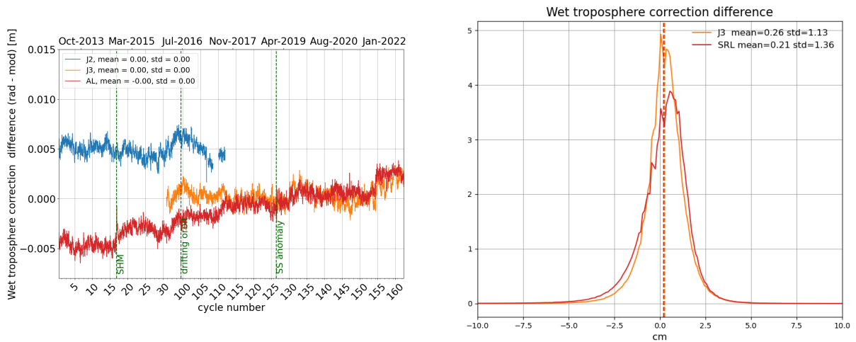
Figure 13: Daily monitoring of wet troposphere differences (Radiometer-ECMWF model) for Saral/AltiKa Jason-2 and Jason-3 (left) and histogram on the right (limited to 66° latitude) for cycle 162 .
