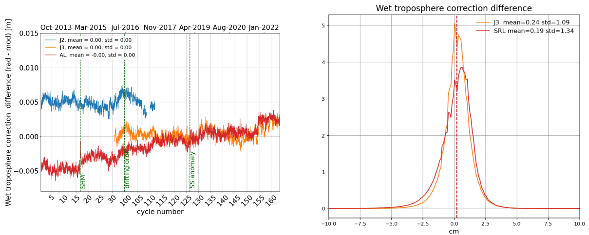
Figure 12: Daily monitoring of wet troposphere differences (Radiometer-ECMWF model) for Saral/AltiKa Jason-2 and Jason-3 (left) and histogram on the right (limited to 66° latitude) for cycle 163 .
