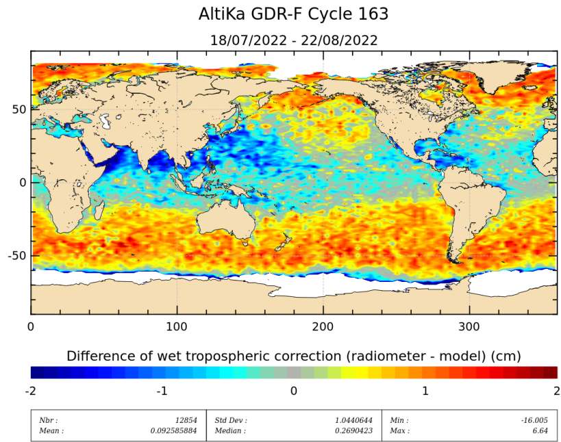
Figure 11: Mean of wet troposphere correction difference (Radiometer-ECMWF model) for cycle 163.
