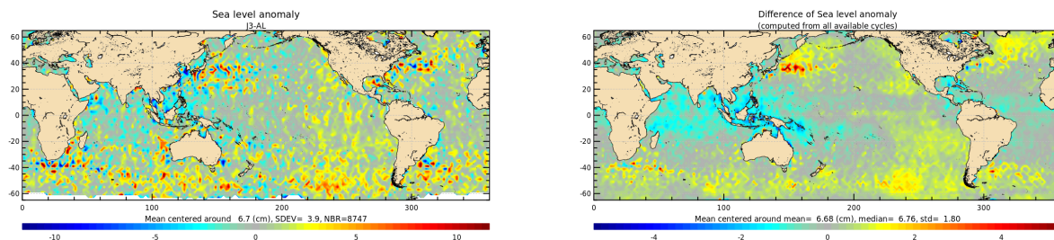
Figure 21: Jason-3 – Saral/AltiKa SLA differences for cycle 163 (left) and averaged over the whole Saral/AltiKa period (right).
