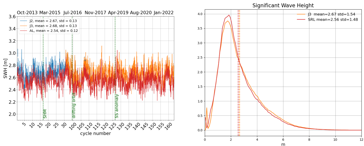
Figure 6: Daily monitoring of significant wave height for AltiKa (Ka-band) Jason-2 and Jason-3 (Ku-band) on the left and histogram for cycle 163 on the right (limited to 66° latitude).
