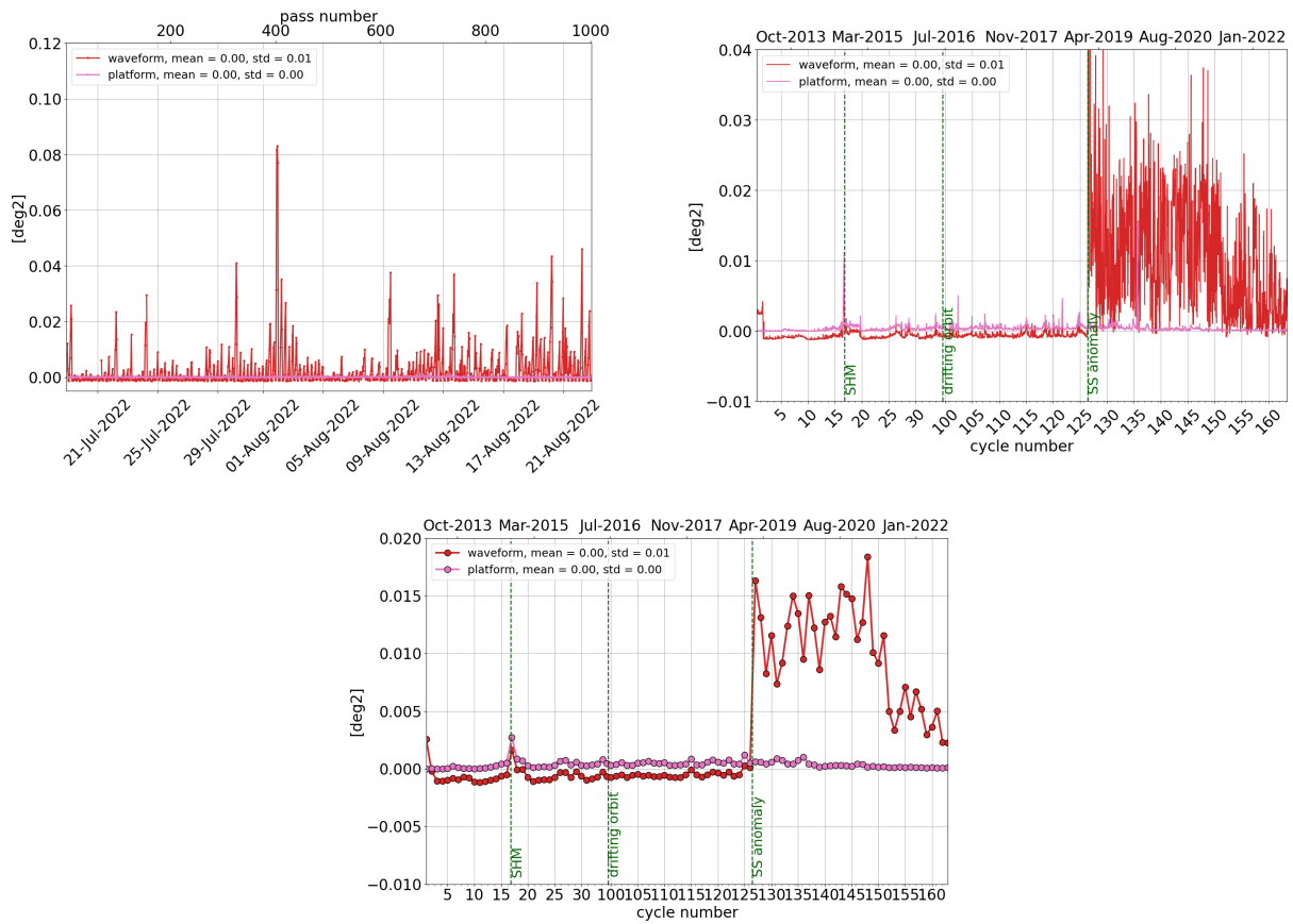
Figure 13: Monitoring per pass for cycle 163 (left), daily monitoring(right) and cyclic monitoring (bottom) of SARAL/AltiKa's mispointing angle: comparison between the one derived from waveform retracking and the one measured by platform startrackers.
