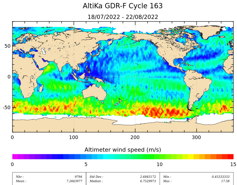
Figure 9: Altimeter wind speed for cycle 163.
