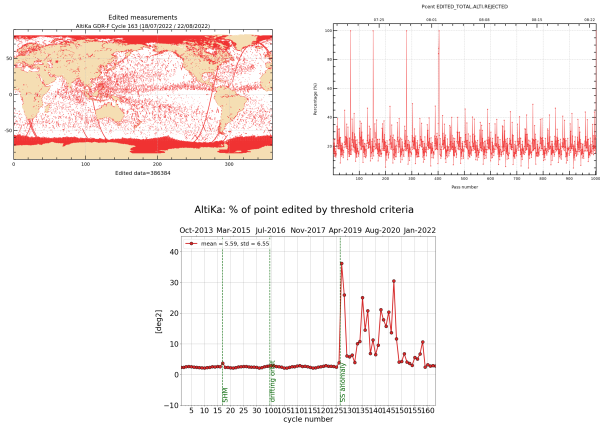
Figure 2: Rejected measurements on thresholds criteria : Cycle 163, map and monitoring of % of rejected measurements per track (top), whole time serie / % of rejected measurements per cycle (bottom).
