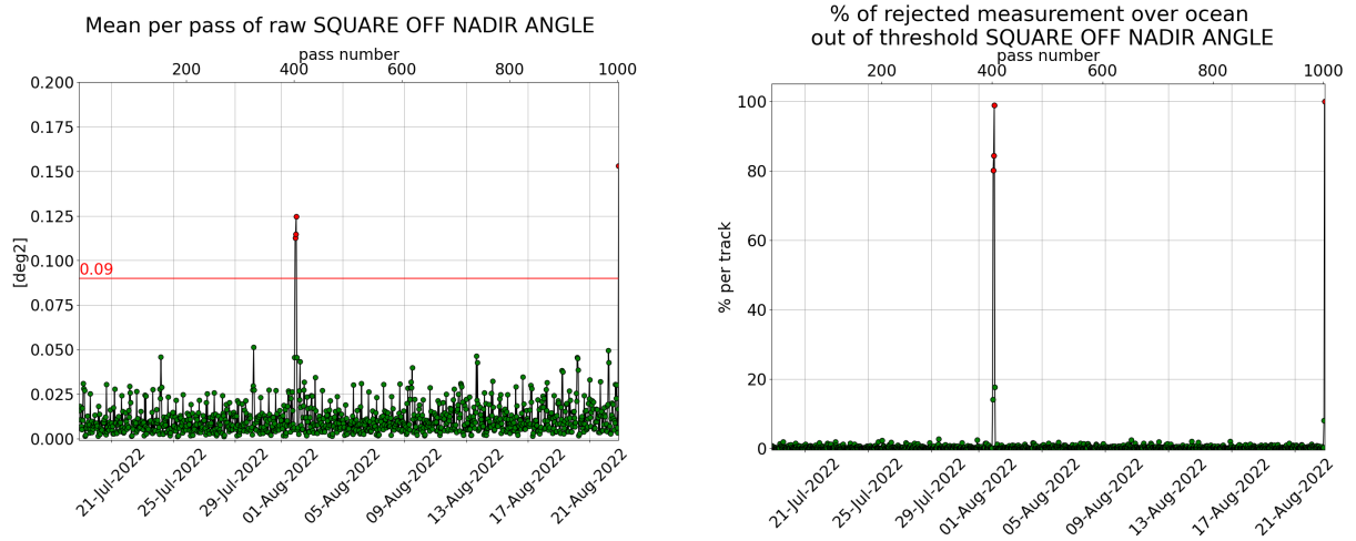
Figure 3: [left] Mispointing cycle 163, [right] Percentage of rejected measurement by threshold on square off-nadir angle.
