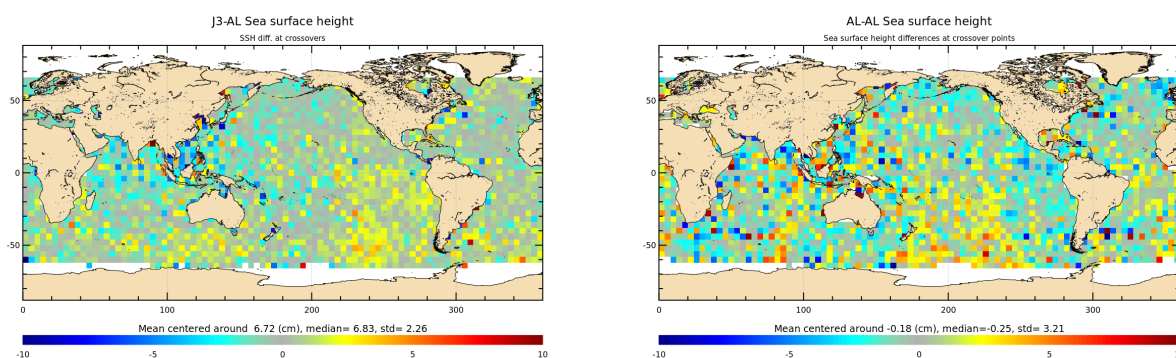
Figure 14: Mean of multi-mission SSH and mono-mission SSH differences at crossovers for cycle 163.
