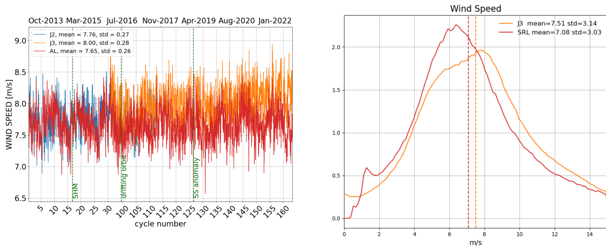
Figure 10: Daily monitoring of altimeter wind speed for Saral/AltiKa, Jason-2 and Jason-3 on the left and histogram for cycle 163 on the right (limited to 66° latitude).
