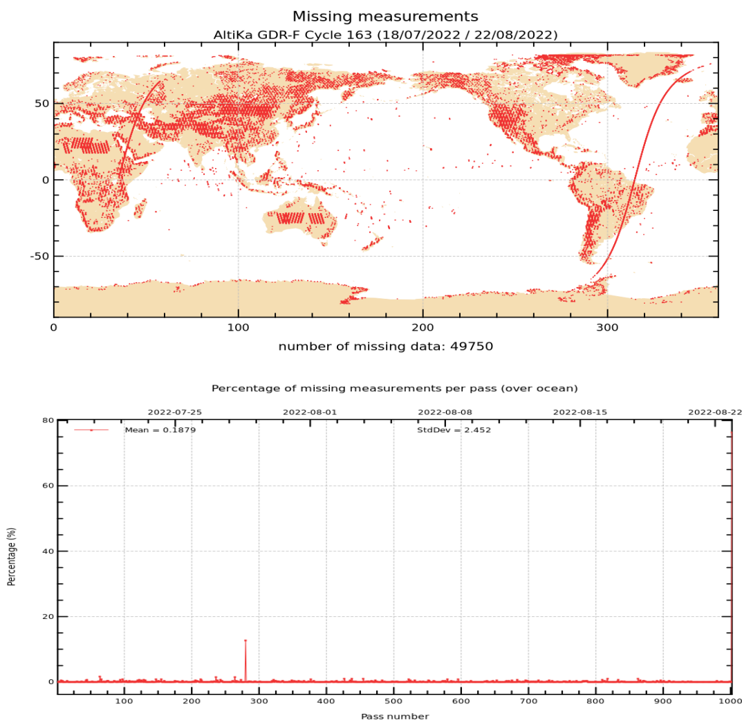
Figure 1: Map of missing measurements for cycle 163 on top. Monitoring of percentage of missing ocean measurements per pass on bottom.
