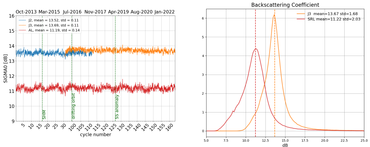
Figure 7: Daily monitoring of backscattering coefficient for Saral/AltiKa, Jason-2 and Jason-3 on the left and histogram for cycle 163 on the right (limited to 66° latitude).
