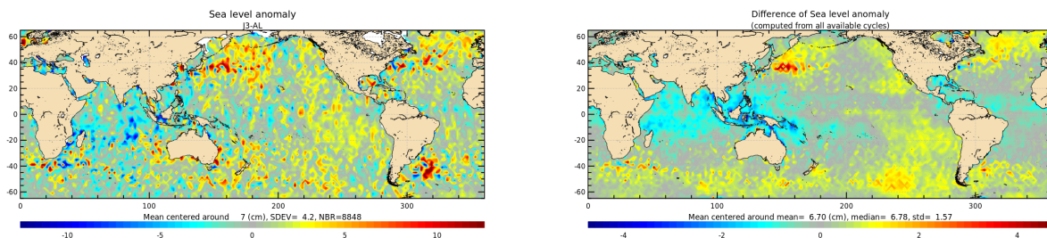
Figure 21: Jason-3 – Saral/AltiKa SLA differences for cycle 168 (left) and averaged over the whole Saral/AltiKa period (right).
