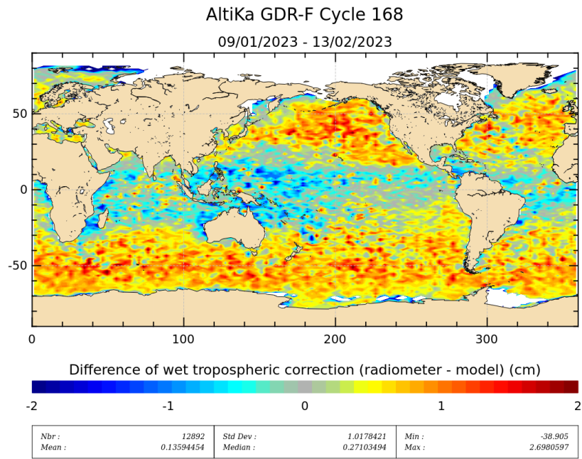
Figure 11: Mean of wet troposphere correction difference (Radiometer-ECMWF model) for cycle 168.
