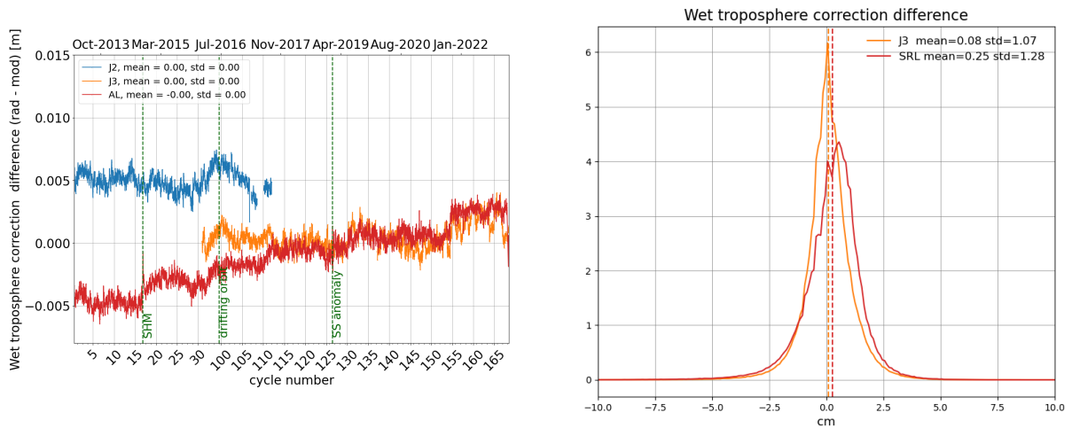
Figure 12: Daily monitoring of wet troposphere differences (Radiometer-ECMWF model) for Saral/AltiKa Jason-2 and Jason-3 (left) and histogram on the right (limited to 66° latitude) for cycle 168 .
