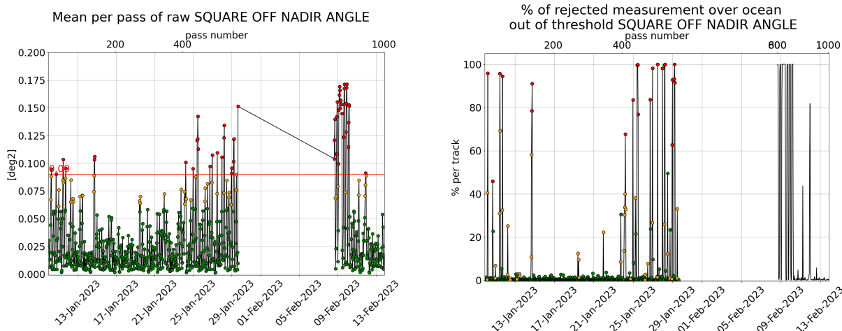
Figure 3: [left] Mispointing cycle 168, [right] Percentage of rejected measurement by threshold on square off-nadir angle.
