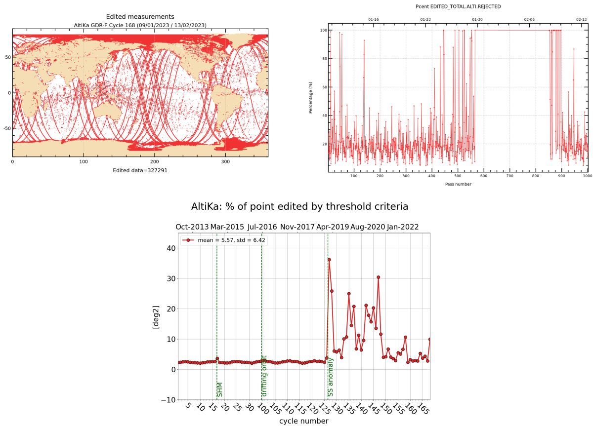
Figure 2: Rejected measurements on thresholds criteria : Cycle 168, map and monitoring of % of rejected measurements per track (top), whole time serie / % of rejected measurements per cycle (bottom).
