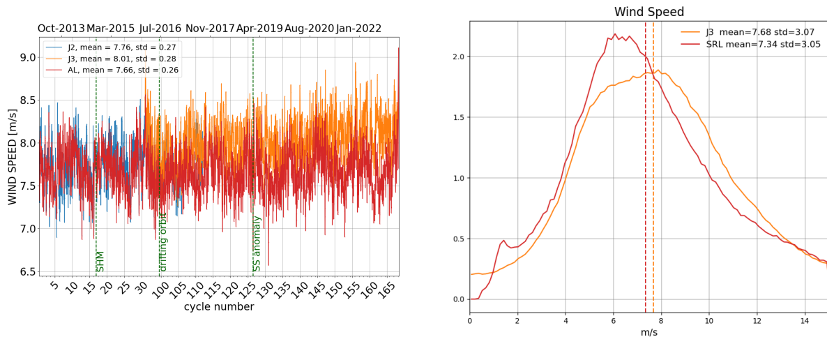
Figure 10: Daily monitoring of altimeter wind speed for Saral/AltiKa, Jason-2 and Jason-3 on the left and histogram for cycle 168 on the right (limited to 66° latitude).
