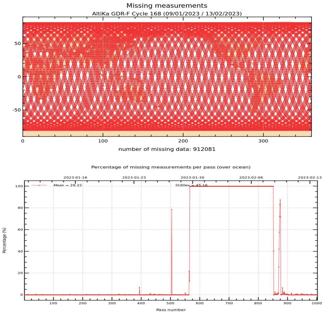
Figure 1: Map of missing measurements for cycle 168 on top. Monitoring of percentage of missing ocean measurements per pass on bottom.
