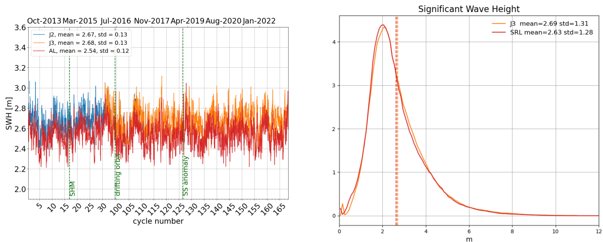
Figure 6: Daily monitoring of significant wave height for AltiKa (Ka-band) Jason-2 and Jason-3 (Ku-band) on the left and histogram for cycle 168 on the right (limited to 66^\circ latitude).
