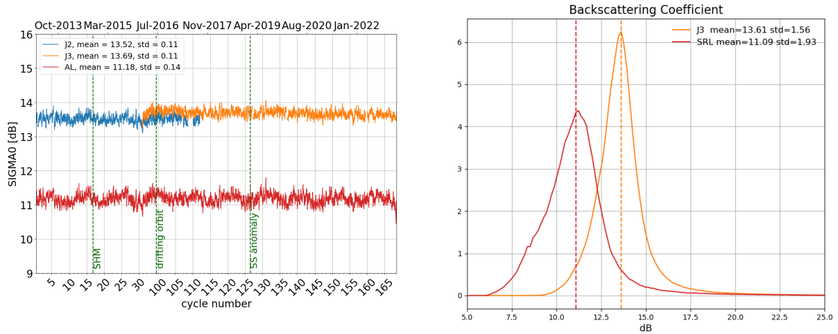
Figure 7: Daily monitoring of backscattering coefficient for Saral/AltiKa, Jason-2 and Jason-3 on the left and histogram for cycle 168 on the right (limited to 66° latitude).
