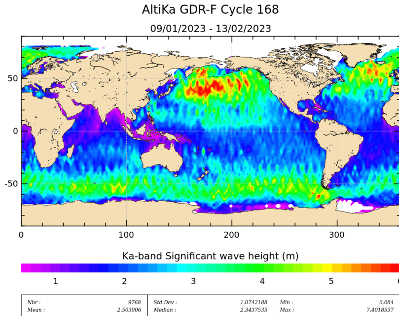
Figure 5: Significant wave height for cycle 168.
