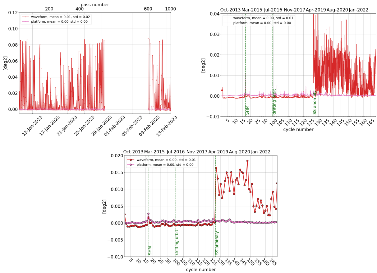
Figure 13: Monitoring per pass for cycle 168 (left), daily monitoring(right) and cyclic monitoring (bottom) of SARAL/AltiKa's mispointing angle: comparison between the one derived from waveform retracking and the one measured by platform startrackers.
