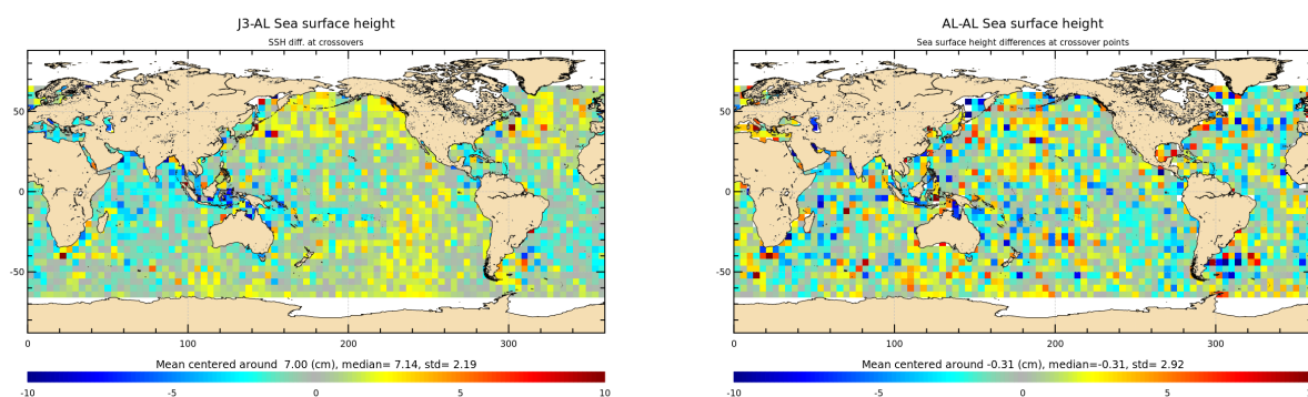
Figure 14: Mean of multi-mission SSH and mono-mission SSH differences at crossovers for cycle 169.
