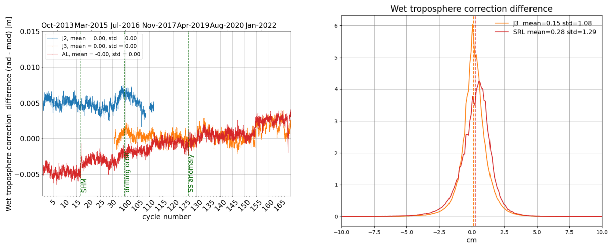
Figure 12: Daily monitoring of wet troposphere differences (Radiometer-ECMWF model) for Saral/AltiKa Jason-2 and Jason-3 (left) and histogram on the right (limited to 66° latitude) for cycle 169 .
