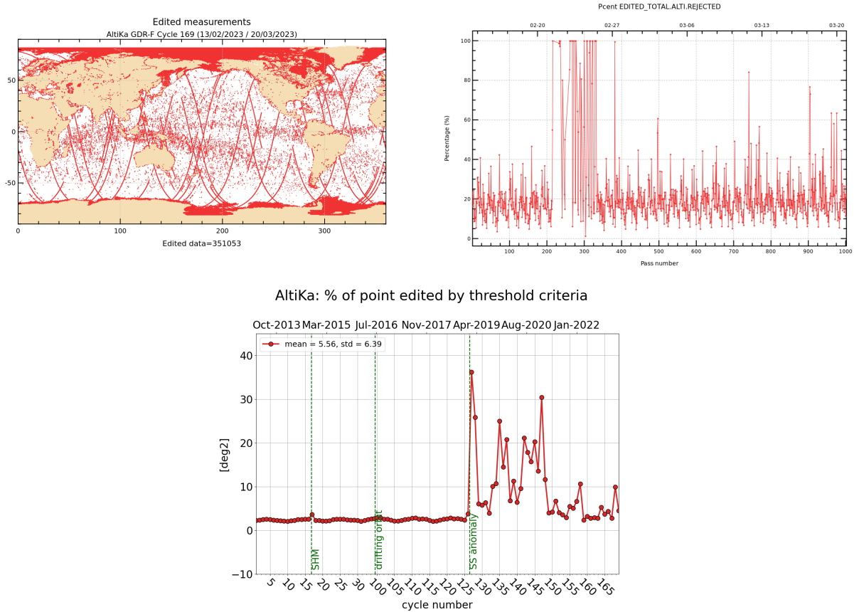
Figure 2: Rejected measurements on thresholds criteria : Cycle 169, map and monitoring of % of rejected measurements per track (top), whole time serie / % of rejected measurements per cycle (bottom).
