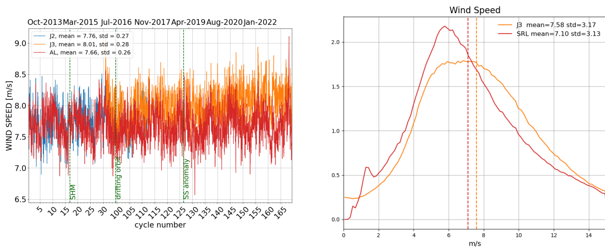
Figure 10: Daily monitoring of altimeter wind speed for Saral/AltiKa, Jason-2 and Jason-3 on the left and histogram for cycle 169 on the right (limited to 66° latitude).
