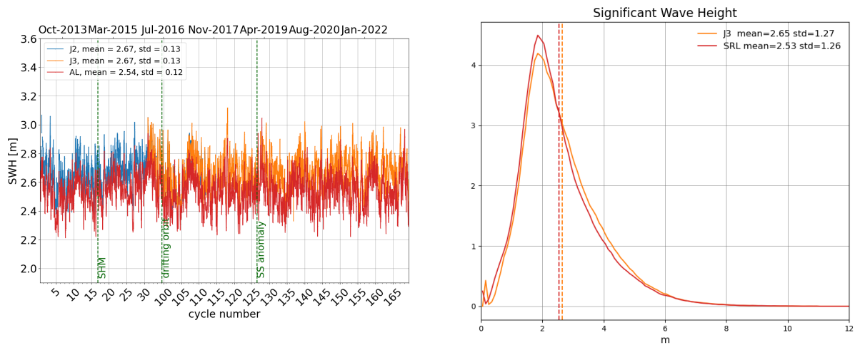
Figure 6: Daily monitoring of significant wave height for AltiKa (Ka-band) Jason-2 and Jason-3 (Ku-band) on the left and histogram for cycle 169 on the right (limited to 66^\circ latitude).
