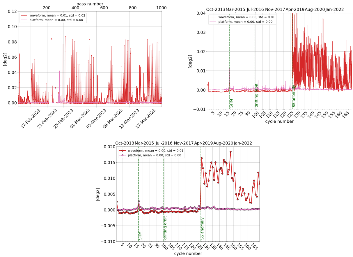
Figure 13: Monitoring per pass for cycle 169 (left), daily monitoring (right) and cyclic monitoring (bottom) of SARAL/AltiKa's mispointing angle: comparison between the one derived from waveform retracking and the one measured by platform startrackers.
