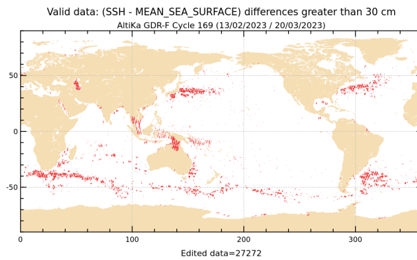
Figure 20: SLA higher than 30 cm for cycle 169.
