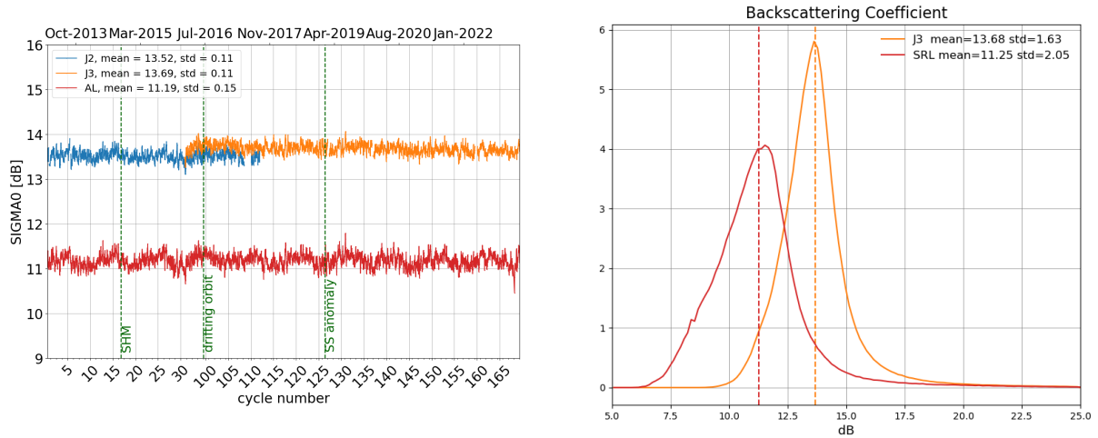
Figure 7: Daily monitoring of backscattering coefficient for Saral/AltiKa, Jason-2 and Jason-3 on the left and histogram for cycle 169 on the right (limited to 66° latitude).
