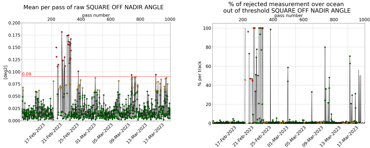
Figure 3: [left] Mispointing cycle 169, [right] Percentage of rejected measurement by threshold on square off-nadir angle.
