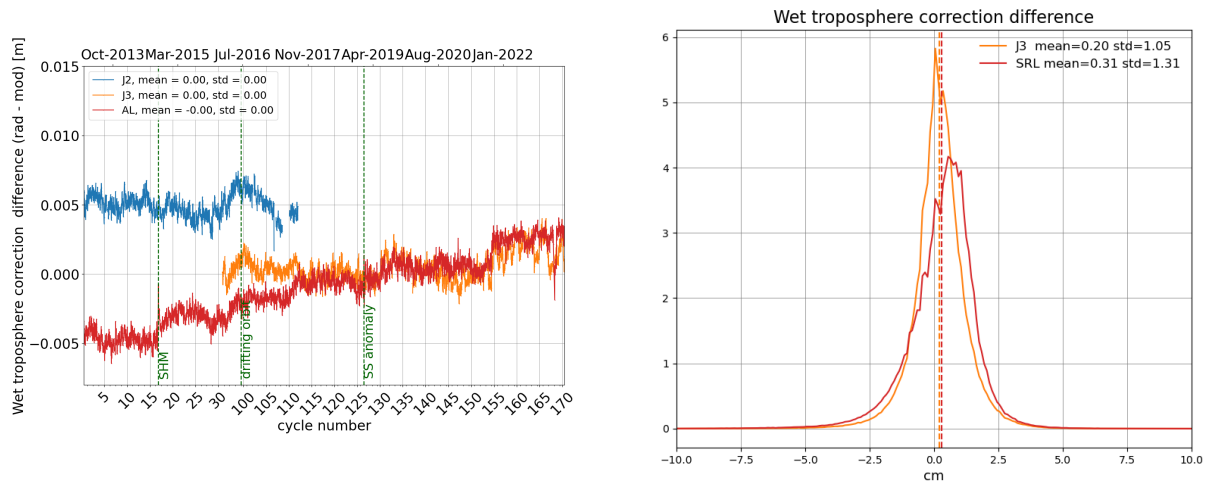
Figure 12: Daily monitoring of wet troposphere differences (Radiometer-ECMWF model) for Saral/AltiKa Jason-2 and Jason-3 (left) and histogram on the right (limited to 66° latitude) for cycle 170 .
