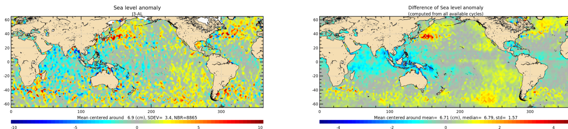
Figure 21: Jason-3 – Saral/AltiKa SLA differences for cycle 170 (left) and averaged over the whole Saral/AltiKa period (right).
