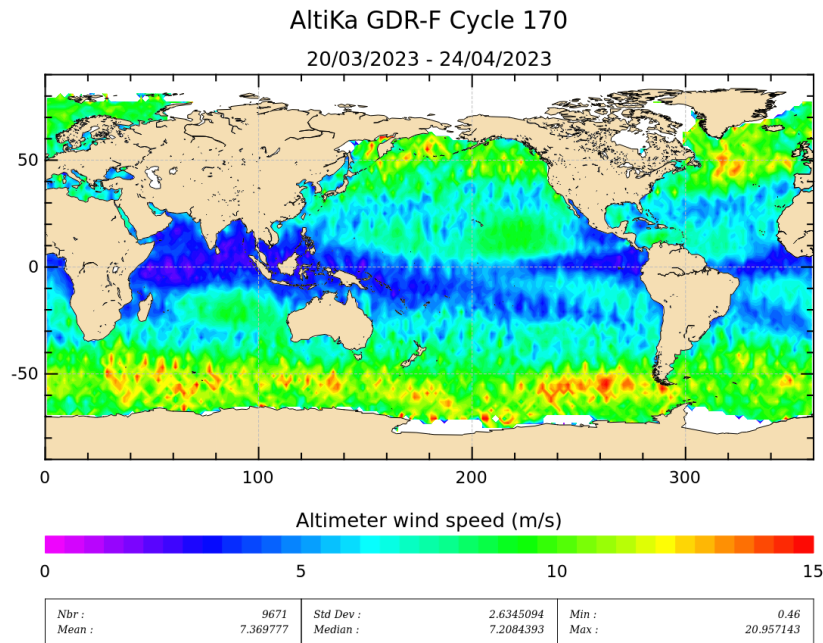
Figure 9: Altimeter wind speed for cycle 170.
