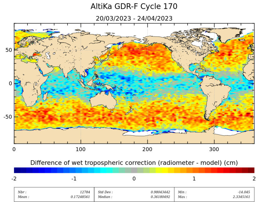
Figure 11: Mean of wet troposphere correction difference (Radiometer-ECMWF model) for cycle 170.
