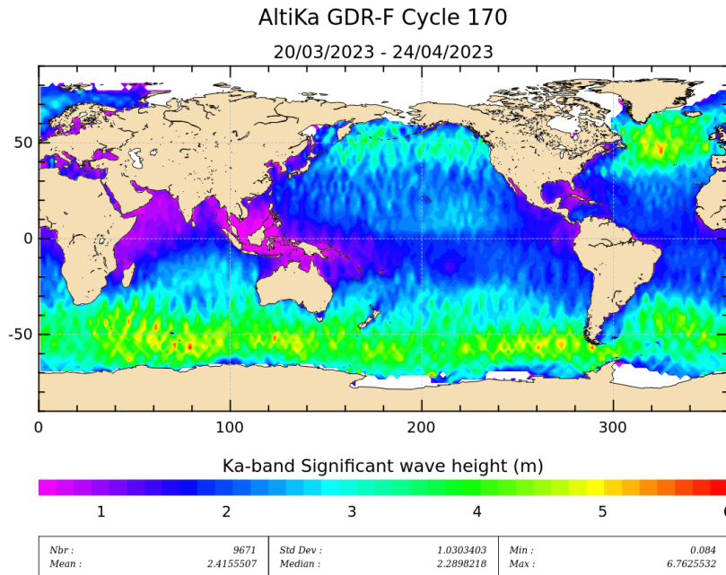
Figure 5: Significant wave height for cycle 170.
