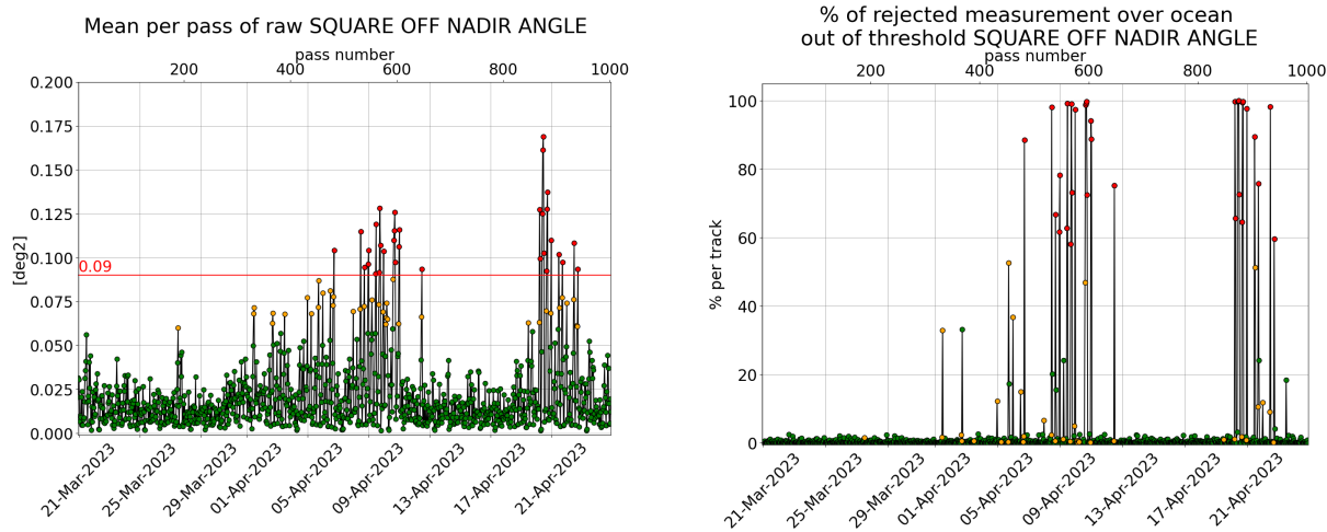
Figure 3: [left] Mispointing cycle 170, [right] Percentage of rejected measurement by threshold on square off-nadir angle.
