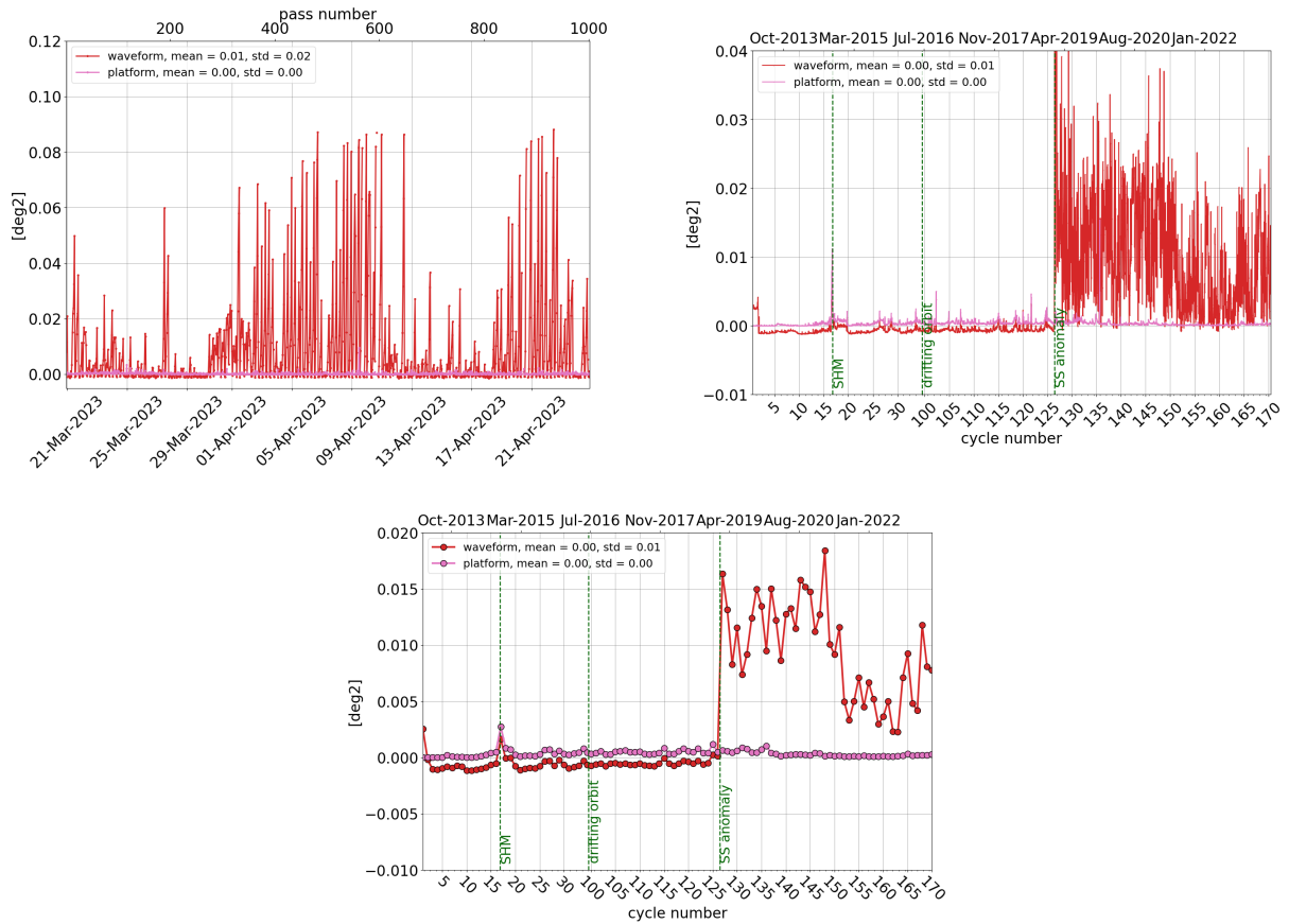
Figure 13: Monitoring per pass for cycle 170 (left), daily monitoring(right) and cyclic monitoring (bottom) of SARAL/AltiKa's mispointing angle: comparison between the one derived from waveform retracking and the one measured by platform startrackers.
