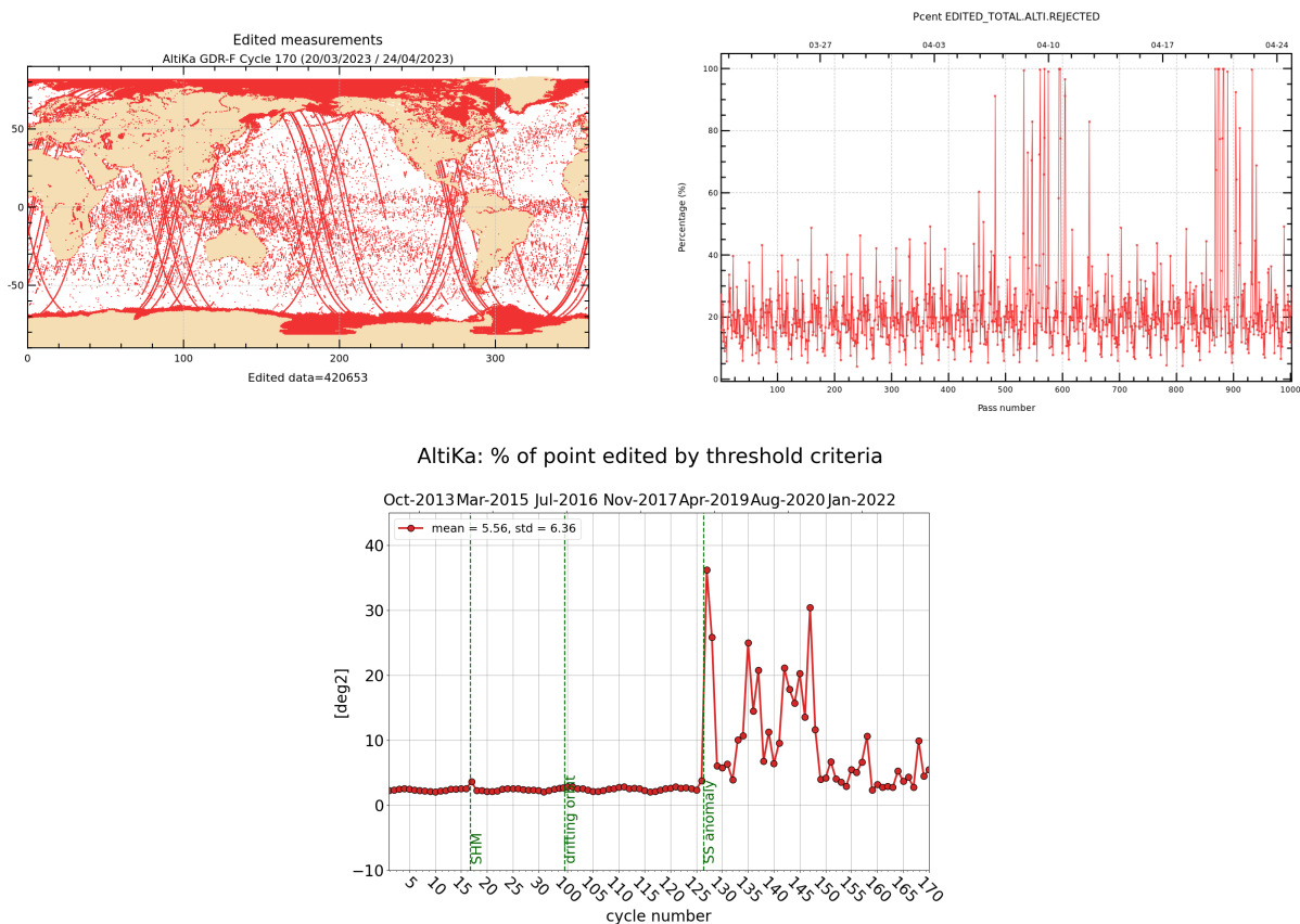
Figure 2: Rejected measurements on thresholds criteria : Cycle 170, map and monitoring of % of rejected measurements per track (top), whole time serie / % of rejected measurements per cycle (bottom).
