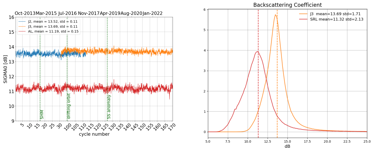
Figure 7: Daily monitoring of backscattering coefficient for Saral/AltiKa, Jason-2 and Jason-3 on the left and histogram for cycle 170 on the right (limited to 66° latitude).
