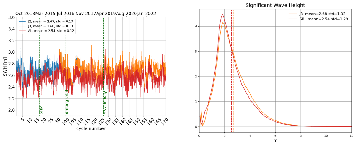
Figure 6: Daily monitoring of significant wave height for AltiKa (Ka-band) Jason-2 and Jason-3 (Ku-band) on the left and histogram for cycle 170 on the right (limited to 66° latitude).
