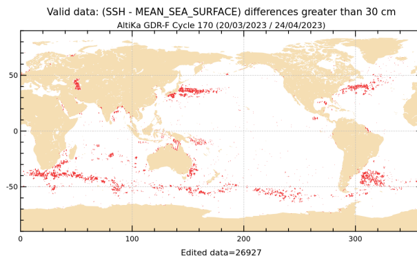
Figure 20: SLA higher than 30 cm for cycle 170.
