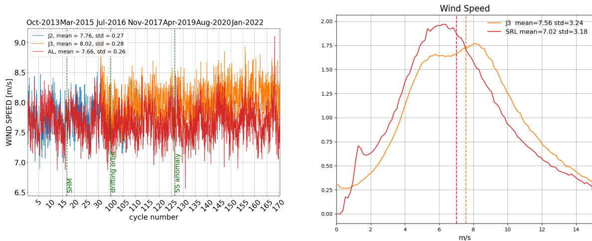
Figure 10: Daily monitoring of altimeter wind speed for Saral/AltiKa, Jason-2 and Jason-3 on the left and histogram for cycle 170 on the right (limited to 66° latitude).
