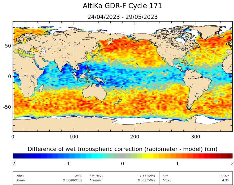
Figure 11: Mean of wet troposphere correction difference (Radiometer-ECMWF model) for cycle 171.
