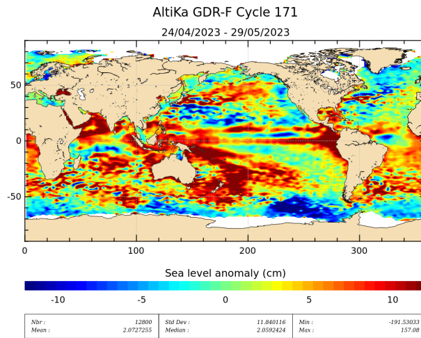
Figure 19: Sea level anomaly relative to MSS for cycle 171.
