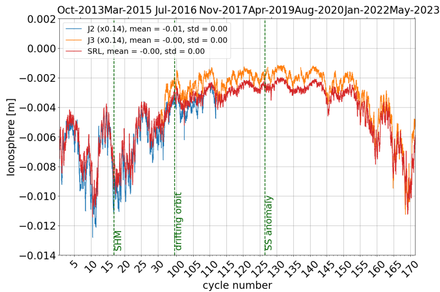
Figure 8: Daily monitoring of dual-frequency ionosphere correction for Jason-2 Jason-3 and GIM ionosphere correction for Saral/AltiKa.
