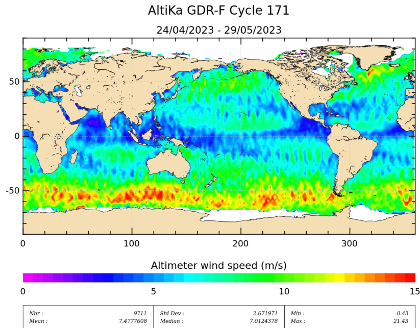
Figure 9: Altimeter wind speed for cycle 171.
