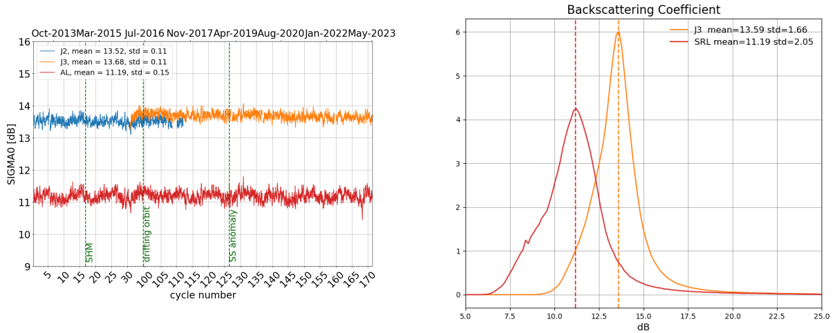
Figure 7: Daily monitoring of backscattering coefficient for Saral/AltiKa, Jason-2 and Jason-3 on the left and histogram for cycle 171 on the right (limited to 66° latitude).
