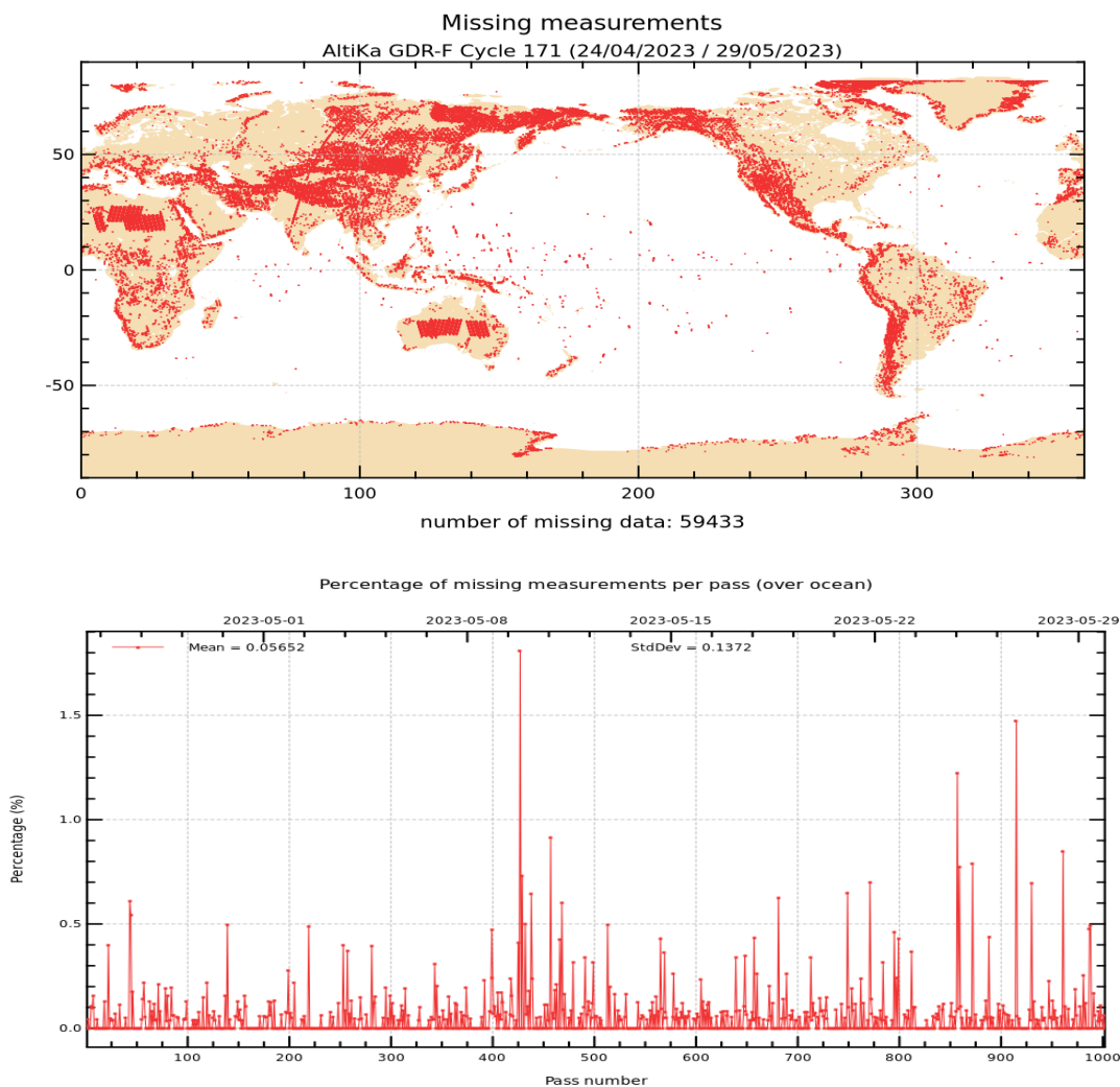
Figure 1: Map of missing measurements for cycle 171 on top. Monitoring of percentage of missing ocean measurements per pass on bottom.
