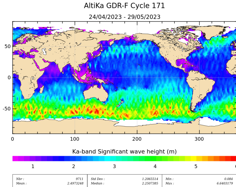
Figure 5: Significant wave height for cycle 171.
