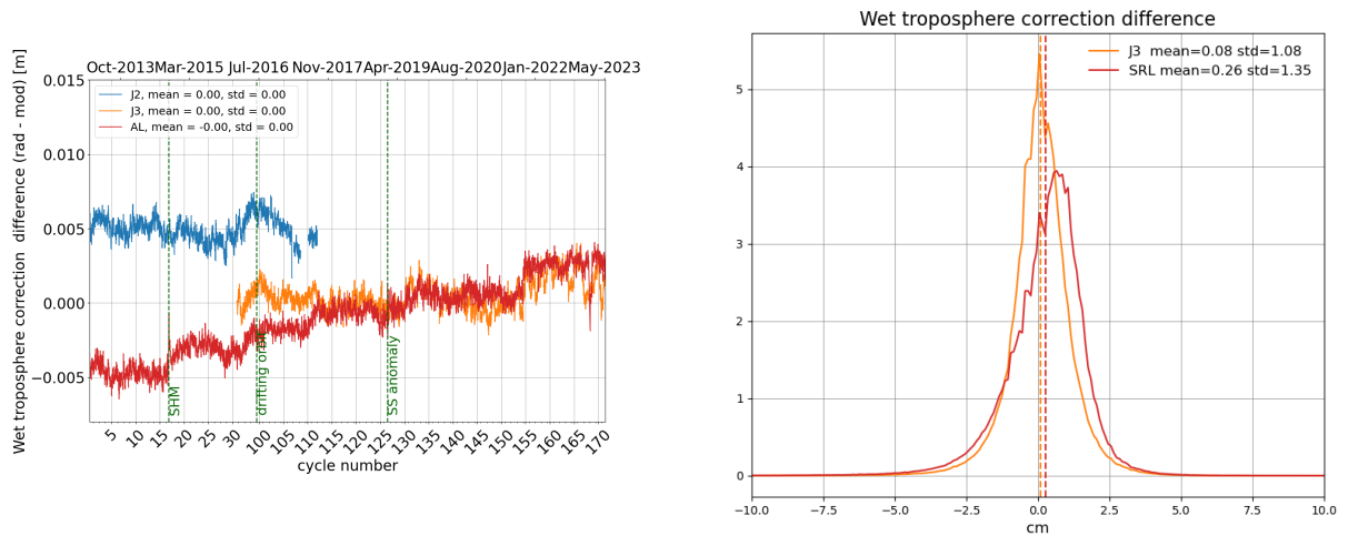
Figure 12: Daily monitoring of wet troposphere differences (Radiometer-ECMWF model) for Saral/AltiKa Jason-2 and Jason-3 (left) and histogram on the right (limited to 66° latitude) for cycle 171 .
