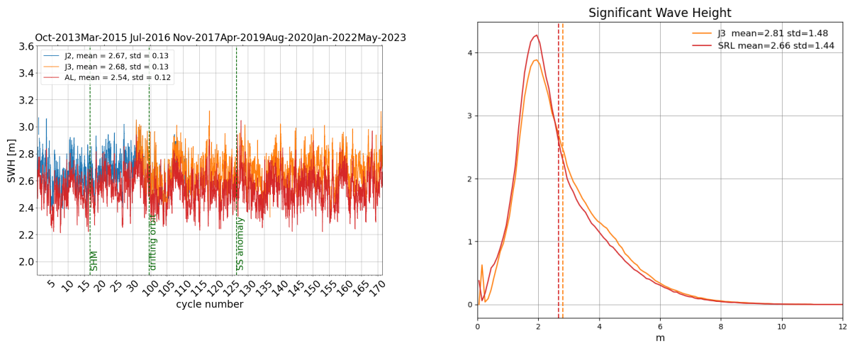
Figure 6: Daily monitoring of significant wave height for AltiKa (Ka-band) Jason-2 and Jason-3 (Ku-band) on the left and histogram for cycle 171 on the right (limited to 66^\circ latitude).
