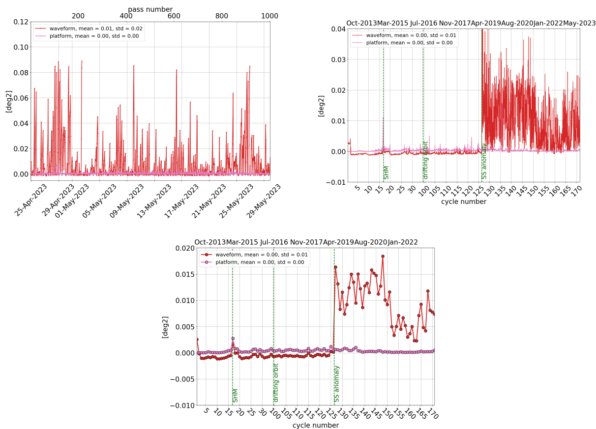
Figure 13: Monitoring per pass for cycle 171 (left), daily monitoring(right) and cyclic monitoring (bottom) of SARAL/AltiKa's mispointing angle: comparison between the one derived from waveform retracking and the one measured by platform startrackers.
