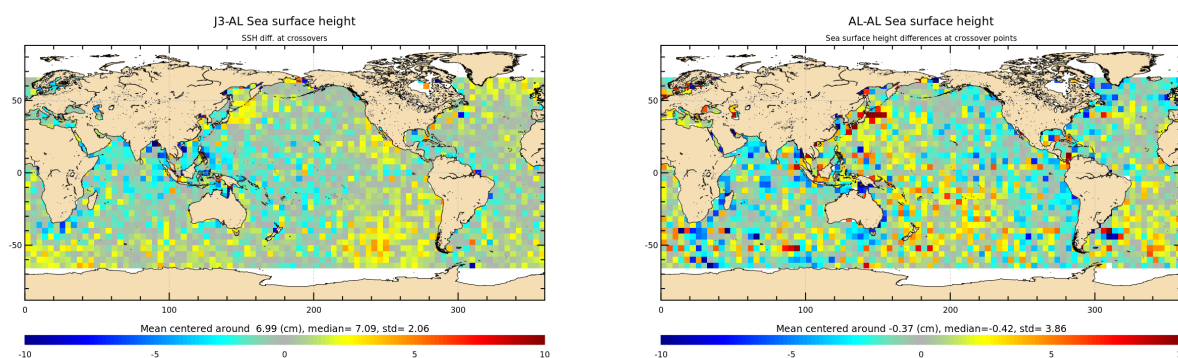
Figure 14: Mean of multi-mission SSH and mono-mission SSH differences at crossovers for cycle 171.
