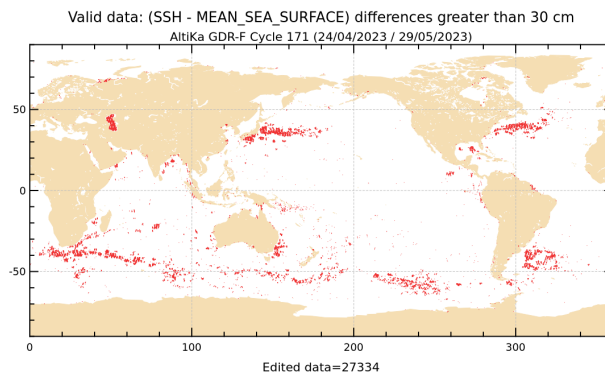
Figure 20: SLA higher than 30 cm for cycle 171.
