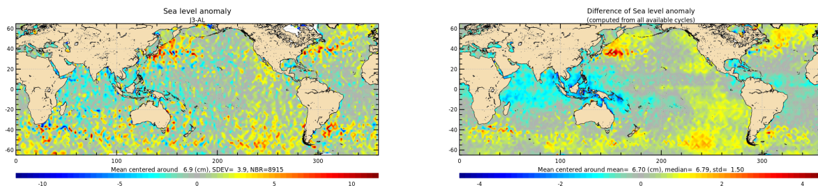
Figure 21: Jason-3 – Saral/AltiKa SLA differences for cycle 171 (left) and averaged over the whole Saral/AltiKa period (right).
