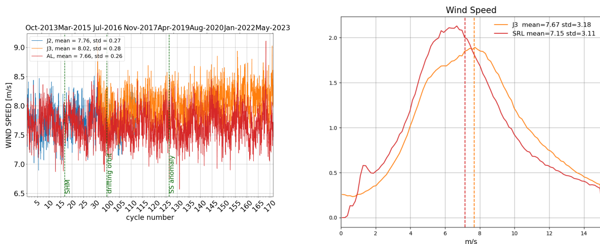
Figure 10: Daily monitoring of altimeter wind speed for Saral/AltiKa, Jason-2 and Jason-3 on the left and histogram for cycle 171 on the right (limited to 66° latitude).
