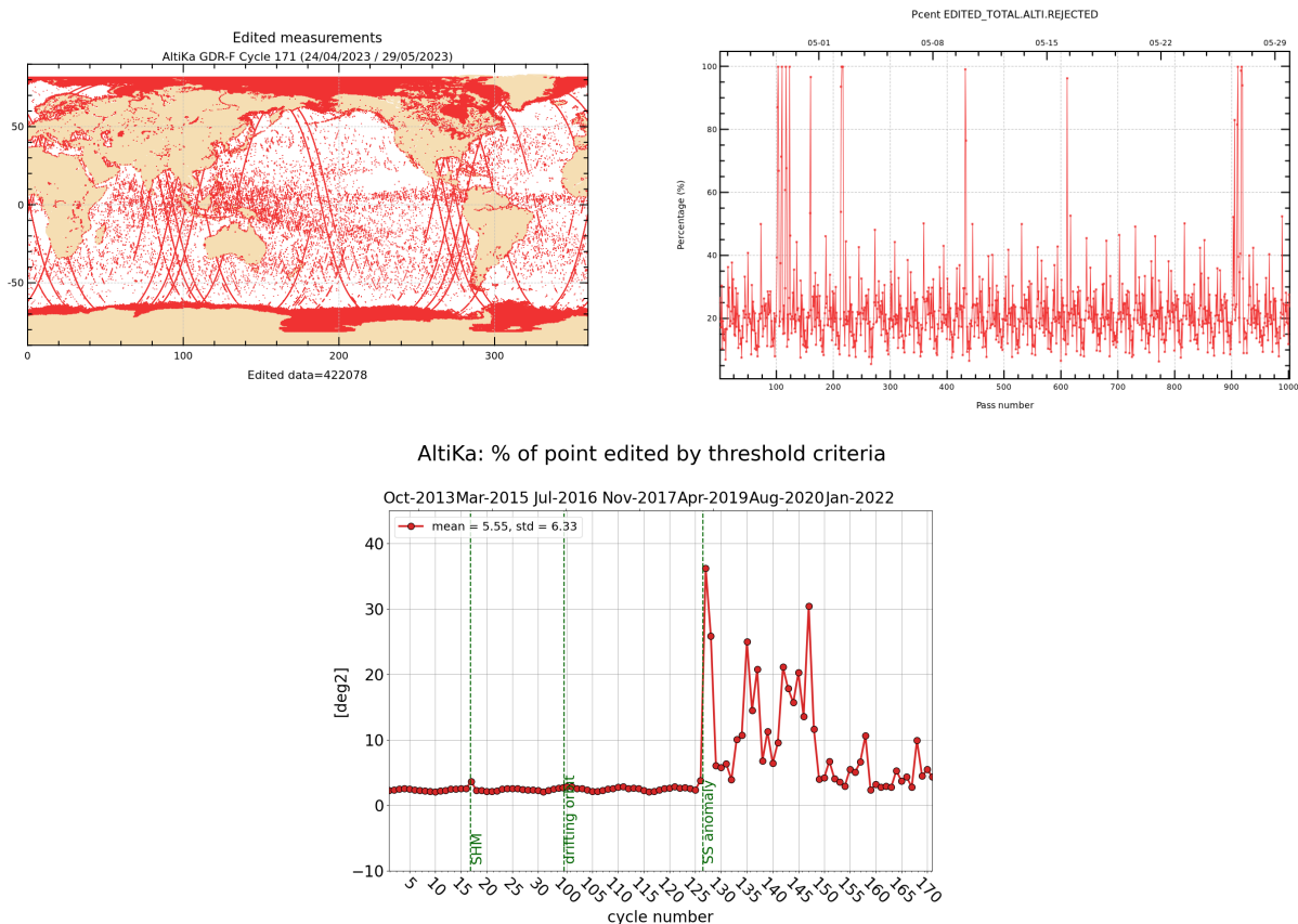
Figure 2: Rejected measurements on thresholds criteria : Cycle 171, map and monitoring of % of rejected measurements per track (top), whole time serie / % of rejected measurements per cycle (bottom).
