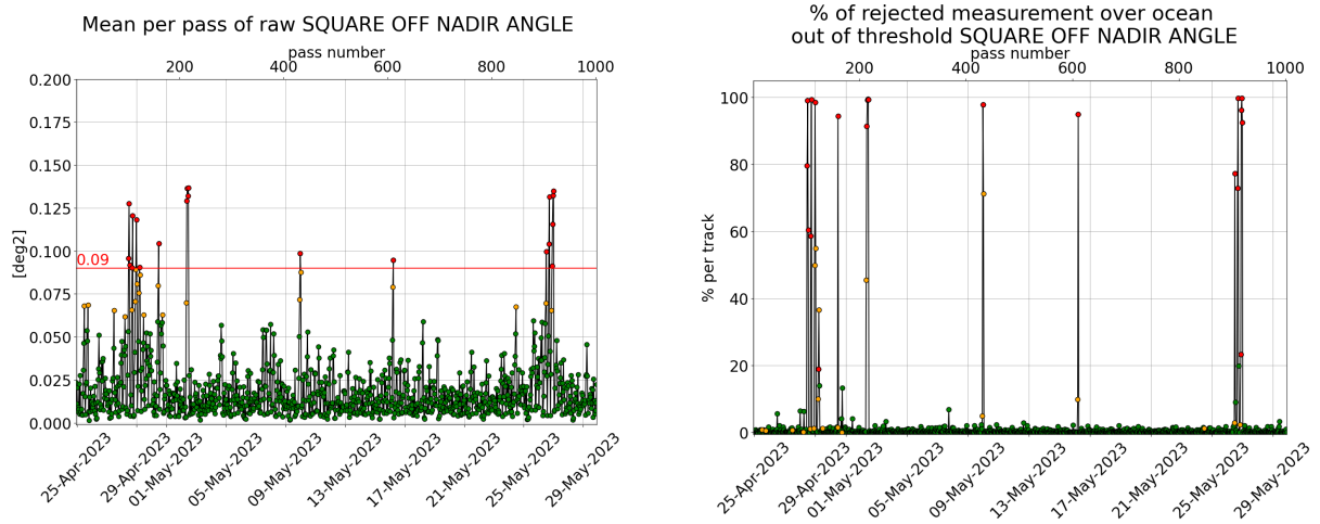
Figure 3: [left] Mispointing cycle 171, [right] Percentage of rejected measurement by threshold on square off-nadir angle.
