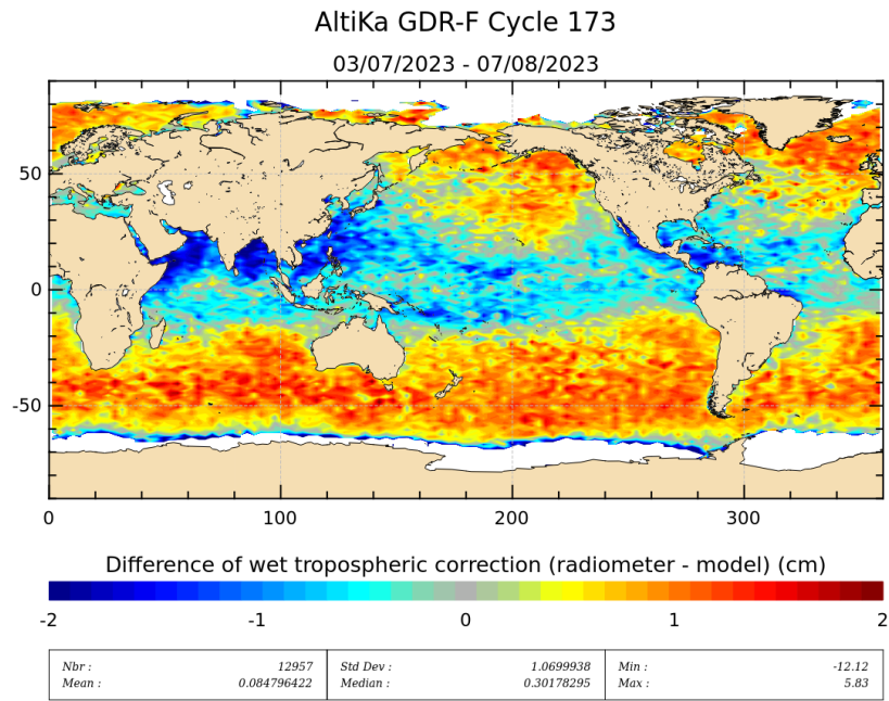
Figure 11: Mean of wet troposphere correction difference (Radiometer-ECMWF model) for cycle 173.
