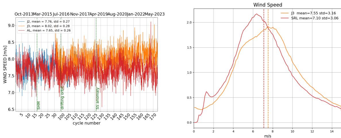
Figure 10: Daily monitoring of altimeter wind speed for Saral/AltiKa, Jason-2 and Jason-3 on the left and histogram for cycle 173 on the right (limited to 66° latitude).
