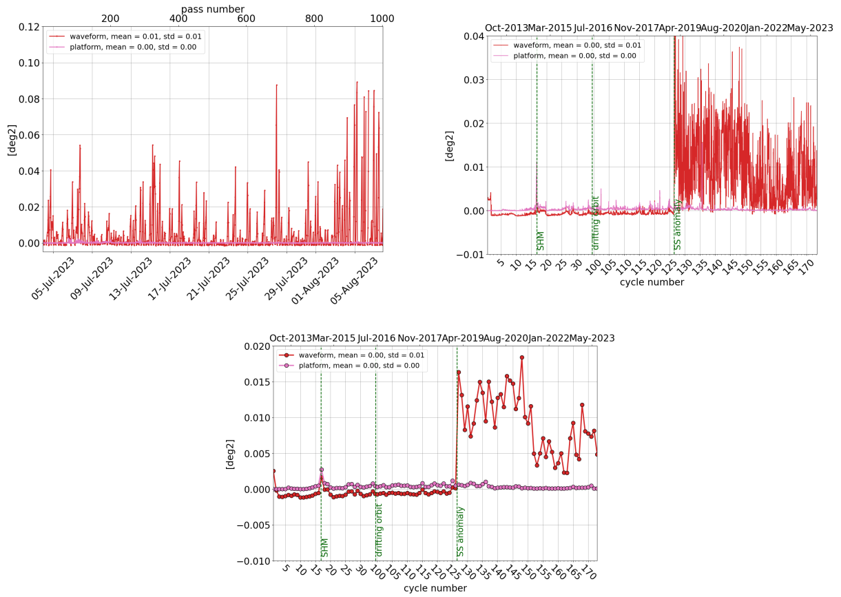
Figure 13: Monitoring per pass for cycle 173 (left), daily monitoring(right) and cyclic monitoring (bottom) of SARAL/AltiKa's mispointing angle: comparison between the one derived from waveform retracking and the one measured by platform startrackers.
