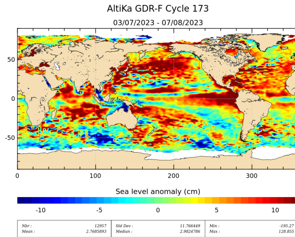
Figure 19: Sea level anomaly relative to MSS for cycle 173.
