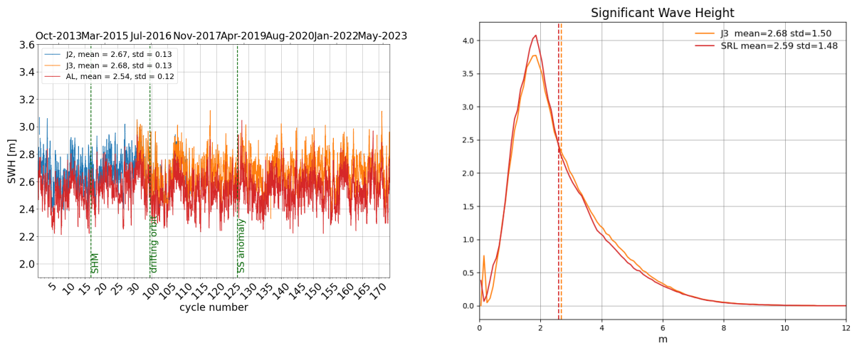
Figure 6: Daily monitoring of significant wave height for AltiKa (Ka-band) Jason-2 and Jason-3 (Ku-band) on the left and histogram for cycle 173 on the right (limited to 66^\circ latitude).
