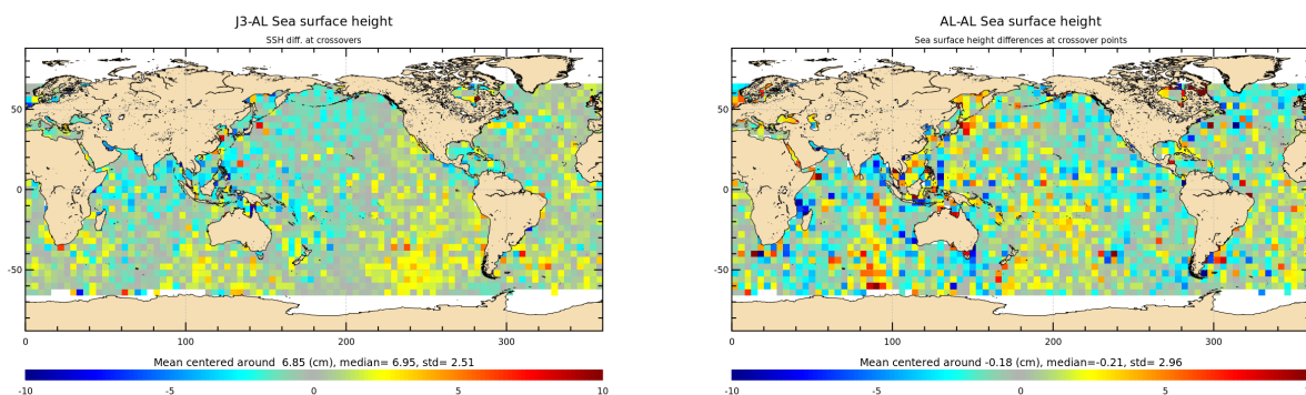
Figure 14: Mean of multi-mission SSH and mono-mission SSH differences at crossovers for cycle 173.
