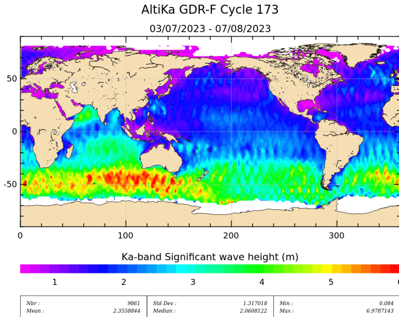
Figure 5: Significant wave height for cycle 173.
