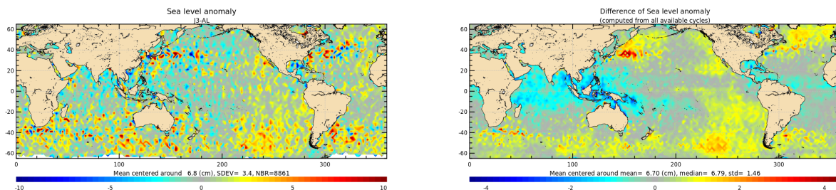
Figure 21: Jason-3 – Saral/AltiKa SLA differences for cycle 173 (left) and averaged over the whole Saral/AltiKa period (right).
