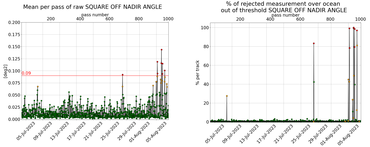
Figure 3: [left] Mispointing cycle 173, [right] Percentage of rejected measurement by threshold on square off-nadir angle.
