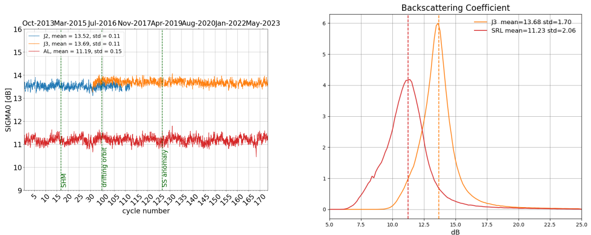
Figure 7: Daily monitoring of backscattering coefficient for Saral/AltiKa, Jason-2 and Jason-3 on the left and histogram for cycle 173 on the right (limited to 66° latitude).
