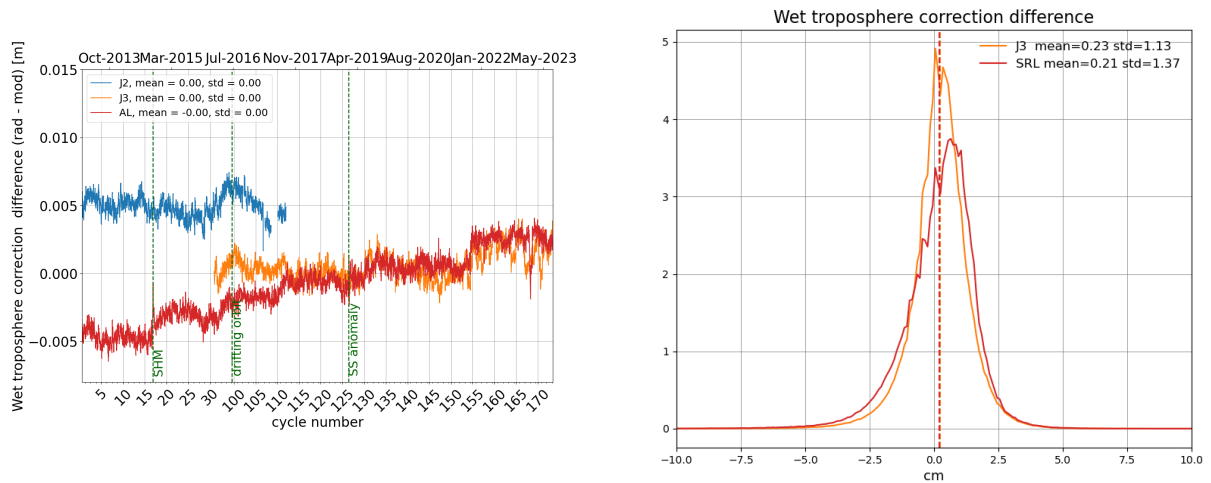
Figure 12: Daily monitoring of wet troposphere differences (Radiometer-ECMWF model) for Saral/AltiKa Jason-2 and Jason-3 (left) and histogram on the right (limited to 66° latitude) for cycle 173 .
