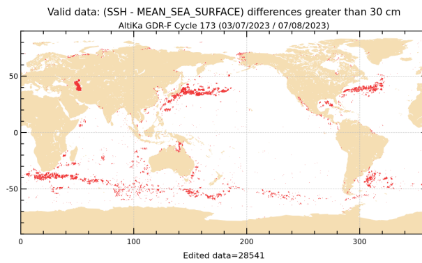
Figure 20: SLA higher than 30 cm for cycle 173.
