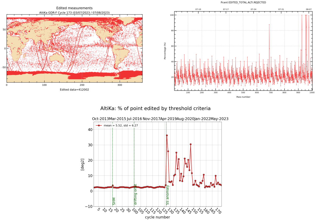
Figure 2: Rejected measurements on thresholds criteria : Cycle 173, map and monitoring of % of rejected measurements per track (top), whole time serie / % of rejected measurements per cycle (bottom).
