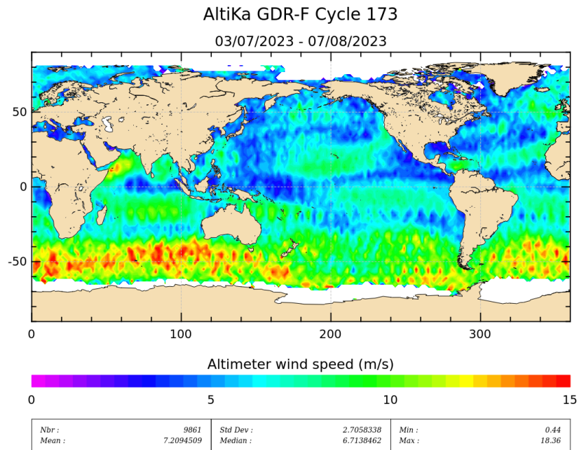
Figure 9: Altimeter wind speed for cycle 173.
