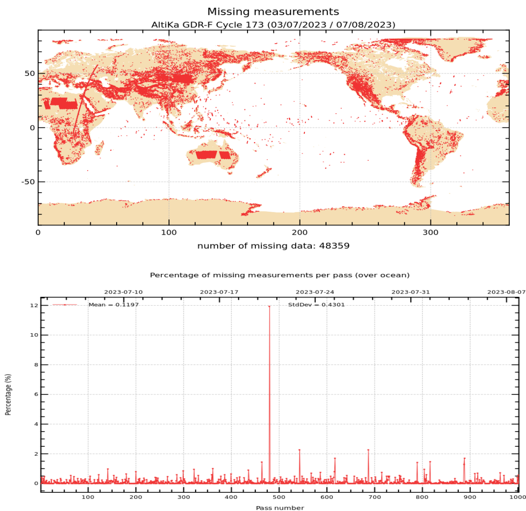
Figure 1: Map of missing measurements for cycle 173 on top. Monitoring of percentage of missing ocean measurements per pass on bottom.
