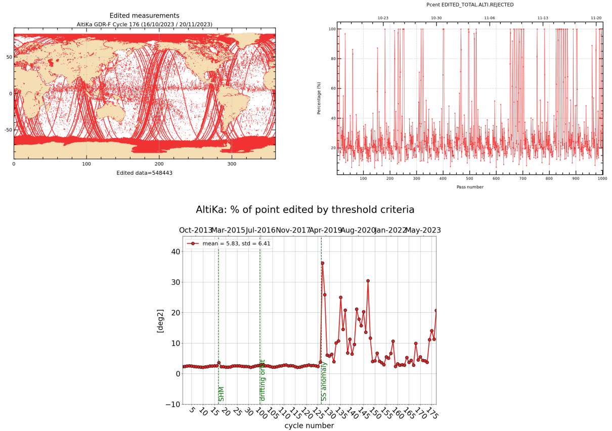
Figure 2: Rejected measurements on thresholds criteria : Cycle 176, map and monitoring of % of rejected measurements per track (top), whole time serie / % of rejected measurements per cycle (bottom).
