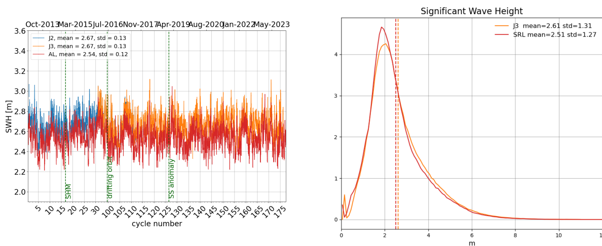
Figure 6: Daily monitoring of significant wave height for AltiKa (Ka-band) Jason-2 and Jason-3 (Ku-band) on the left and histogram for cycle 176 on the right (limited to 66^\circ latitude).
