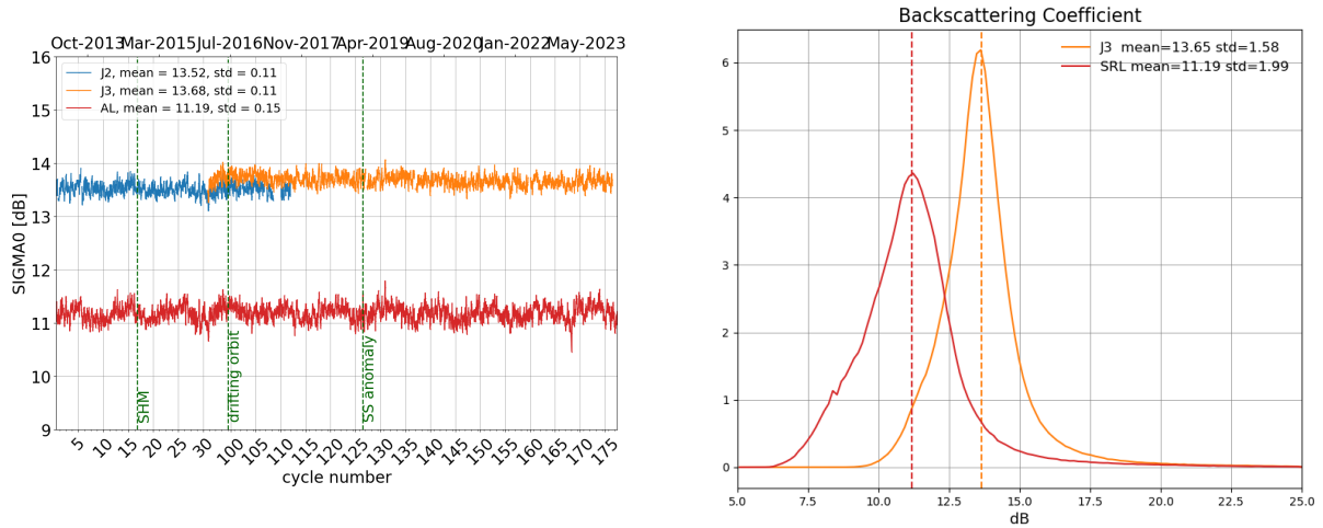
Figure 7: Daily monitoring of backscattering coefficient for Saral/AltiKa, Jason-2 and Jason-3 on the left and histogram for cycle 176 on the right (limited to 66° latitude).
