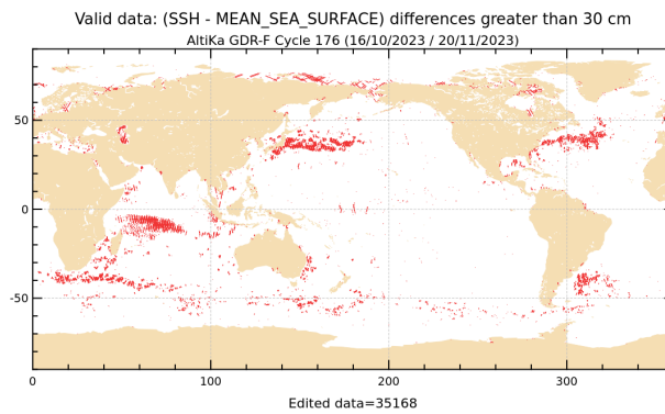
Figure 20: SLA higher than 30 cm for cycle 176.
