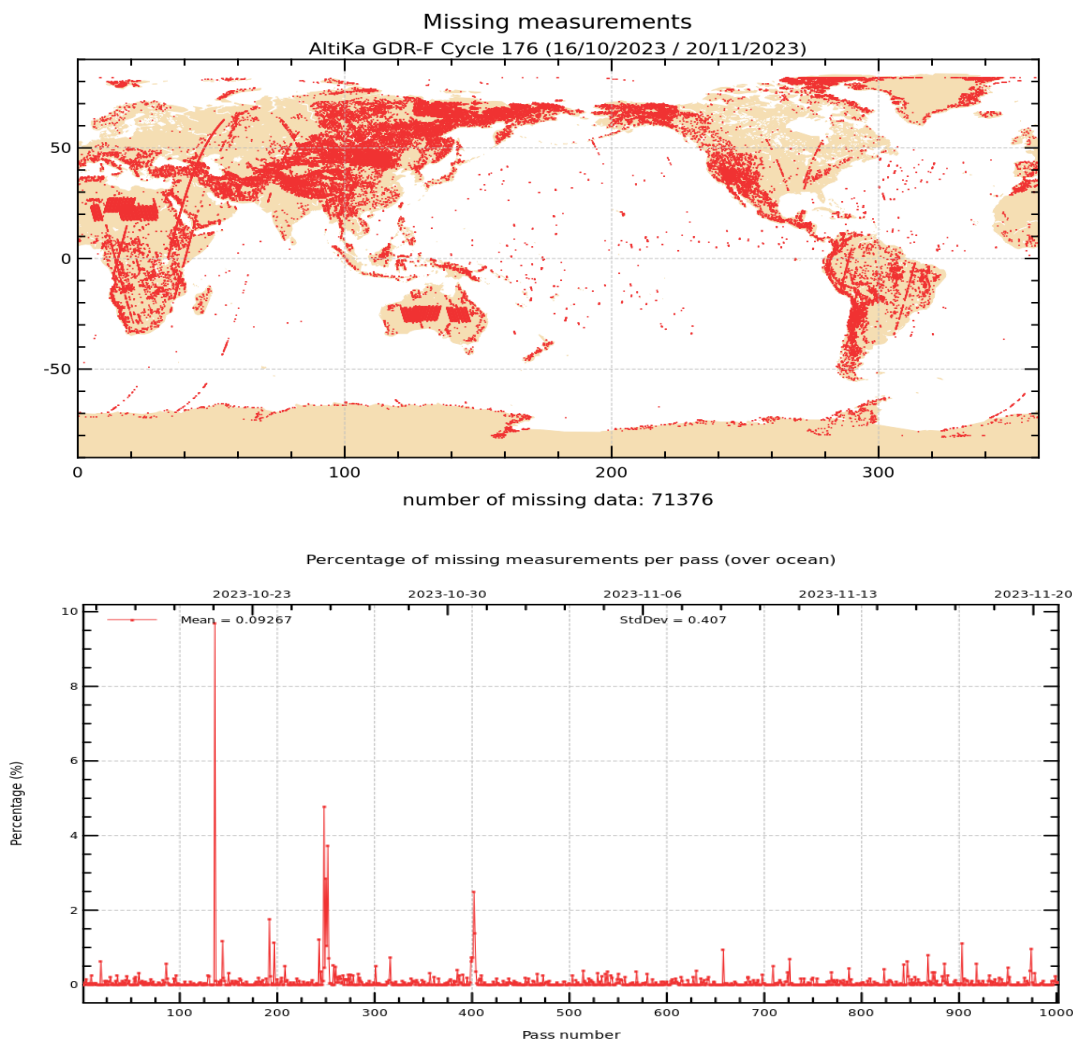
Figure 1: Map of missing measurements for cycle 176 on top. Monitoring of percentage of missing ocean measurements per pass on bottom.
