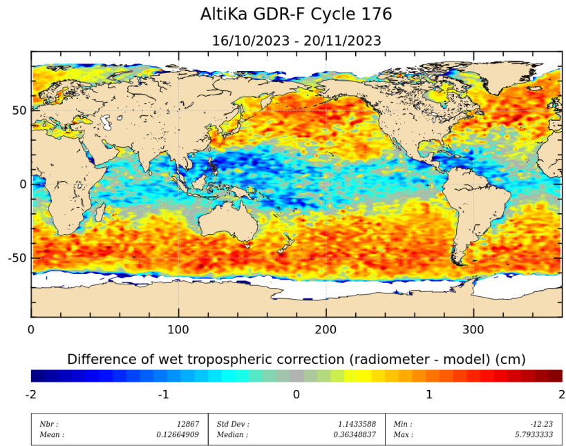
Figure 11: Mean of wet troposphere correction difference (Radiometer-ECMWF model) for cycle 176.
