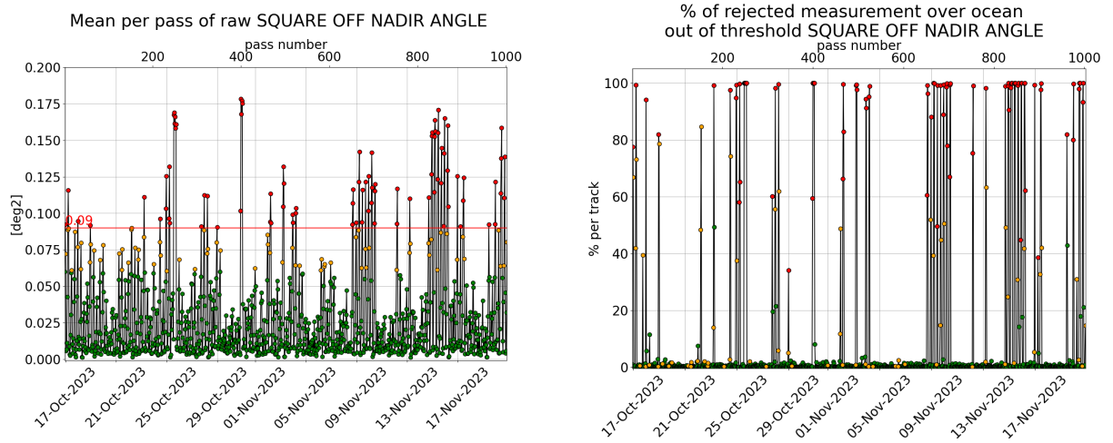
Figure 3: [left] Mispointing cycle 176, [right] Percentage of rejected measurement by threshold on square off-nadir angle.
