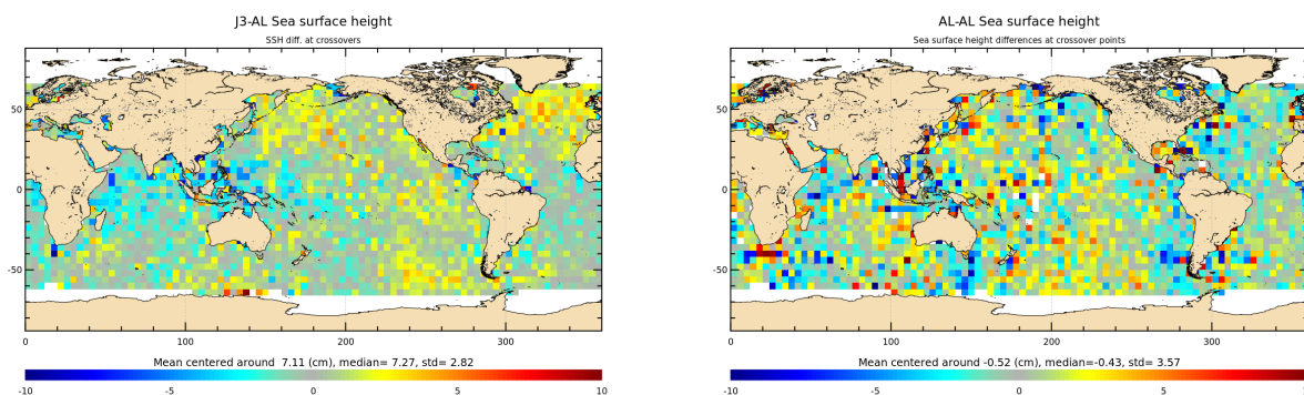
Figure 14: Mean of multi-mission SSH and mono-mission SSH differences at crossovers for cycle 176.
