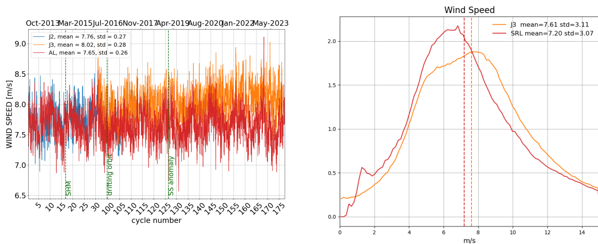
Figure 10: Daily monitoring of altimeter wind speed for Saral/AltiKa, Jason-2 and Jason-3 on the left and histogram for cycle 176 on the right (limited to 66° latitude).
