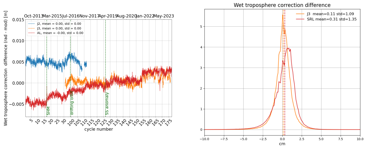
Figure 12: Daily monitoring of wet troposphere differences (Radiometer-ECMWF model) for Saral/AltiKa Jason-2 and Jason-3 (left) and histogram on the right (limited to 66° latitude) for cycle 176 .
