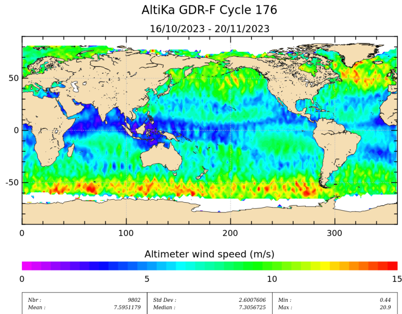
Figure 9: Altimeter wind speed for cycle 176.
