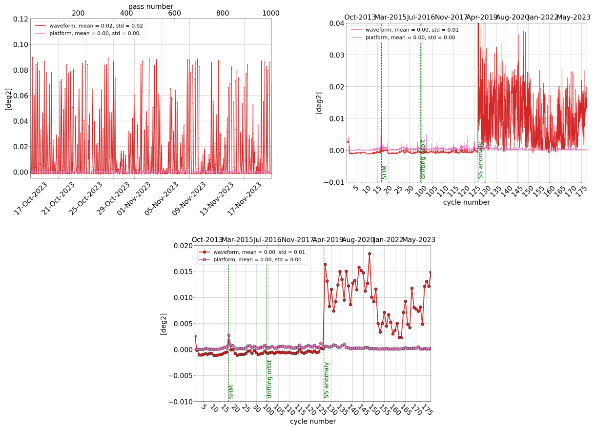
Figure 13: Monitoring per pass for cycle 176 (left), daily monitoring(right) and cyclic monitoring (bottom) of SARAL/AltiKa's mispointing angle: comparison between the one derived from waveform retracking and the one measured by platform startrackers.
