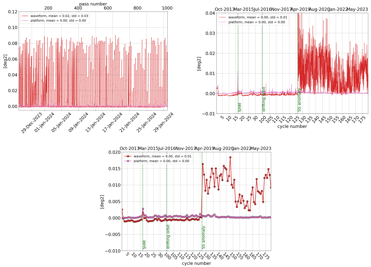
Figure 13: Monitoring per pass for cycle 178 (left), daily monitoring(right) and cyclic monitoring (bottom) of SARAL/AltiKa's mispointing angle: comparison between the one derived from waveform retracking and the one measured by platform startrackers.
