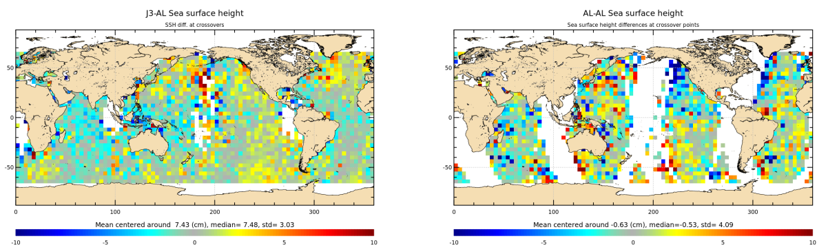
Figure 14: Mean of multi-mission SSH and mono-mission SSH differences at crossovers for cycle 178.
