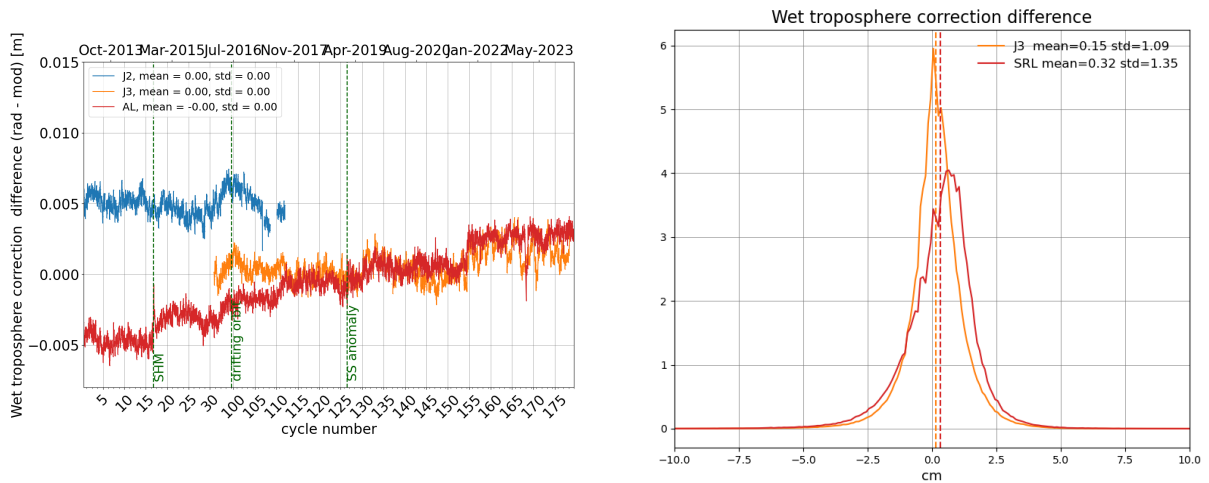
Figure 12: Daily monitoring of wet troposphere differences (Radiometer-ECMWF model) for Saral/AltiKa Jason-2 and Jason-3 (left) and histogram on the right (limited to 66° latitude) for cycle 178 .
