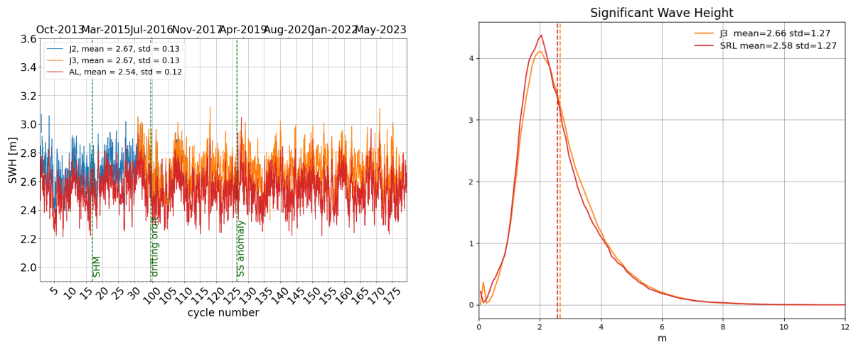
Figure 6: Daily monitoring of significant wave height for AltiKa (Ka-band) Jason-2 and Jason-3 (Ku-band) on the left and histogram for cycle 178 on the right (limited to 66° latitude).
