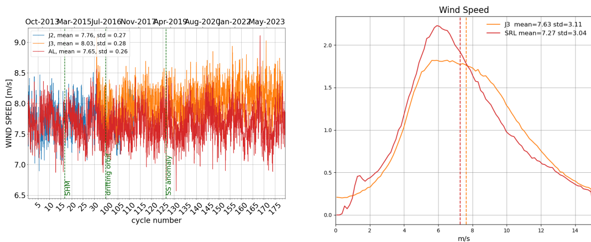
Figure 10: Daily monitoring of altimeter wind speed for Saral/AltiKa, Jason-2 and Jason-3 on the left and histogram for cycle 178 on the right (limited to 66° latitude).
