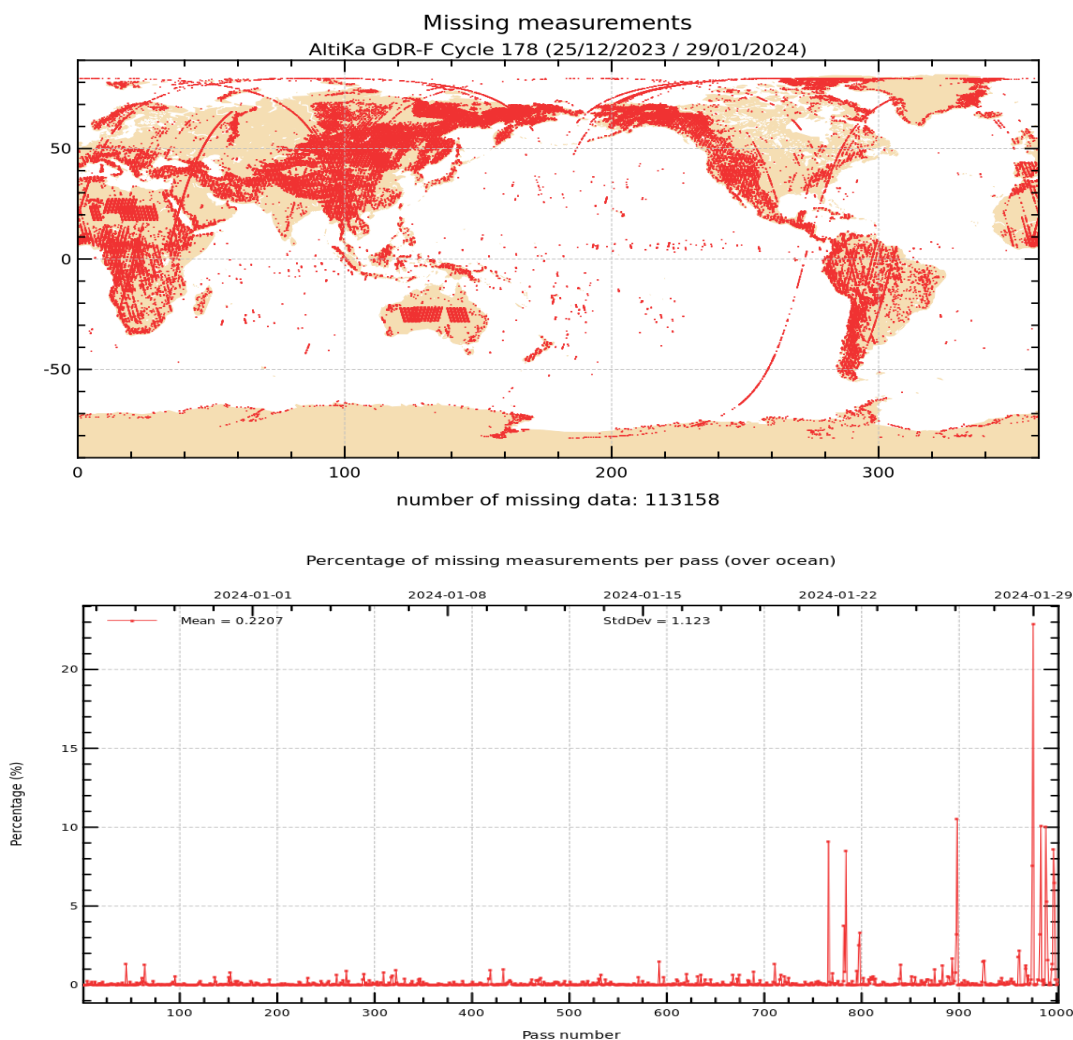
Figure 1: Map of missing measurements for cycle 178 on top. Monitoring of percentage of missing ocean measurements per pass on bottom.
