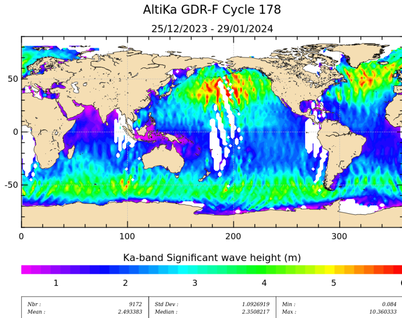
Figure 5: Significant wave height for cycle 178.
