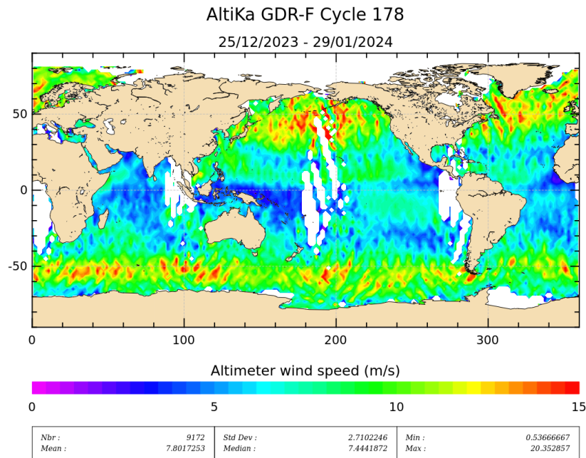
Figure 9: Altimeter wind speed for cycle 178.
