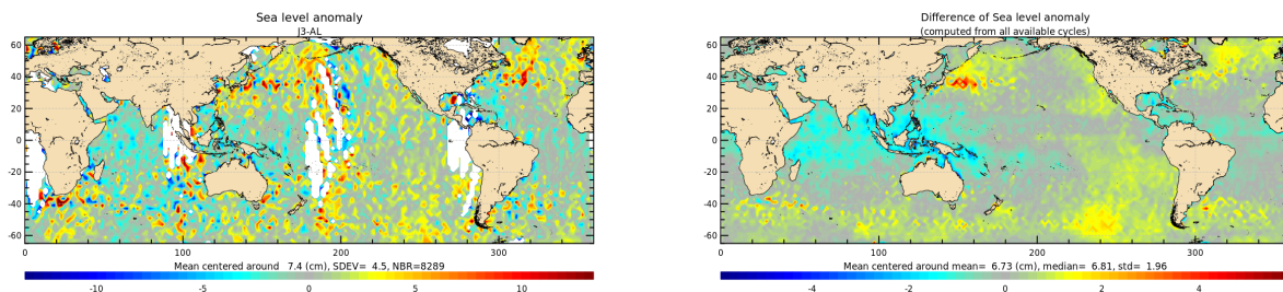
Figure 21: Jason-3 – Saral/AltiKa SLA differences for cycle 178 (left) and averaged over the whole Saral/AltiKa period (right).
