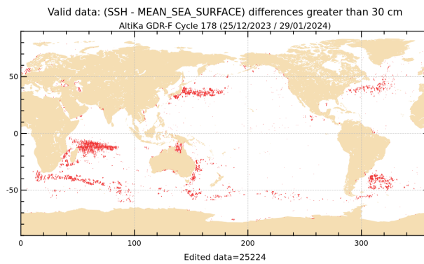
Figure 20: SLA higher than 30 cm for cycle 178.
