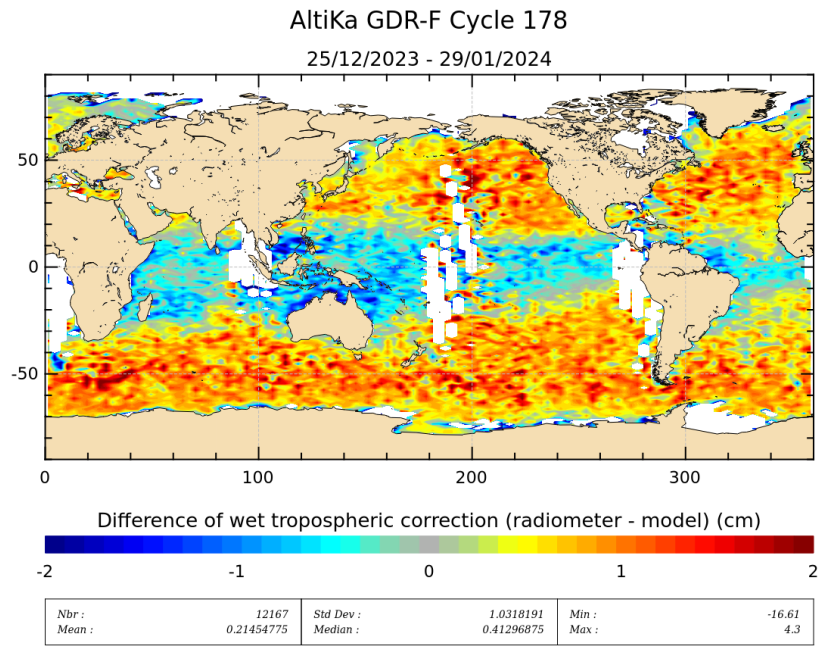
Figure 11: Mean of wet troposphere correction difference (Radiometer-ECMWF model) for cycle 178.
