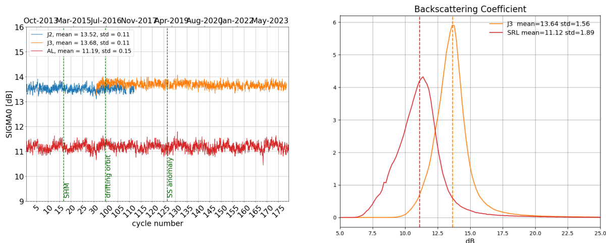
Figure 7: Daily monitoring of backscattering coefficient for Saral/AltiKa, Jason-2 and Jason-3 on the left and histogram for cycle 178 on the right (limited to 66° latitude).
