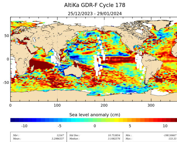
Figure 19: Sea level anomaly relative to MSS for cycle 178.
