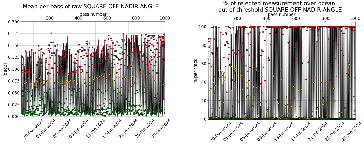
Figure 3: [left] Mispointing cycle 178, [right] Percentage of rejected measurement by threshold on square off-nadir angle.
