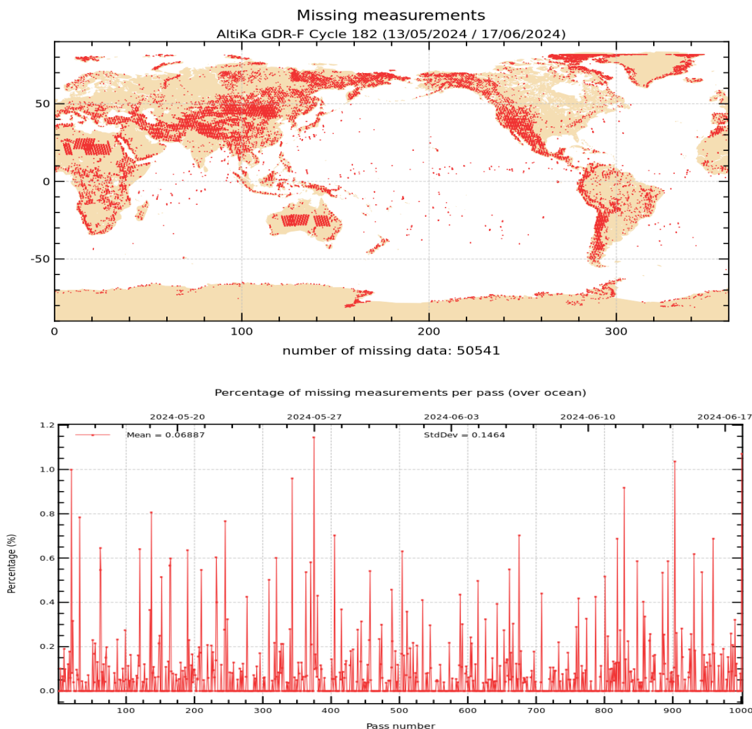
Figure 1: Map of missing measurements for cycle 182 on top. Monitoring of percentage of missing ocean measurements per pass on bottom.
