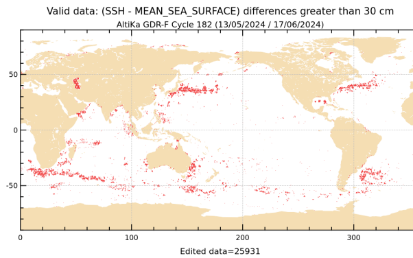
Figure 20: SLA higher than 30 cm for cycle 182.
