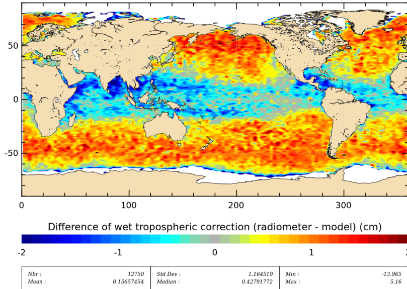
Figure 11: Mean of wet troposphere correction difference (Radiometer-ECMWF model) for cycle 182.
