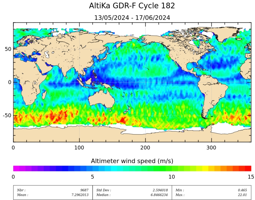
Figure 9: Altimeter wind speed for cycle 182.
