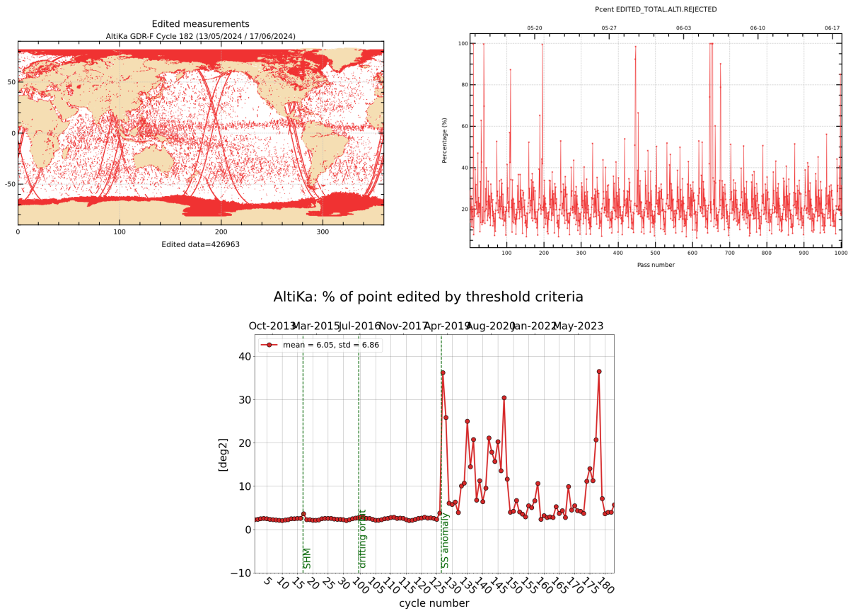
Figure 2: Rejected measurements on thresholds criteria : Cycle 182, map and monitoring of % of rejected measurements per track (top), whole time serie / % of rejected measurements per cycle (bottom).
