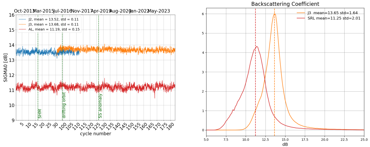
Figure 7: Daily monitoring of backscattering coefficient for Saral/AltiKa, Jason-2 and Jason-3 on the left and histogram for cycle 182 on the right (limited to 66° latitude).
