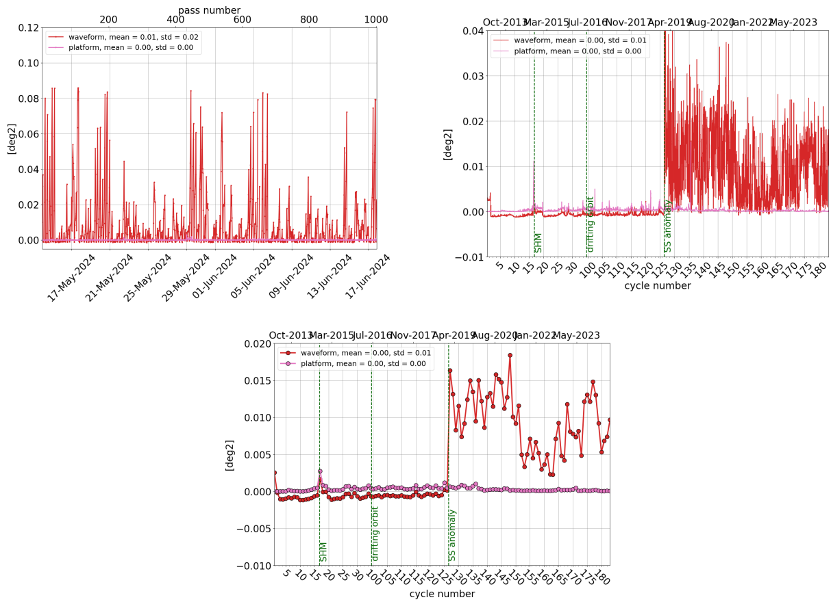
Figure 13: Monitoring per pass for cycle 182 (left), daily monitoring(right) and cyclic monitoring (bottom) of SARAL/AltiKa's mispointing angle: comparison between the one derived from waveform retracking and the one measured by platform startrackers.
