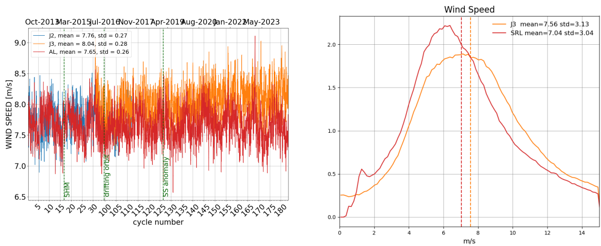
Figure 10: Daily monitoring of altimeter wind speed for Saral/AltiKa, Jason-2 and Jason-3 on the left and histogram for cycle 182 on the right (limited to 66° latitude).
