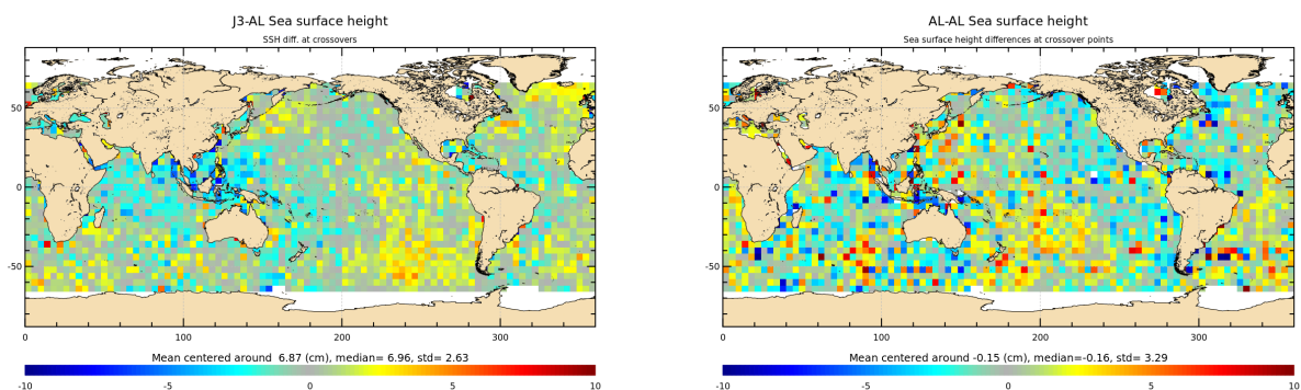
Figure 14: Mean of multi-mission SSH and mono-mission SSH differences at crossovers for cycle 182.
