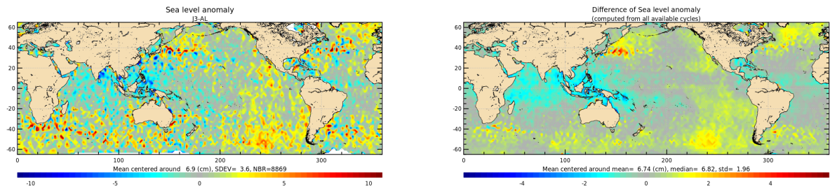
Figure 21: Jason-3 – Saral/AltiKa SLA differences for cycle 182 (left) and averaged over the whole Saral/AltiKa period (right).
