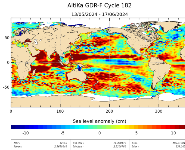
Figure 19: Sea level anomaly relative to MSS for cycle 182.
