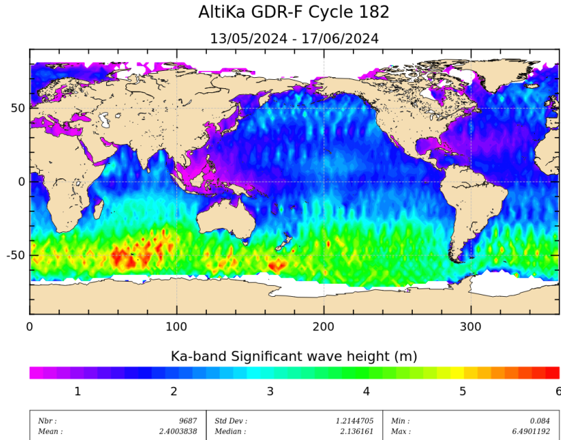
Figure 5: Significant wave height for cycle 182.
