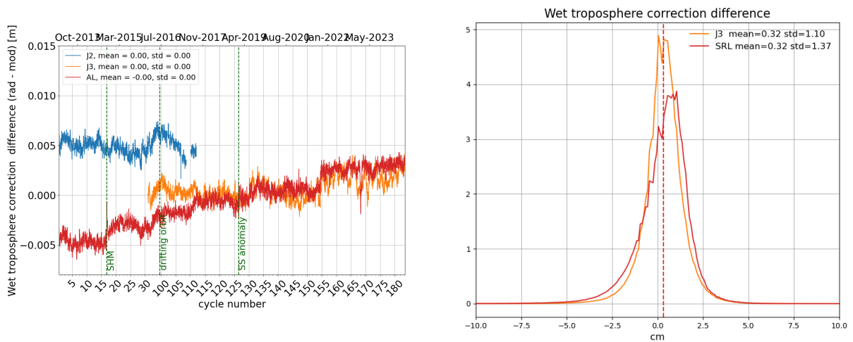
Figure 12: Daily monitoring of wet troposphere differences (Radiometer-ECMWF model) for Saral/AltiKa Jason-2 and Jason-3 (left) and histogram on the right (limited to 66° latitude) for cycle 182 .
