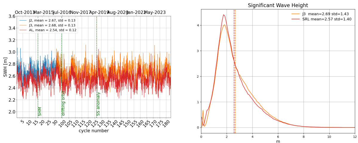
Figure 6: Daily monitoring of significant wave height for AltiKa (Ka-band) Jason-2 and Jason-3 (Ku-band) on the left and histogram for cycle 182 on the right (limited to 66° latitude).
