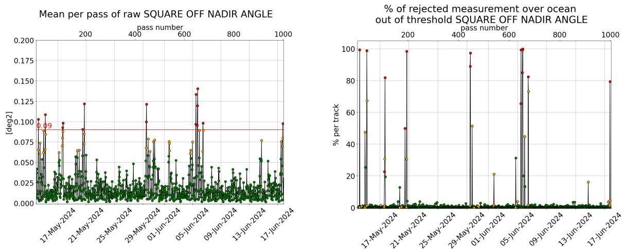
Figure 3: [left] Mispointing cycle 182, [right] Percentage of rejected measurement by threshold on square off-nadir angle.
