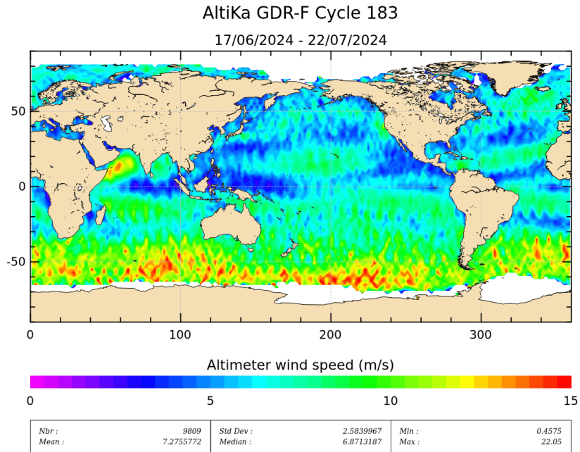
Figure 9: Altimeter wind speed for cycle 183.
