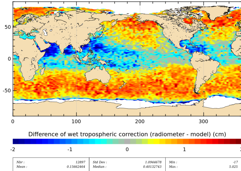
Figure 11: Mean of wet troposphere correction difference (Radiometer-ECMWF model) for cycle 183.
