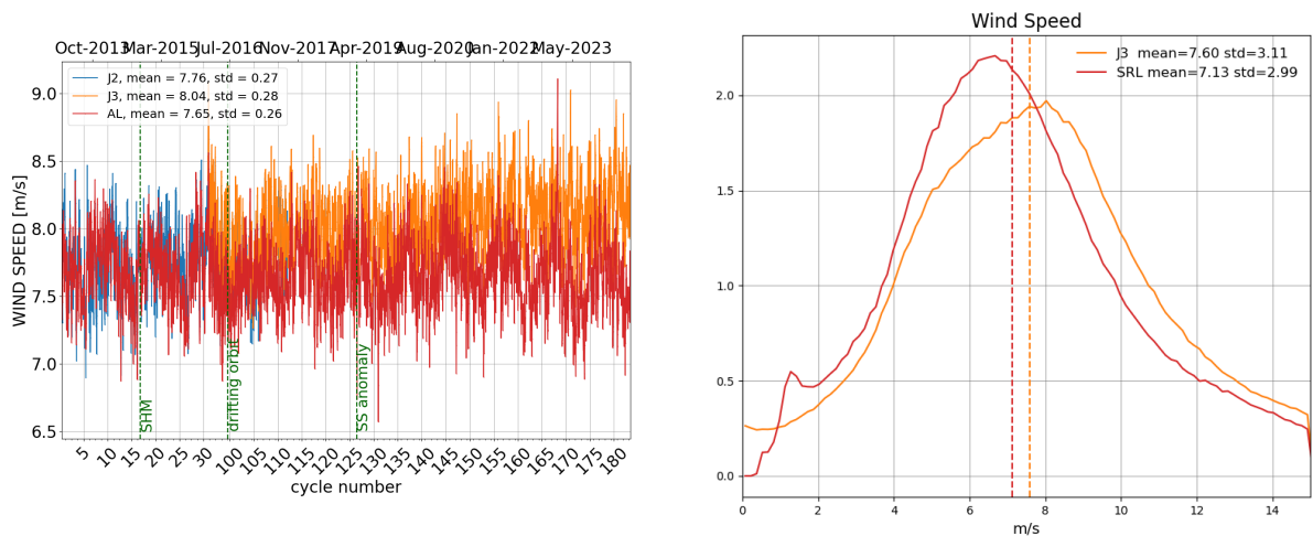
Figure 10: Daily monitoring of altimeter wind speed for Saral/AltiKa, Jason-2 and Jason-3 on the left and histogram for cycle 183 on the right (limited to 66° latitude).
