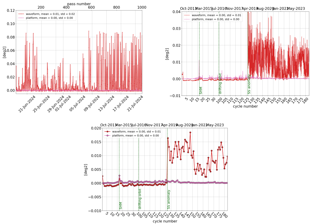
Figure 13: Monitoring per pass for cycle 183 (left), daily monitoring(right) and cyclic monitoring (bottom) of SARAL/AltiKa's mispointing angle: comparison between the one derived from waveform retracking and the one measured by platform startrackers.
