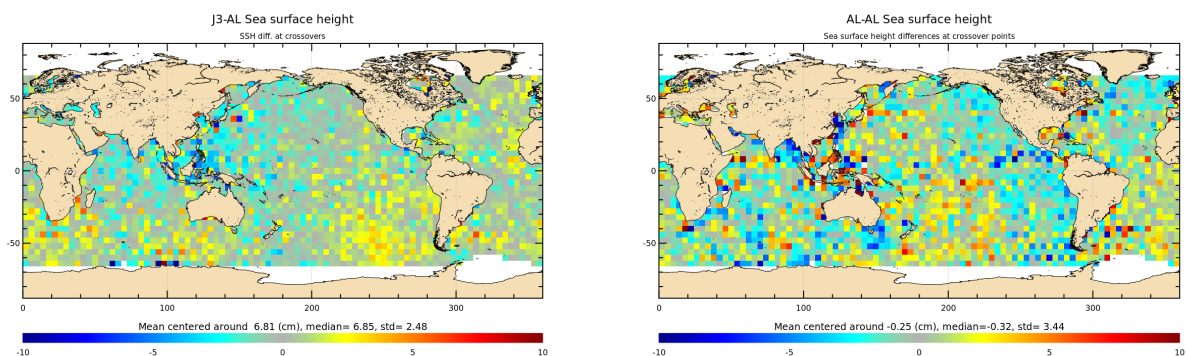
Figure 14: Mean of multi-mission SSH and mono-mission SSH differences at crossovers for cycle 183.
