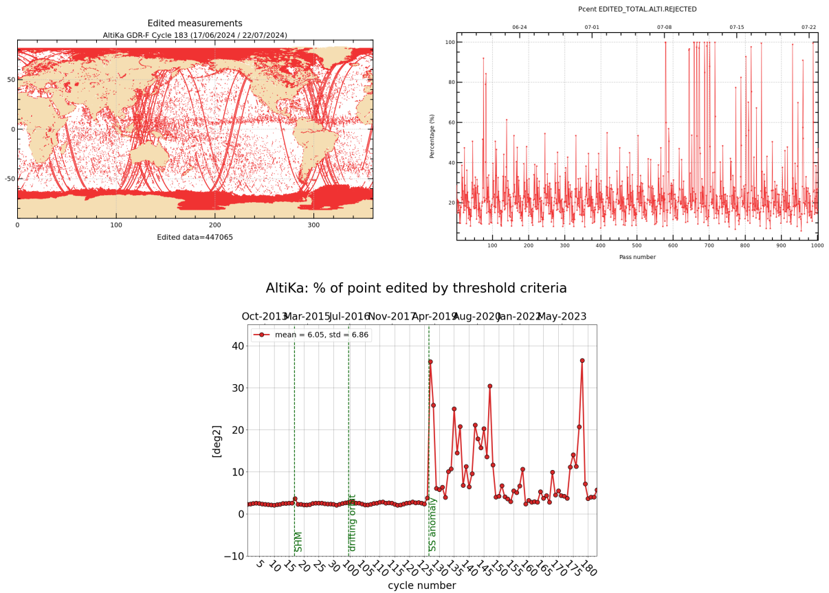
Figure 2: Rejected measurements on thresholds criteria : Cycle 183, map and monitoring of % of rejected measurements per track (top), whole time serie / % of rejected measurements per cycle (bottom).
