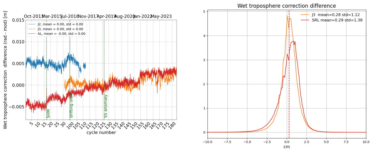
Figure 12: Daily monitoring of wet troposphere differences (Radiometer-ECMWF model) for Saral/AltiKa Jason-2 and Jason-3 (left) and histogram on the right (limited to 66° latitude) for cycle 183 .
