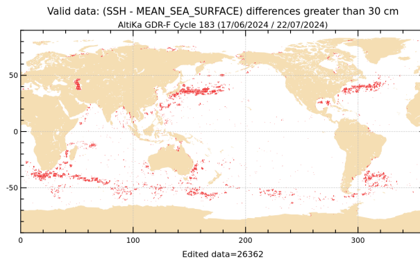
Figure 20: SLA higher than 30 cm for cycle 183.
