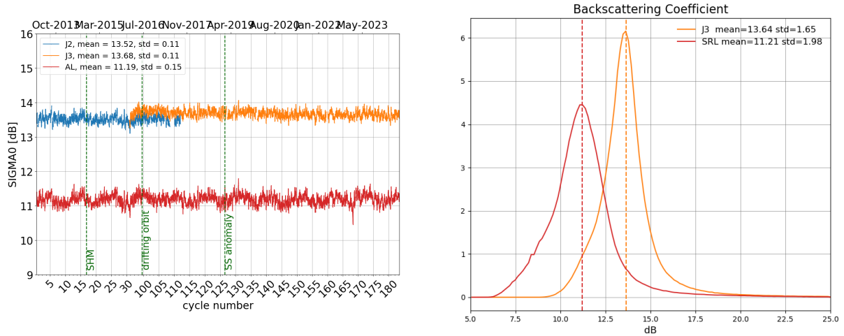
Figure 7: Daily monitoring of backscattering coefficient for Saral/AltiKa, Jason-2 and Jason-3 on the left and histogram for cycle 183 on the right (limited to 66° latitude).
