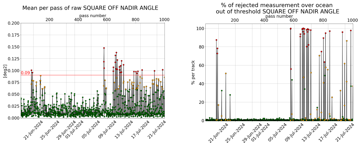
Figure 3: [left] Mispointing cycle 183, [right] Percentage of rejected measurement by threshold on square off-nadir angle.
