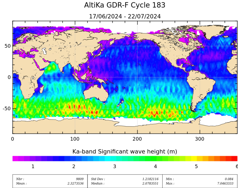
Figure 5: Significant wave height for cycle 183.
