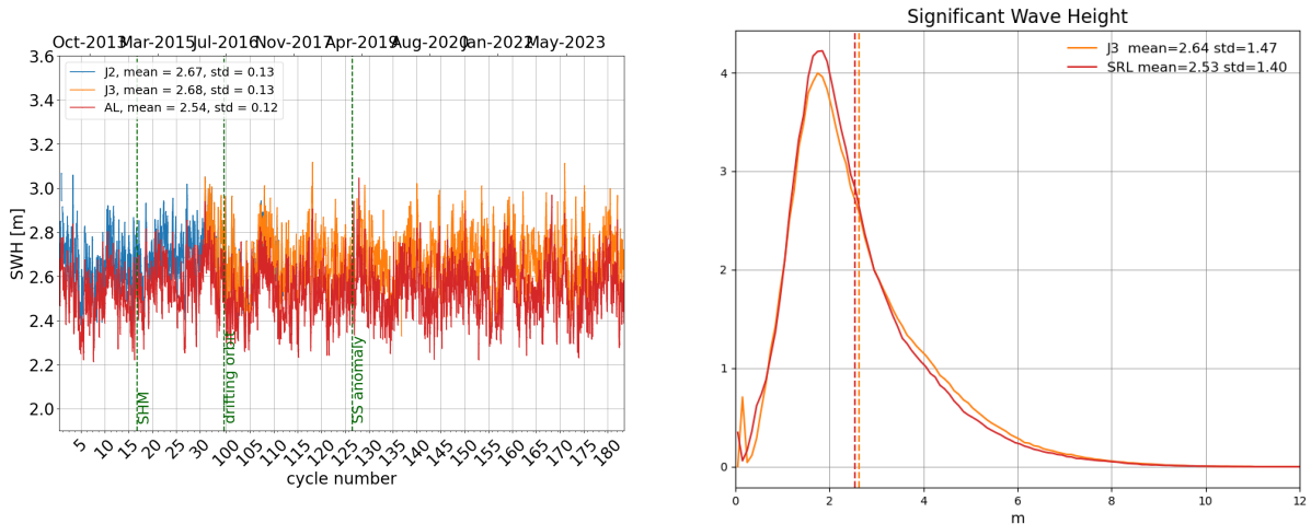
Figure 6: Daily monitoring of significant wave height for AltiKa (Ka-band) Jason-2 and Jason-3 (Ku-band) on the left and histogram for cycle 183 on the right (limited to 66^\circ latitude).
