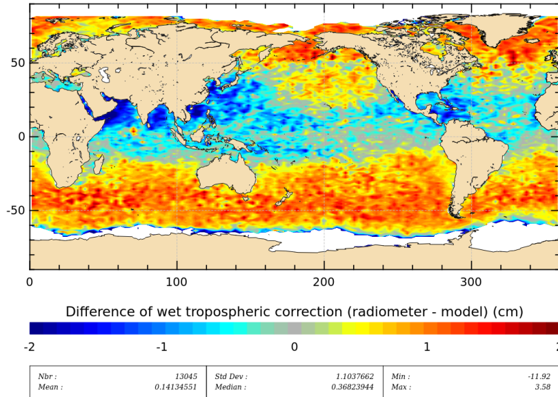
Figure 11: Mean of wet troposphere correction difference (Radiometer-ECMWF model) for cycle 184.
