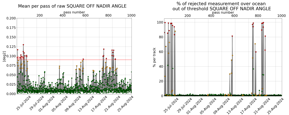
Figure 3: [left] Mispointing cycle 184, [right] Percentage of rejected measurement by threshold on square off-nadir angle.
