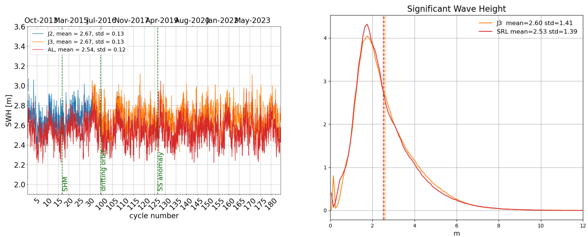
Figure 6: Daily monitoring of significant wave height for AltiKa (Ka-band) Jason-2 and Jason-3 (Ku-band) on the left and histogram for cycle 184 on the right (limited to 66^\circ latitude).
