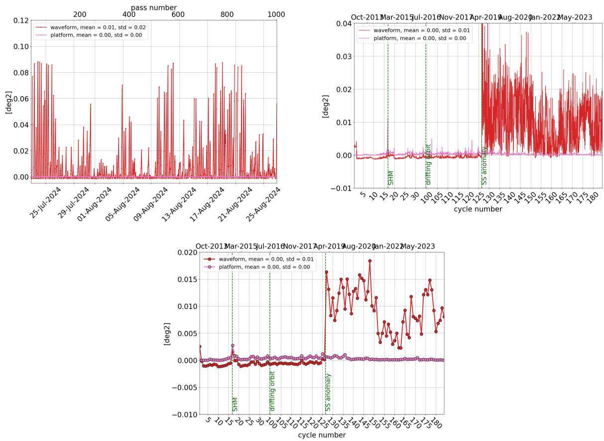
Figure 13: Monitoring per pass for cycle 184 (left), daily monitoring(right) and cyclic monitoring (bottom) of SARAL/AltiKa's mispointing angle: comparison between the one derived from waveform retracking and the one measured by platform startrackers.
