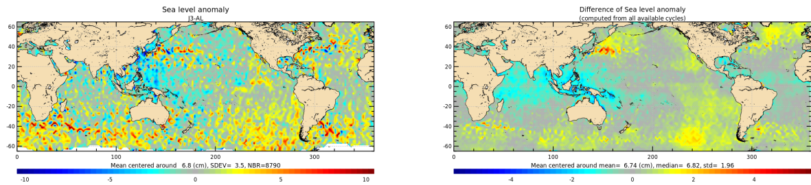
Figure 21: Jason-3 – Saral/AltiKa SLA differences for cycle 184 (left) and averaged over the whole Saral/AltiKa period (right).
