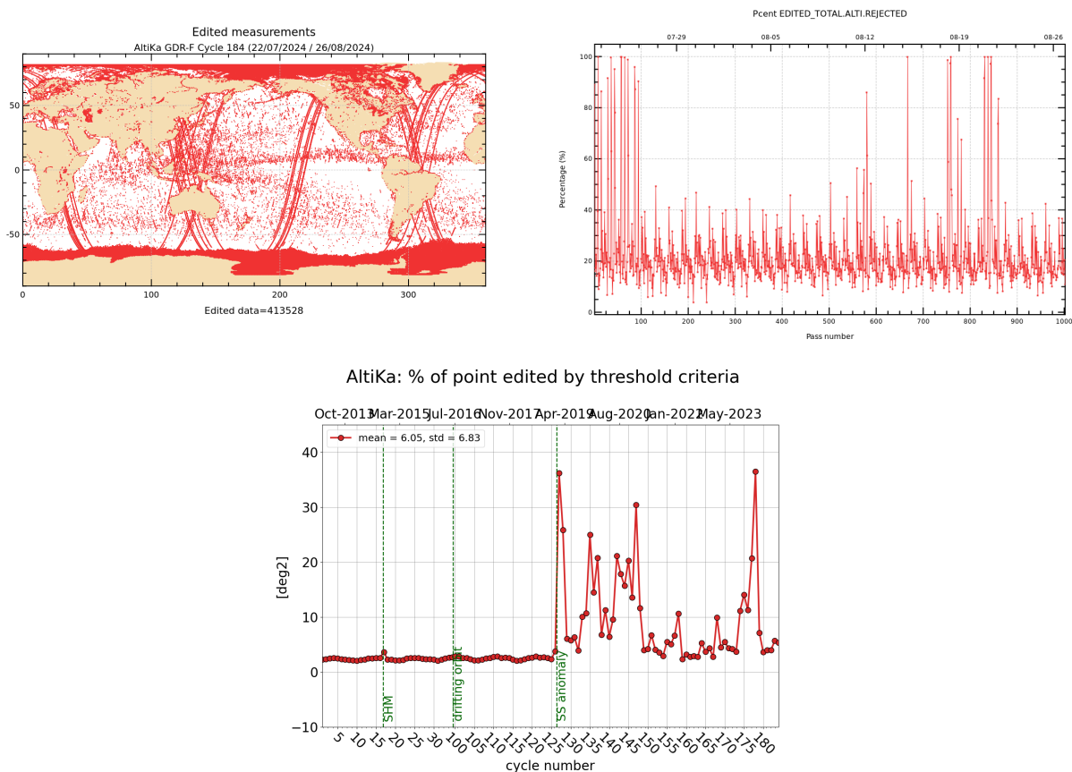
Figure 2: Rejected measurements on thresholds criteria : Cycle 184, map and monitoring of % of rejected measurements per track (top), whole time serie / % of rejected measurements per cycle (bottom).
