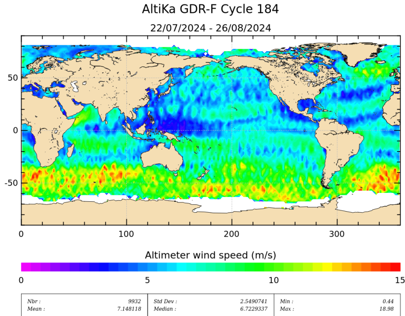
Figure 9: Altimeter wind speed for cycle 184.
