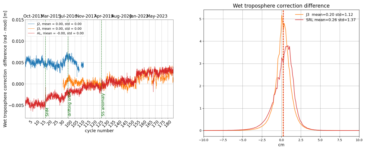
Figure 12: Daily monitoring of wet troposphere differences (Radiometer-ECMWF model) for Saral/AltiKa Jason-2 and Jason-3 (left) and histogram on the right (limited to 66° latitude) for cycle 184 .
