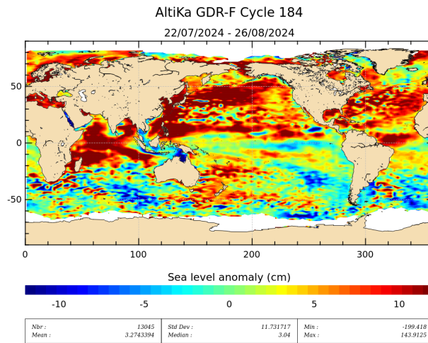
Figure 19: Sea level anomaly relative to MSS for cycle 184.
