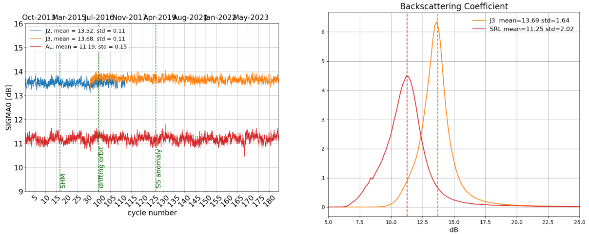
Figure 7: Daily monitoring of backscattering coefficient for Saral/AltiKa, Jason-2 and Jason-3 on the left and histogram for cycle 184 on the right (limited to 66° latitude).
