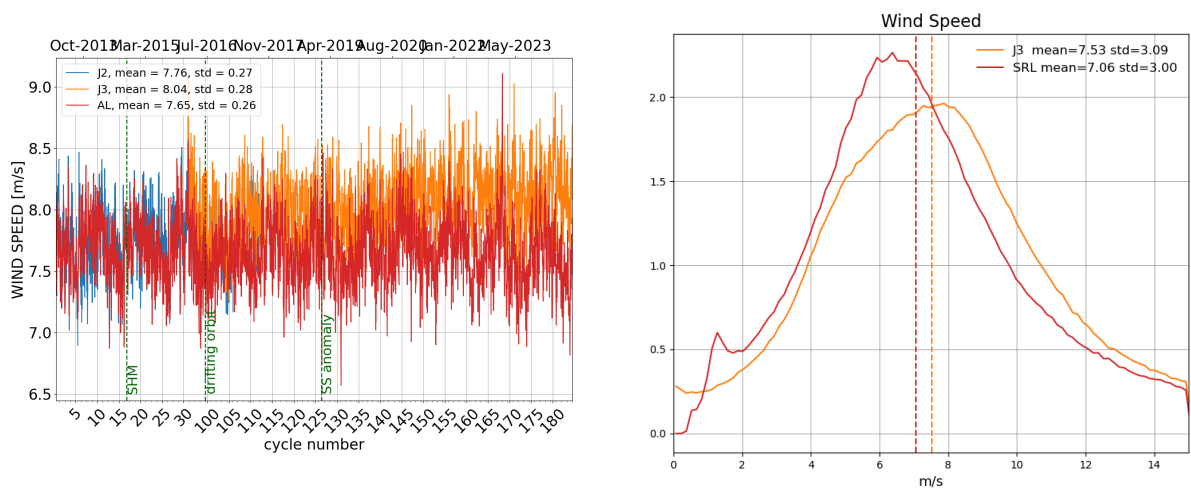
Figure 10: Daily monitoring of altimeter wind speed for Saral/AltiKa, Jason-2 and Jason-3 on the left and histogram for cycle 184 on the right (limited to 66° latitude).
