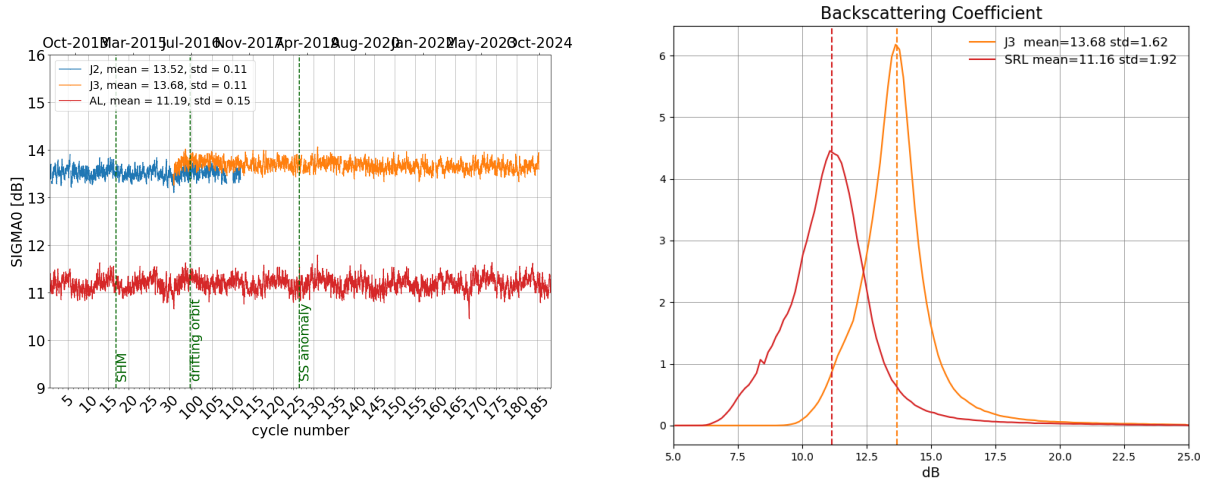
Figure 7: Daily monitoring of backscattering coefficient for Saral/AltiKa, Jason-2 and Jason-3 on the left and histogram for cycle 185 on the right (limited to 66° latitude).
