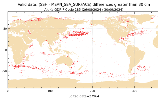
Figure 20: SLA higher than 30 cm for cycle 185.
