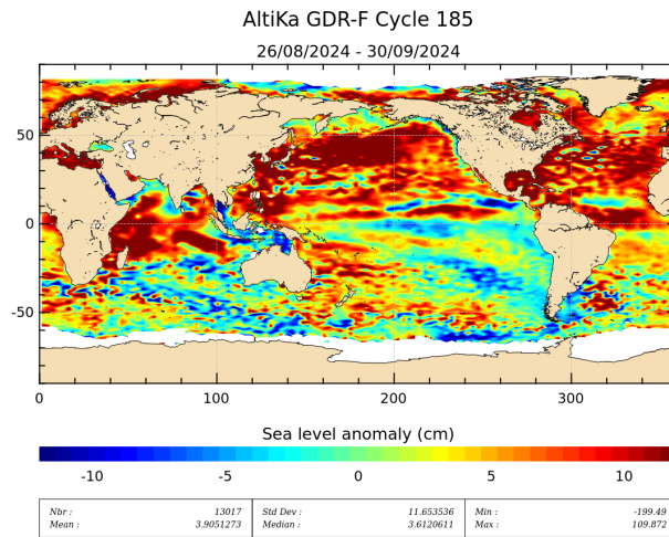
Figure 19: Sea level anomaly relative to MSS for cycle 185.
