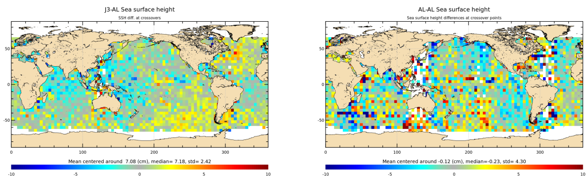
Figure 14: Mean of multi-mission SSH and mono-mission SSH differences at crossovers for cycle 185.
