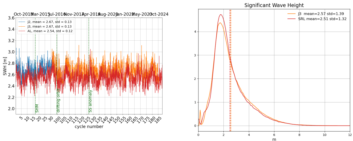
Figure 6: Daily monitoring of significant wave height for AltiKa (Ka-band) Jason-2 and Jason-3 (Ku-band) on the left and histogram for cycle 185 on the right (limited to 66^\circ latitude).
