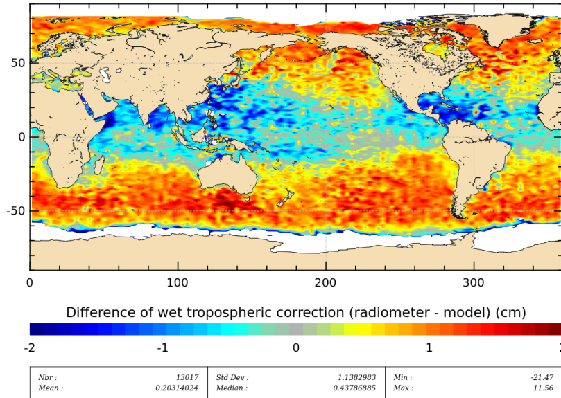
Figure 11: Mean of wet troposphere correction difference (Radiometer-ECMWF model) for cycle 185.
