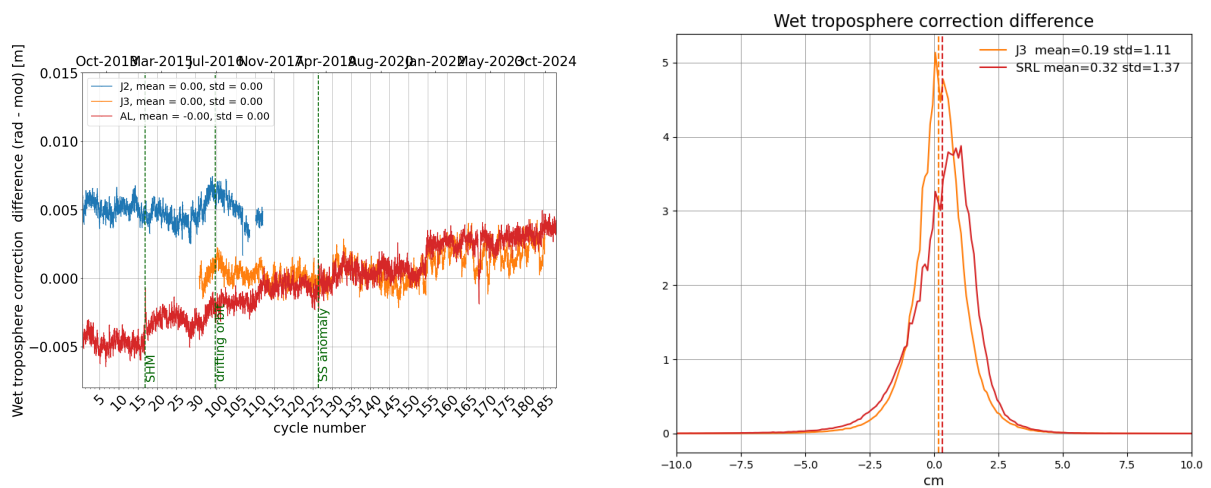
Figure 12: Daily monitoring of wet troposphere differences (Radiometer-ECMWF model) for Saral/AltiKa Jason-2 and Jason-3 (left) and histogram on the right (limited to 66° latitude) for cycle 185 .
