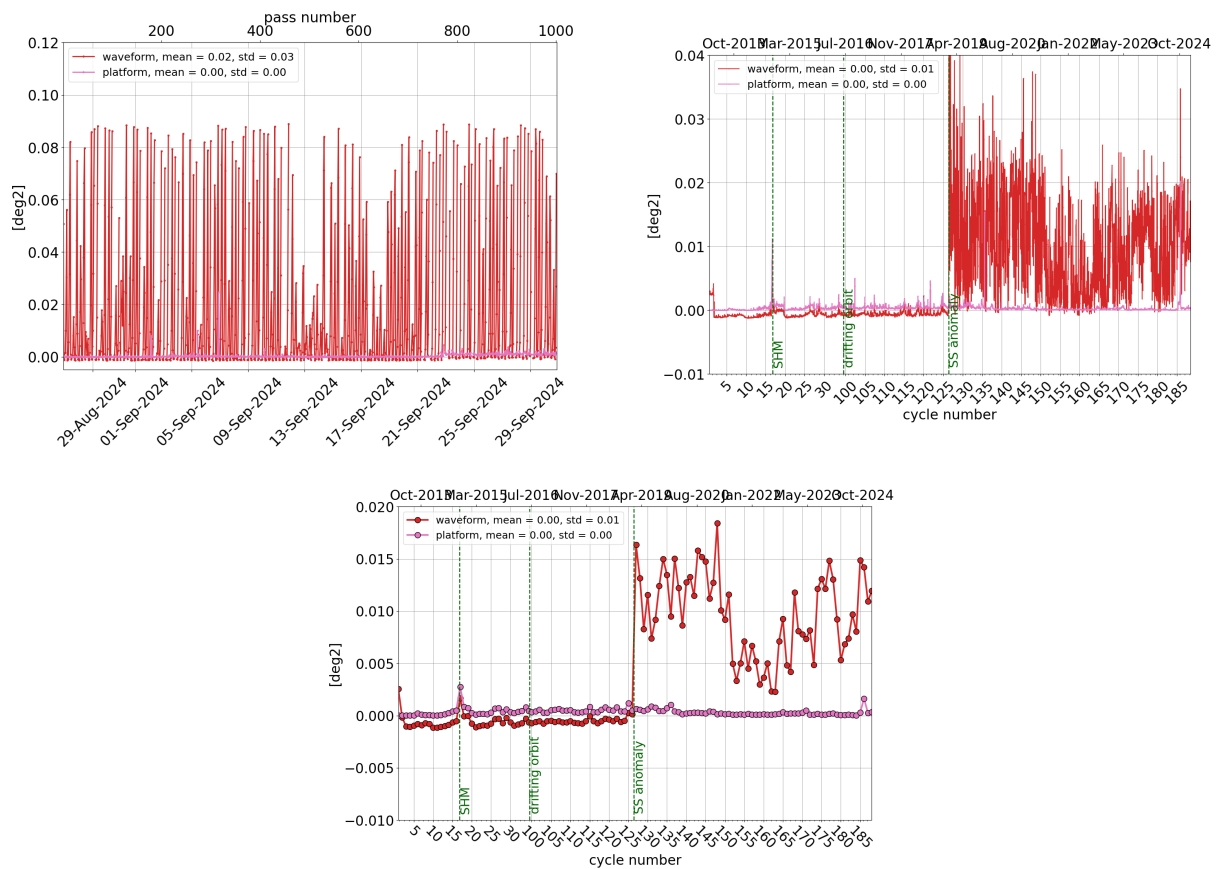
Figure 13: Monitoring per pass for cycle 185 (left), daily monitoring(right) and cyclic monitoring (bottom) of SARAL/AltiKa's mispointing angle: comparison between the one derived from waveform retracking and the one measured by platform startrackers.
