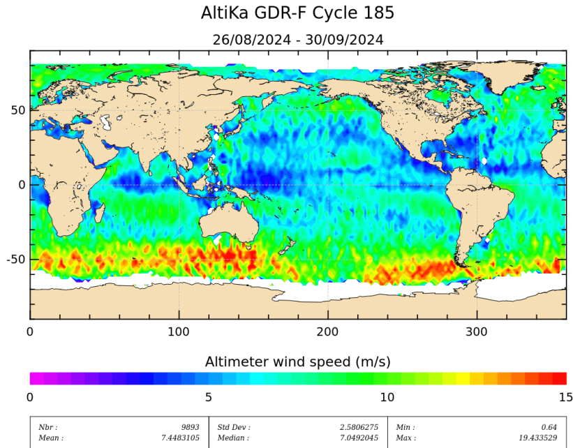
Figure 9: Altimeter wind speed for cycle 185.
