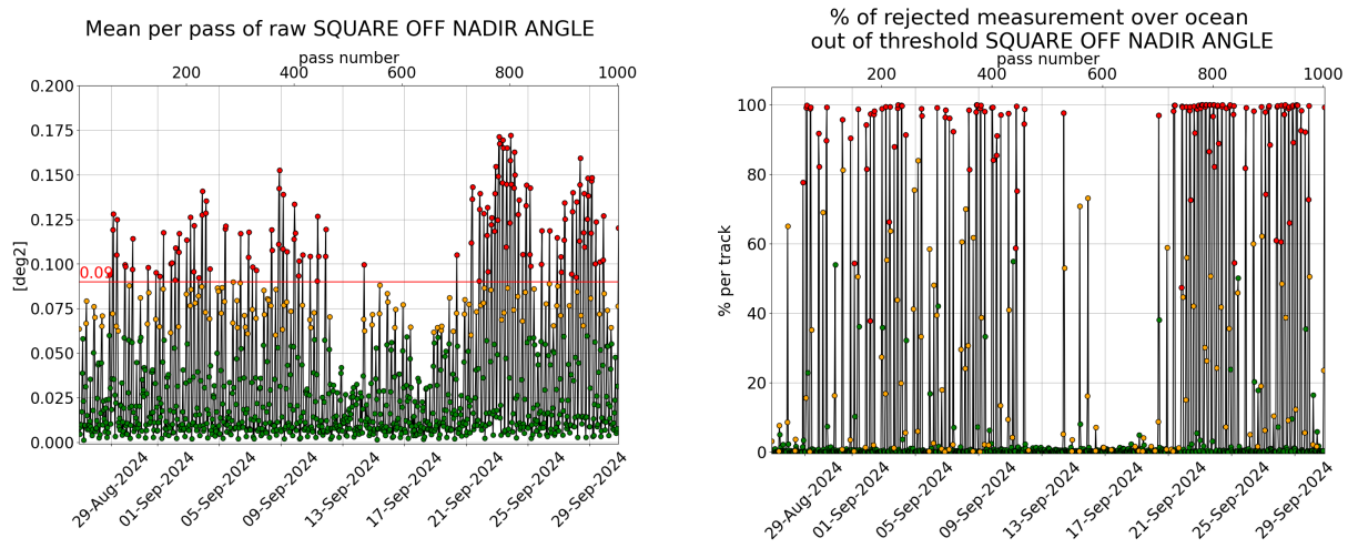
Figure 3: [left] Mispointing cycle 185, [right] Percentage of rejected measurement by threshold on square off-nadir angle.
