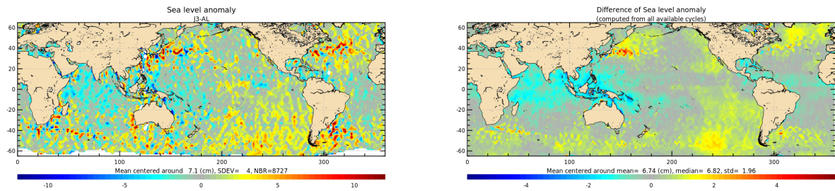
Figure 21: Jason-3 – Saral/AltiKa SLA differences for cycle 185 (left) and averaged over the whole Saral/AltiKa period (right).
