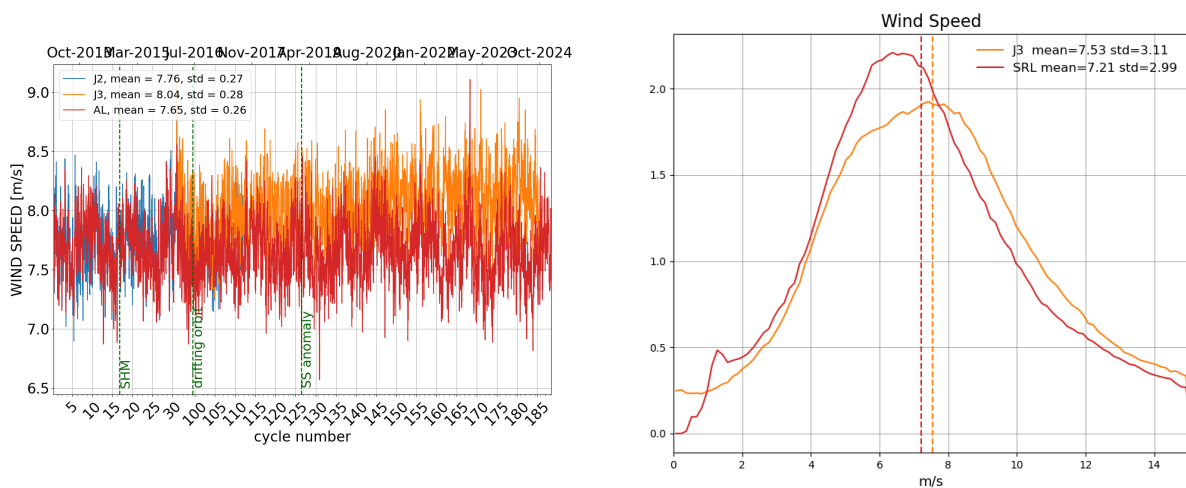
Figure 10: Daily monitoring of altimeter wind speed for Saral/AltiKa, Jason-2 and Jason-3 on the left and histogram for cycle 185 on the right (limited to 66° latitude).
