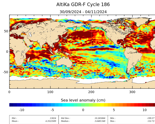
Figure 19: Sea level anomaly relative to MSS for cycle 186.
