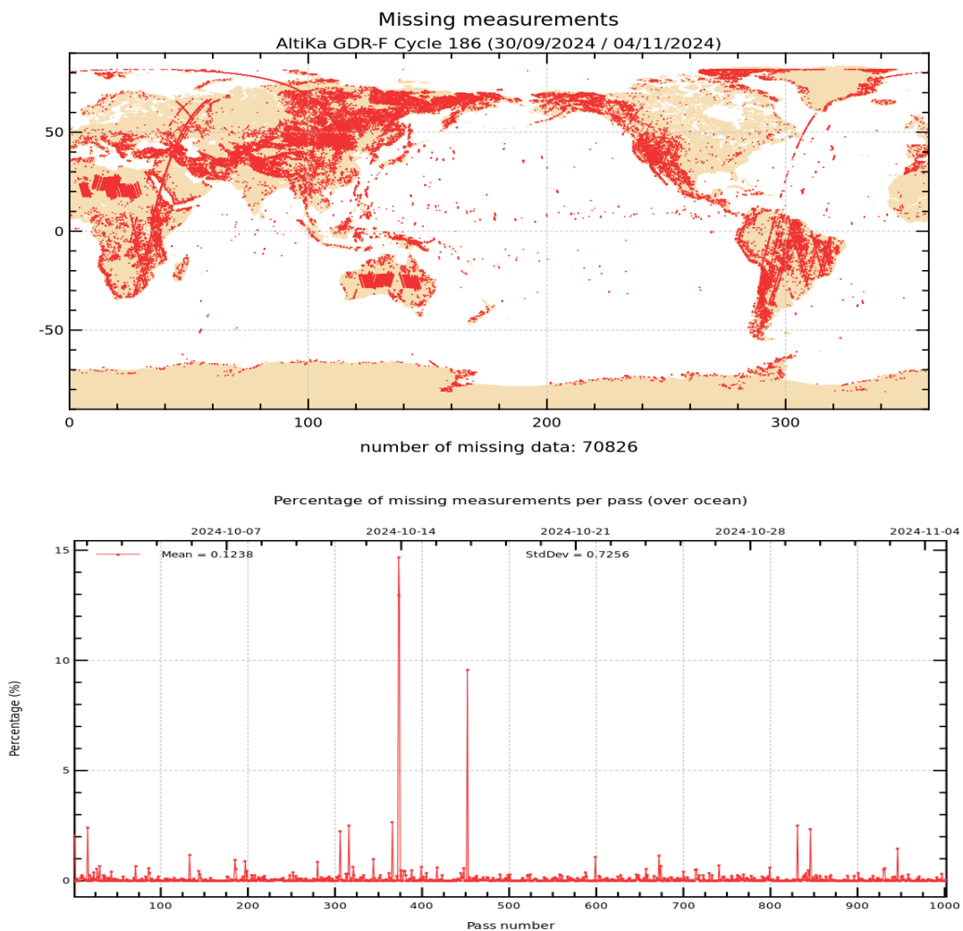
Figure 1: Map of missing measurements for cycle 186 on top. Monitoring of percentage of missing ocean measurements per pass on bottom.
