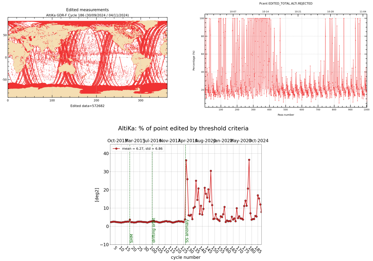
Figure 2: Rejected measurements on thresholds criteria : Cycle 186, map and monitoring of % of rejected measurements per track (top), whole time serie / % of rejected measurements per cycle (bottom).
