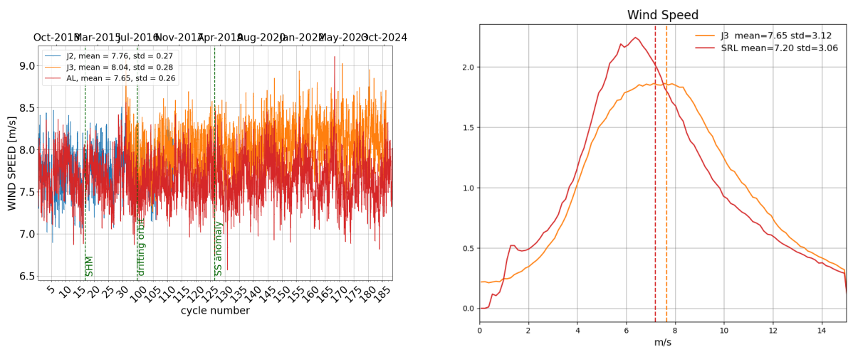
Figure 10: Daily monitoring of altimeter wind speed for Saral/AltiKa, Jason-2 and Jason-3 on the left and histogram for cycle 186 on the right (limited to 66° latitude).
