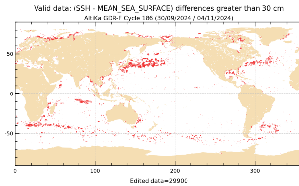
Figure 20: SLA higher than 30 cm for cycle 186.
