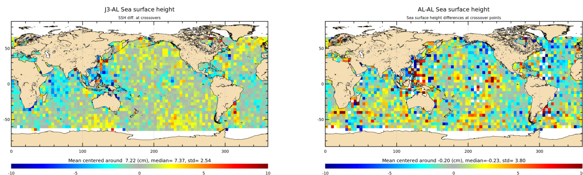
Figure 14: Mean of multi-mission SSH and mono-mission SSH differences at crossovers for cycle 186.
