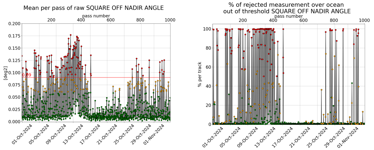
Figure 3: [left] Mispointing cycle 186, [right] Percentage of rejected measurement by threshold on square off-nadir angle.
