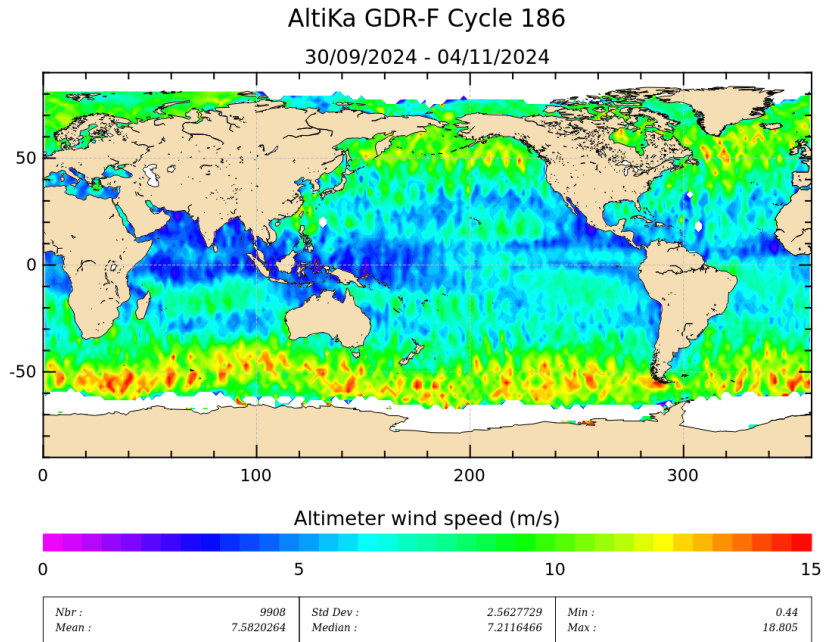
Figure 9: Altimeter wind speed for cycle 186.
