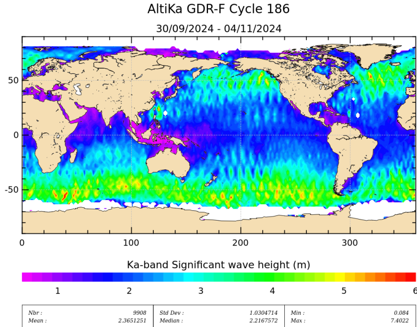
Figure 5: Significant wave height for cycle 186.
