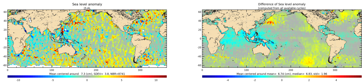
Figure 21: Jason-3 – Saral/AltiKa SLA differences for cycle 186 (left) and averaged over the whole Saral/AltiKa period (right).
