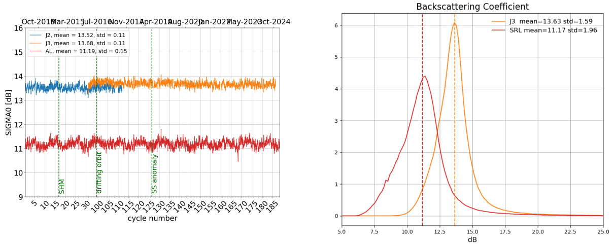
Figure 7: Daily monitoring of backscattering coefficient for Saral/AltiKa, Jason-2 and Jason-3 on the left and histogram for cycle 186 on the right (limited to 66° latitude).
