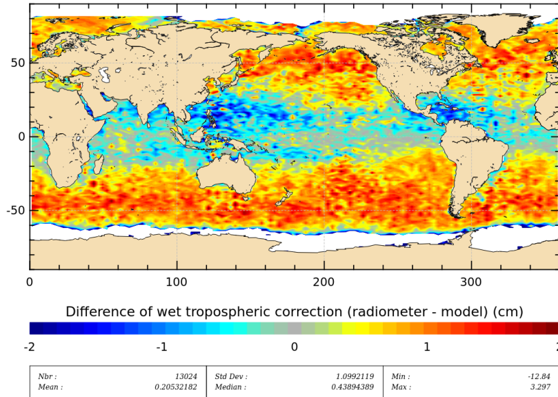
Figure 11: Mean of wet troposphere correction difference (Radiometer-ECMWF model) for cycle 186.
