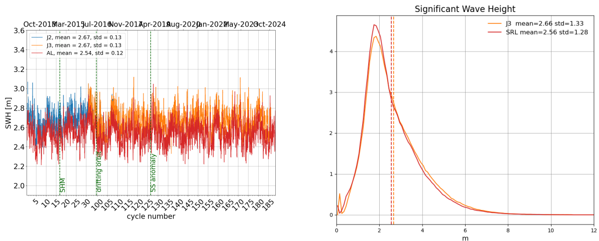
Figure 6: Daily monitoring of significant wave height for AltiKa (Ka-band) Jason-2 and Jason-3 (Ku-band) on the left and histogram for cycle 186 on the right (limited to 66^\circ latitude).
