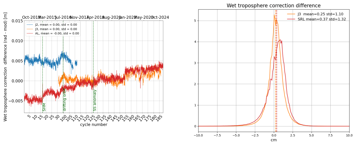
Figure 12: Daily monitoring of wet troposphere differences (Radiometer-ECMWF model) for Saral/AltiKa Jason-2 and Jason-3 (left) and histogram on the right (limited to 66° latitude) for cycle 186 .
