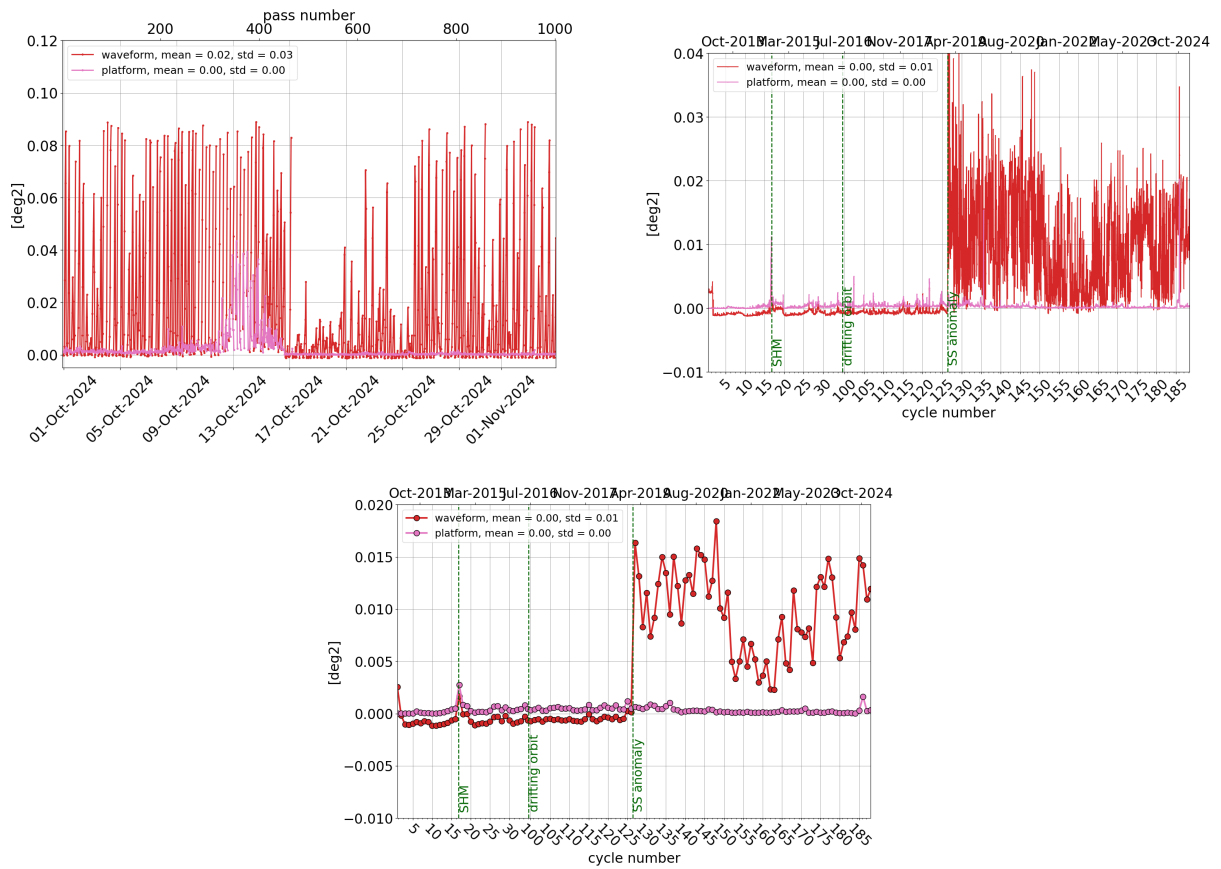
Figure 13: Monitoring per pass for cycle 186 (left), daily monitoring(right) and cyclic monitoring (bottom) of SARAL/AltiKa's mispointing angle: comparison between the one derived from waveform retracking and the one measured by platform startrackers.
