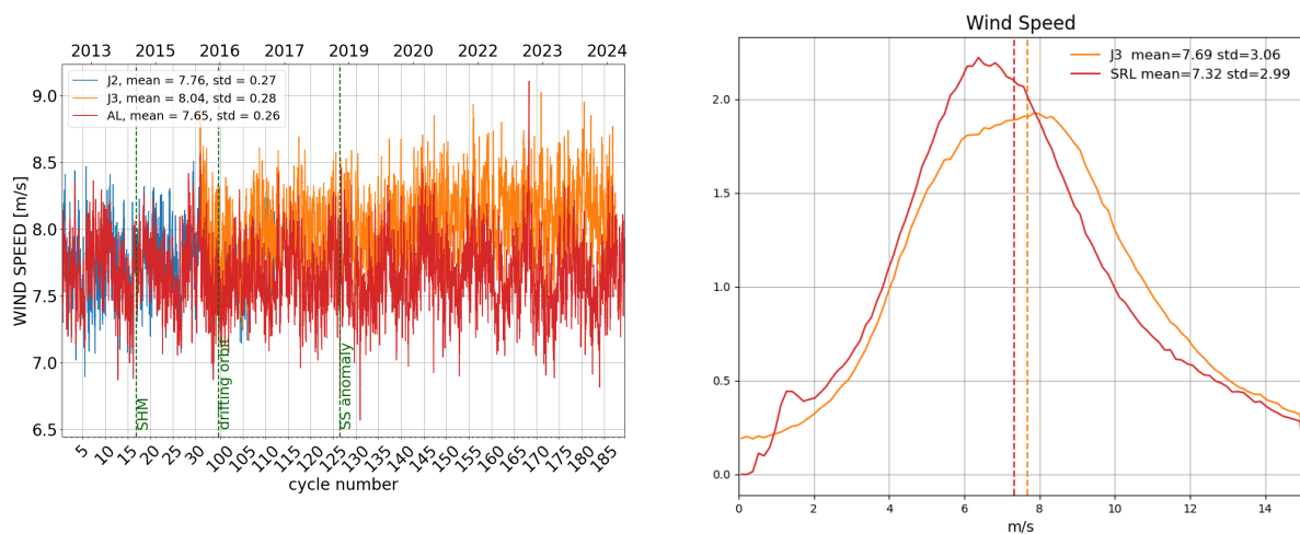
Figure 10: Daily monitoring of altimeter wind speed for Saral/AltiKa, Jason-2 and Jason-3 on the left and histogram for cycle 187 on the right (limited to 66° latitude).
