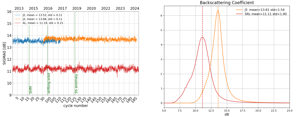
Figure 7: Daily monitoring of backscattering coefficient for Saral/AltiKa, Jason-2 and Jason-3 on the left and histogram for cycle 187 on the right (limited to 66° latitude).
