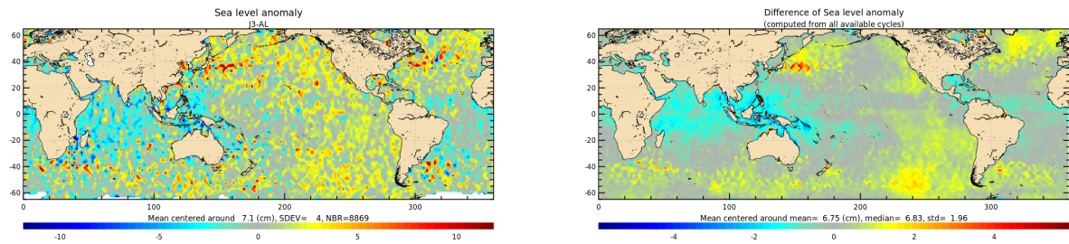
Figure 21: Jason-3 — Saral/AltiKa SLA differences for cycle 187 (left) and averaged over the whole Saral/AltiKa period (right).
