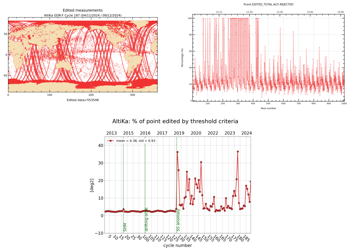
Figure 2: Rejected measurements on thresholds criteria : Cycle 187, map and monitoring of % of rejected measurements per track (top), whole time serie / % of rejected measurements per cycle (bottom).
