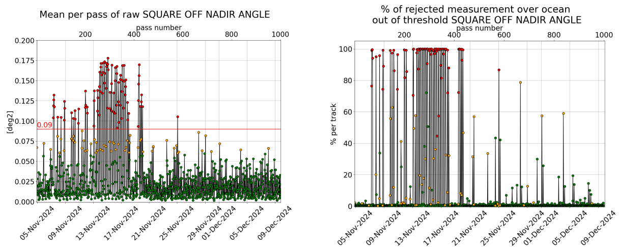
Figure 3: [left] Mispointing cycle 187, [right] Percentage of rejected measurement by threshold on square off-nadir angle.
