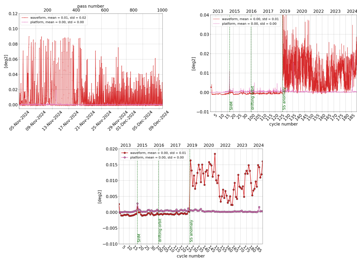
Figure 13: Monitoring per pass for cycle 187 (left), daily monitoring(right) and cyclic monitoring (bottom) of SARAL/AltiKa's mispointing angle: comparison between the one derived from waveform retracking and the one measured by platform startrackers.
