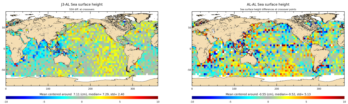
Figure 14: Mean of multi-mission SSH and mono-mission SSH differences at crossovers for cycle 187.
