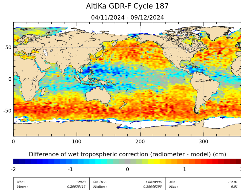
Figure 11: Mean of wet troposphere correction difference (Radiometer-ECMWF model)for cycle 187.
