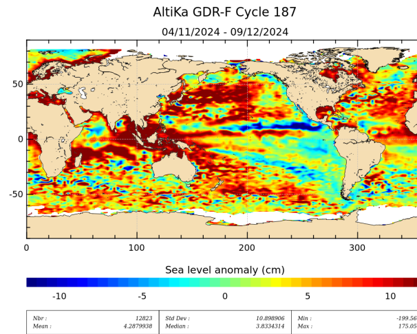
Figure 19: Sea level anomaly relative to MSS for cycle 187.
