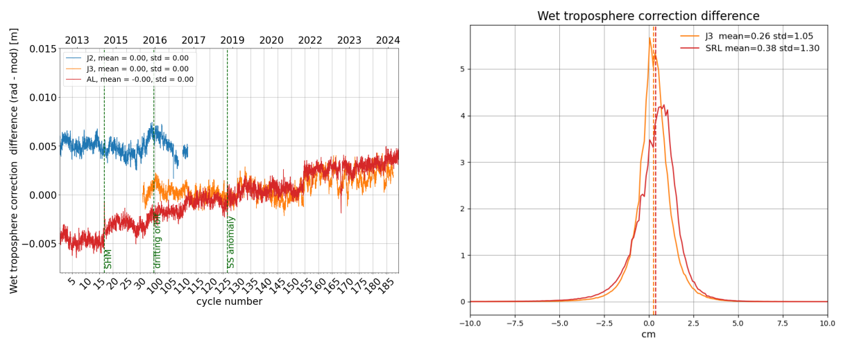
Figure 12: Daily monitoring of wet troposphere differences (Radiometer-ECMWF model) for Saral/AltiKa Jason-2 and Jason-3 (left) and histogram on the right (limited to 66° latitude) for cycle 187 .
