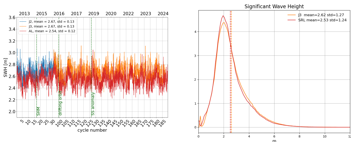
Figure 6: Daily monitoring of significant wave height for AltiKa (Ka-band) Jason-2 and Jason-3 (Ku-band) on the left and histogram for cycle 187 on the right (limited to 66^\circ latitude).
