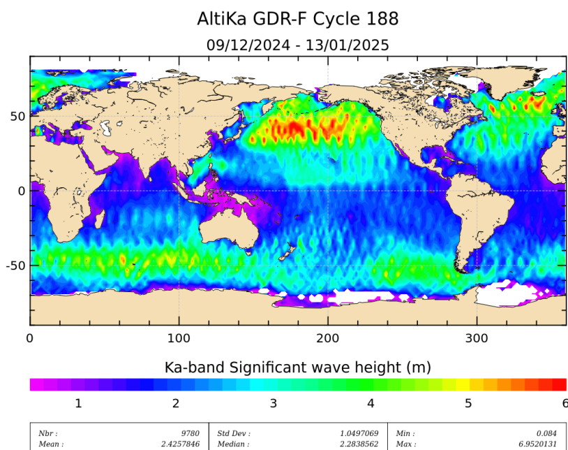
Figure 5: Significant wave height for cycle 188.
