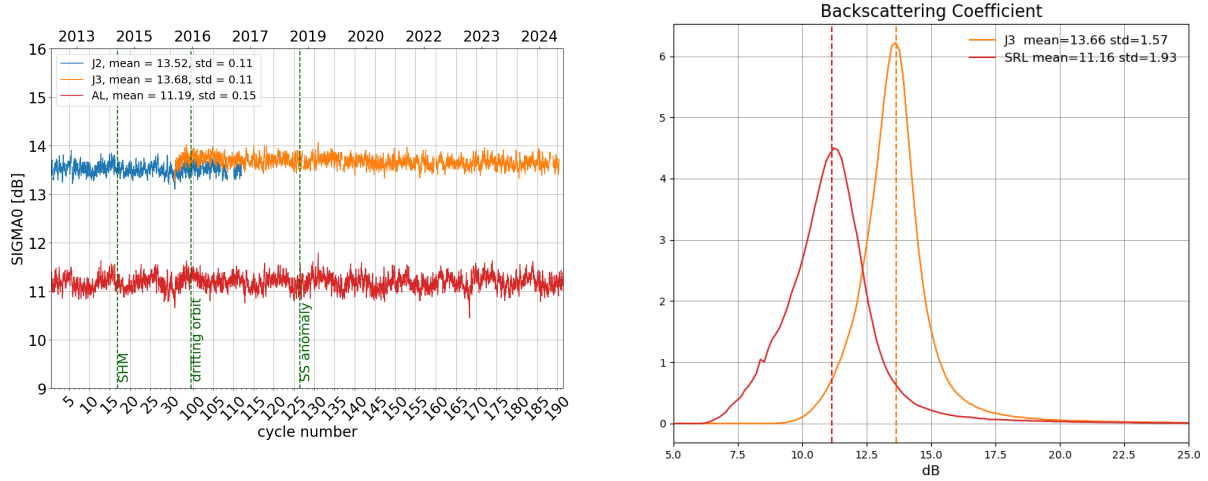
Figure 7: Daily monitoring of backscattering coefficient for Saral/AltiKa, Jason-2 and Jason-3 on the left and histogram for cycle 188 on the right (limited to 66° latitude).
