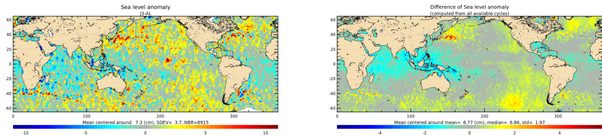
Figure 21: Jason-3 — Saral/AltiKa SLA differences for cycle 188 (left) and averaged over the whole Saral/AltiKa period (right).
