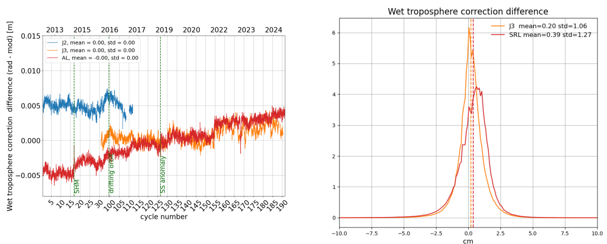
Figure 12: Daily monitoring of wet troposphere differences (Radiometer-ECMWF model) for Saral/AltiKa Jason-2 and Jason-3 (left) and histogram on the right (limited to 66° latitude) for cycle 188 .
