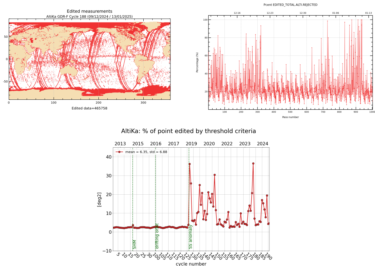
Figure 2: Rejected measurements on thresholds criteria : Cycle 188, map and monitoring of % of rejected measurements per track (top), whole time serie / % of rejected measurements per cycle (bottom).
