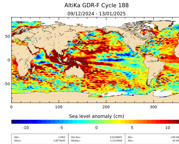
Figure 19: Sea level anomaly relative to MSS for cycle 188.
