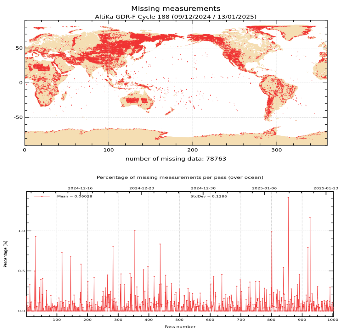
Figure 1: Map of missing measurements for cycle 188 on top. Monitoring of percentage of missing ocean measurements per pass on bottom.
