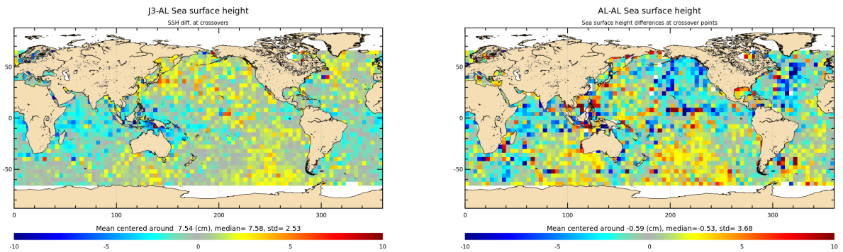
Figure 14: Mean of multi-mission SSH and mono-mission SSH differences at crossovers for cycle 188.
