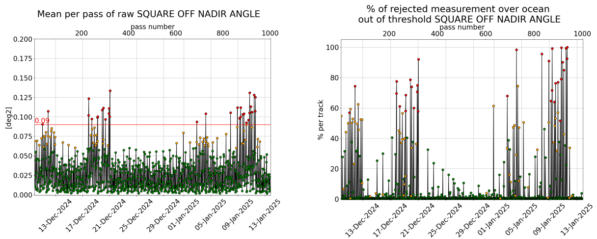
Figure 3: [left] Mispointing cycle 188, [right] Percentage of rejected measurement by threshold on square off-nadir angle.
