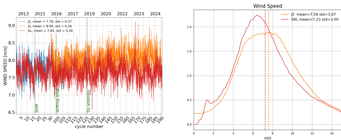
Figure 10: Daily monitoring of altimeter wind speed for Saral/AltiKa, Jason-2 and Jason-3 on the left and histogram for cycle 188 on the right (limited to 66° latitude).
