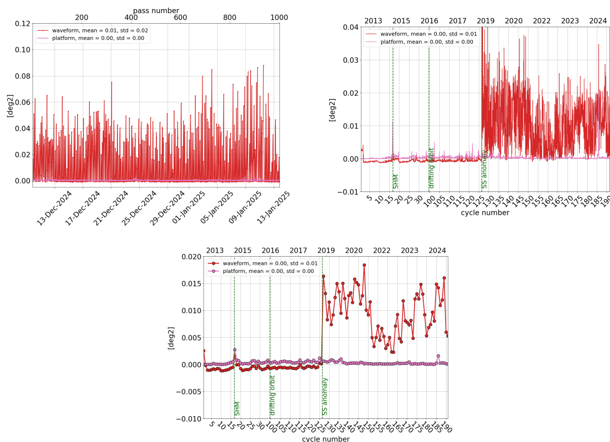
Figure 13: Monitoring per pass for cycle 188 (left), daily monitoring(right) and cyclic monitoring (bottom) of SARAL/AltiKa's mispointing angle: comparison between the one derived from waveform retracking and the one measured by platform startrackers.
