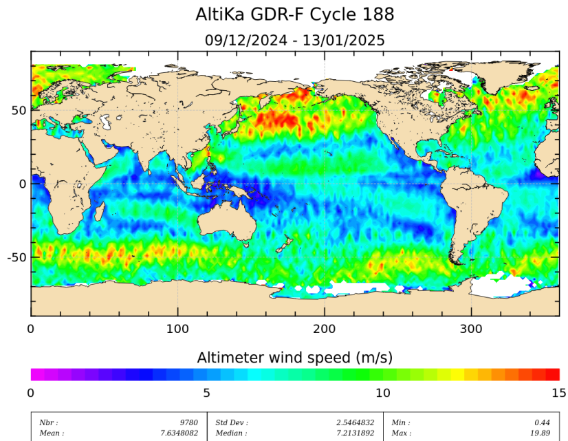
Figure 9: Altimeter wind speed for cycle 188.
