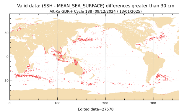
Figure 20: SLA higher than 30 cm for cycle 188.
