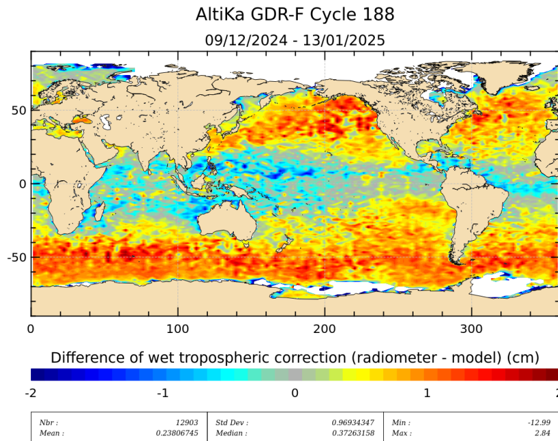
Figure 11: Mean of wet troposphere correction difference (Radiometer-ECMWF model)for cycle 188.
