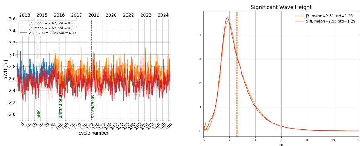
Figure 6: Daily monitoring of significant wave height for AltiKa (Ka-band) Jason-2 and Jason-3 (Ku-band) on the left and histogram for cycle 188 on the right (limited to 66^\circ latitude).
