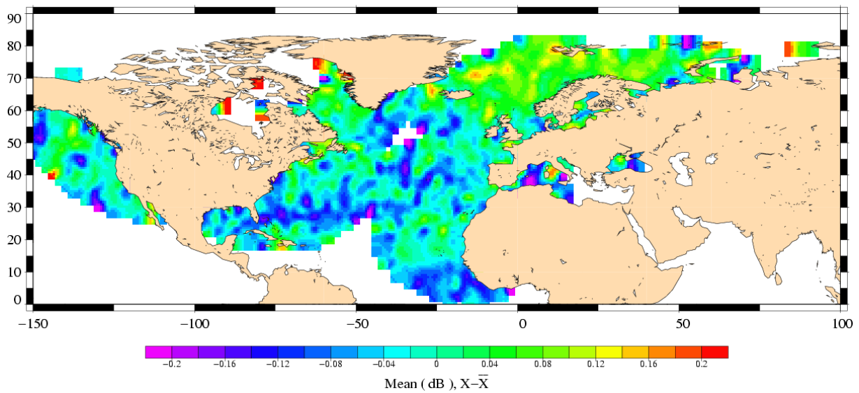
Sigma0 differences ERS-2 (Cycle 095) – Envisat (Cycle 027)
