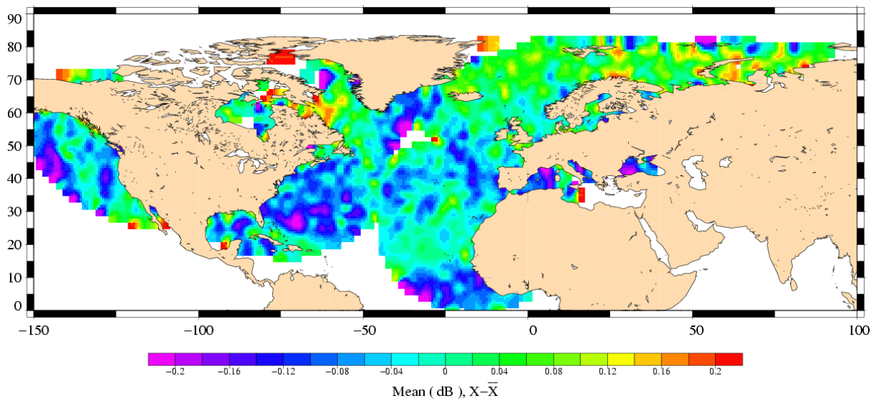
Sigma0 differences ERS-2 (Cycle 096) – Envisat (Cycle 028)
