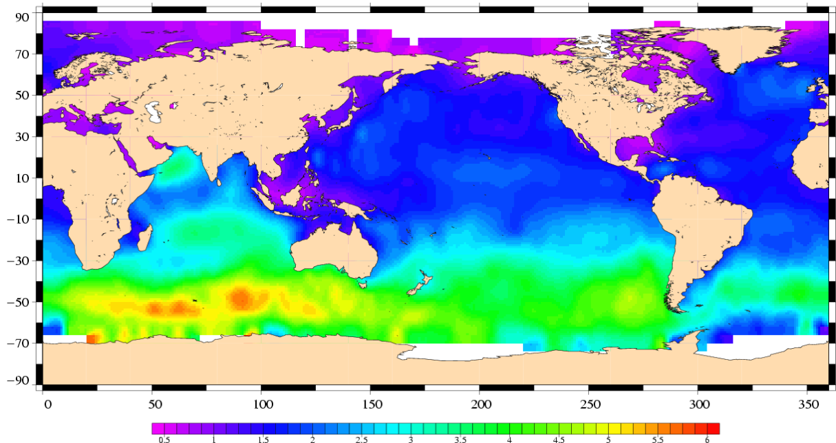
Significant Wave Height (m) Envisat Cycle 028 21/06/2004 – 26/07/2004
