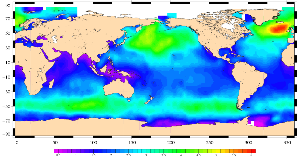
Significant Wave Height (m) Envisat Cycle 033 13/12/2004 – 17/01/2005
