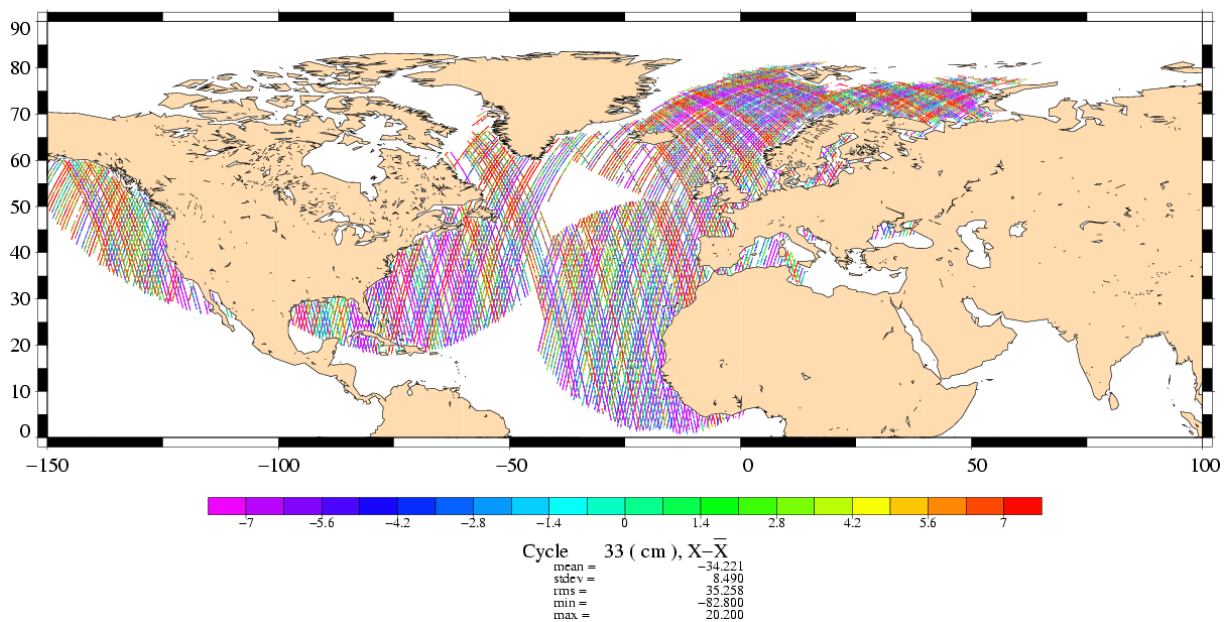
Corrected SLA (GIM iono, ECMWF (gaussian) wet tropo configuration) ERS-2 (Cycle 101) – Envisat (Cycle 033)
