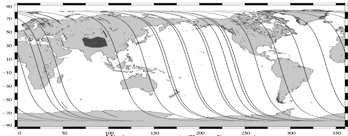
Missing measurements (Descending passes) Envisat Cycle 036 (28/03/2005 / 02/05/2005)
