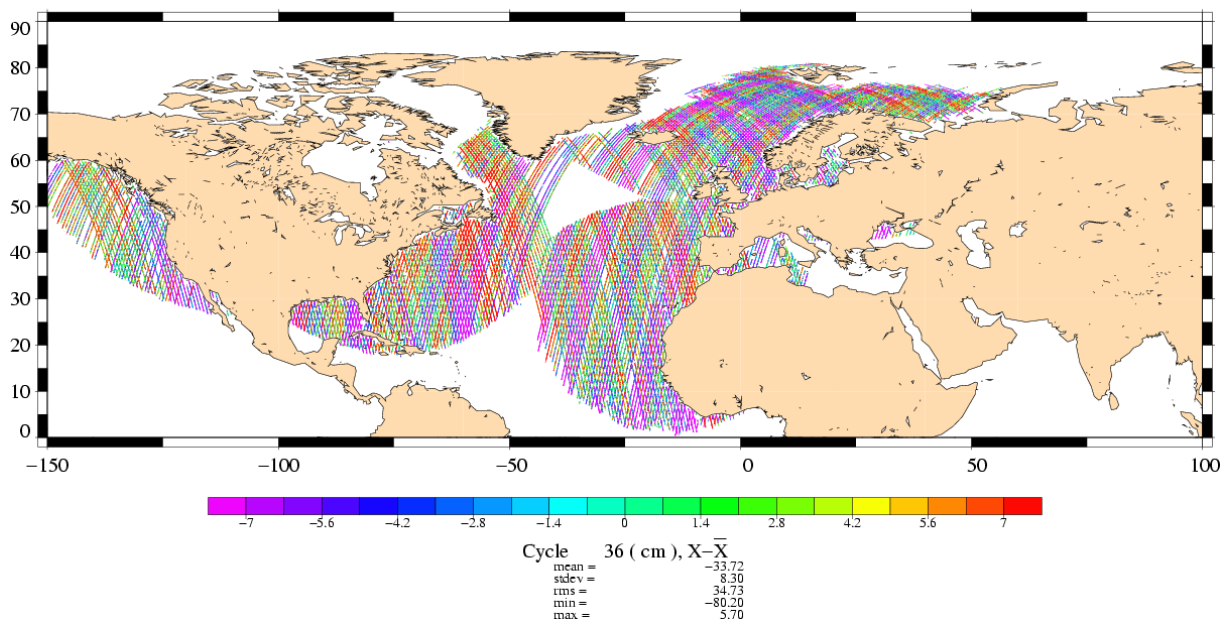
Corrected SLA (GIM iono, ECMWF (gaussian) wet tropo configuration) ERS-2 (Cycle 104) – Envisat (Cycle 036)
