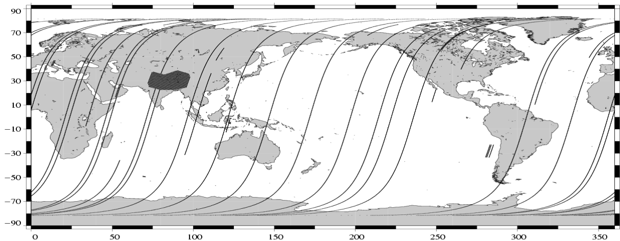
Missing measurements (Descending passes) Envisat Cycle 036 (28/03/2005 / 02/05/2005)
