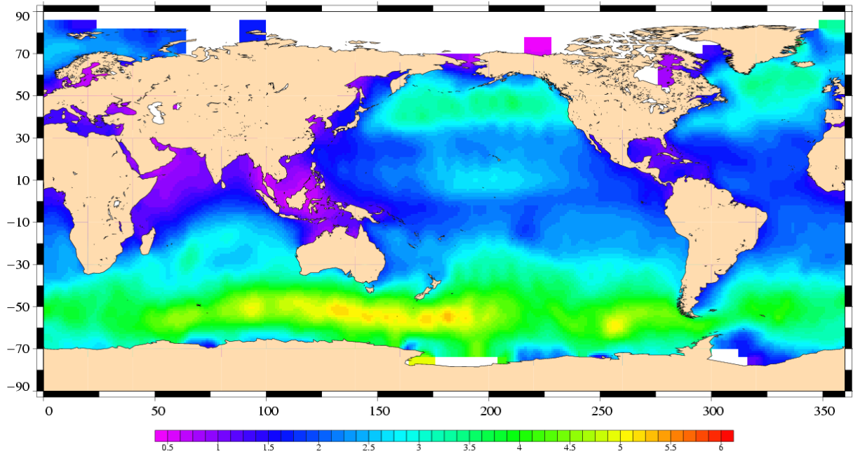
Significant Wave Height (m) Envisat Cycle 036 28/03/2005 – 02/05/2005
