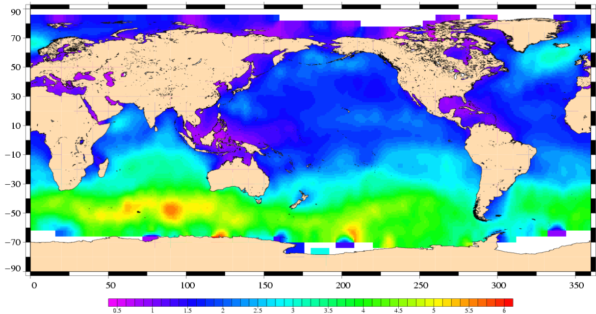
Significant Wave Height (m) Envisat Cycle 040 15/08/2005 – 19/09/2005
