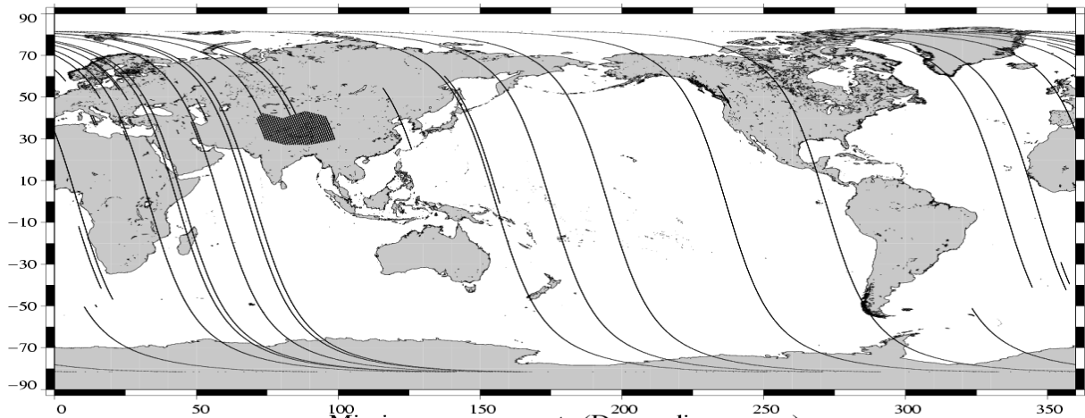
Missing measurements (Descending passes) Envisat Cycle 040 (15/08/2005 / 19/09/2005)
