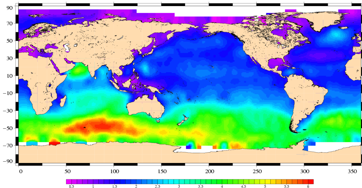
Significant Wave Height (m) Envisat Cycle 049 26/06/2006 – 31/07/2006
