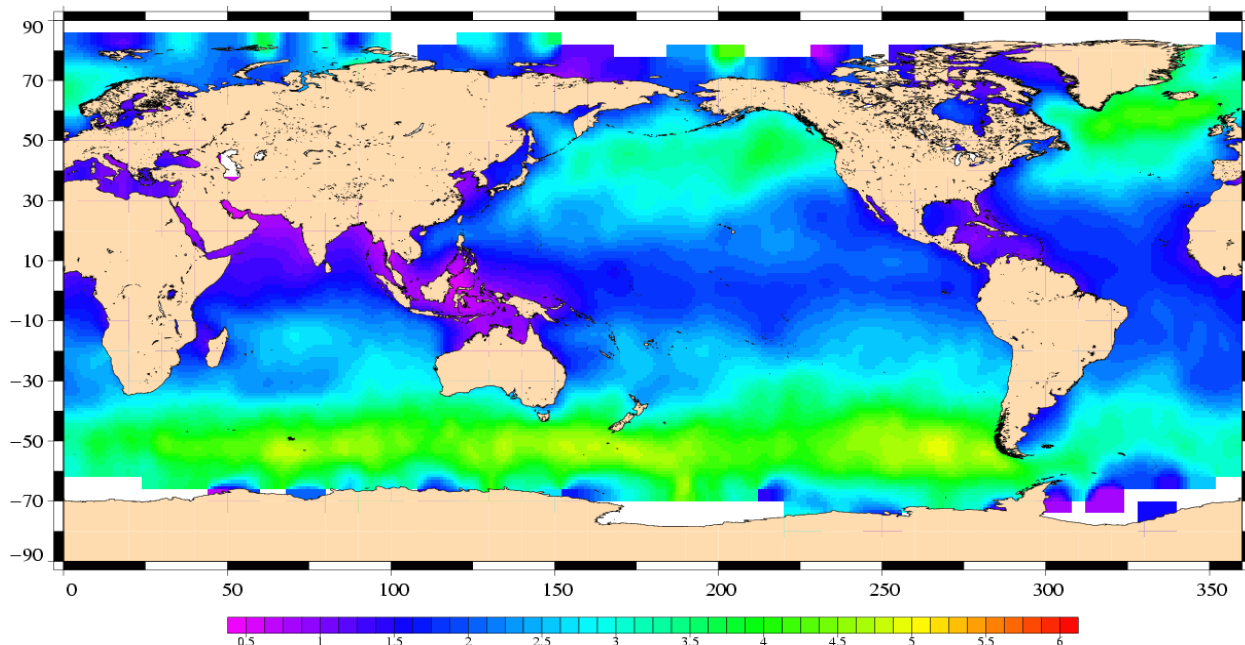
Significant Wave Height (m) Envisat Cycle 052 09/10/2006 – 13/11/2006
