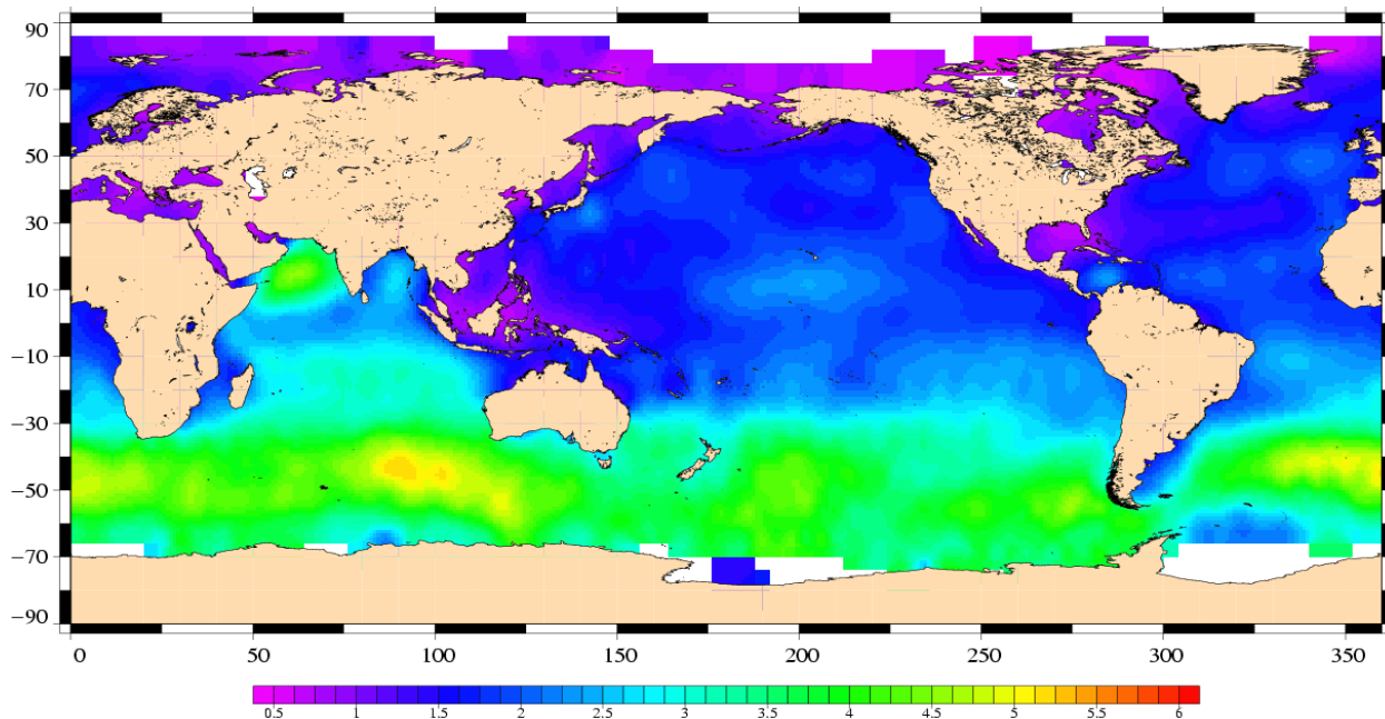
Significant Wave Height (m) Envisat Cycle 059 11/06/2007 – 16/07/2007
