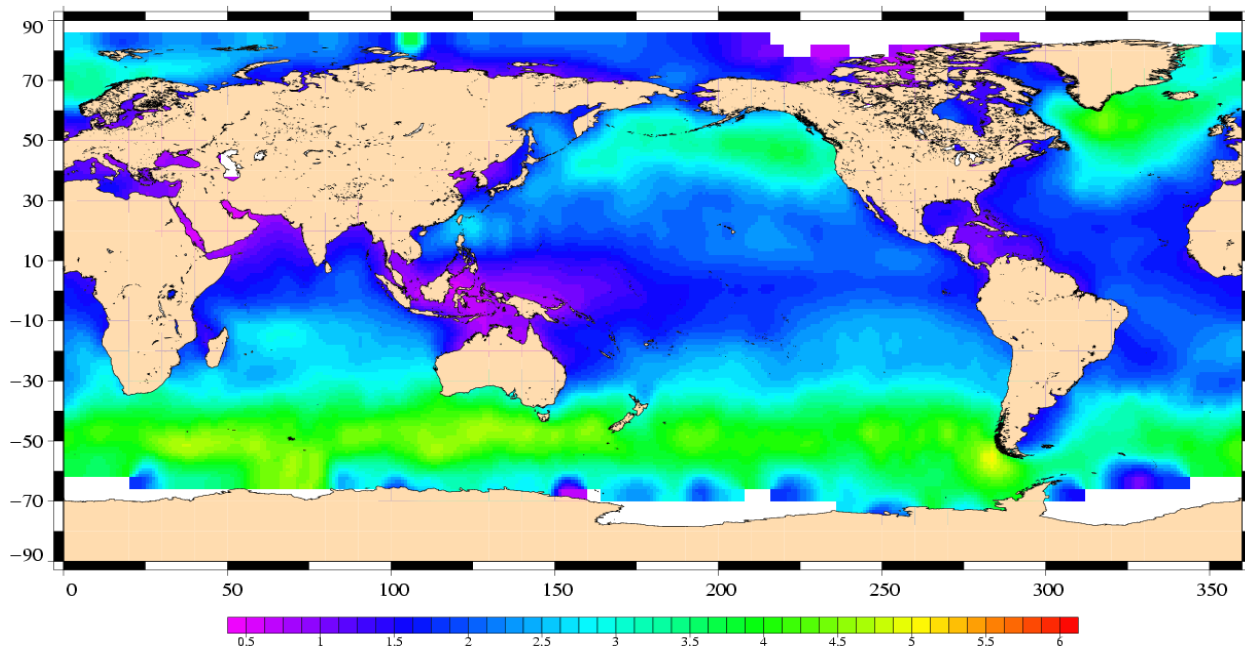
Significant Wave Height (m) Envisat Cycle 062 27/09/2007 – 29/10/2007
