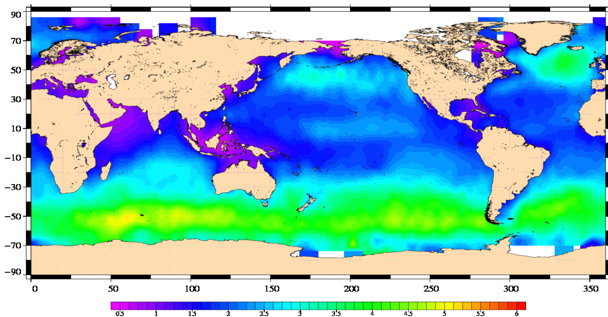
Significant Wave Height (m) Envisat Cycle 078 06/04/2009 – 11/05/2009
