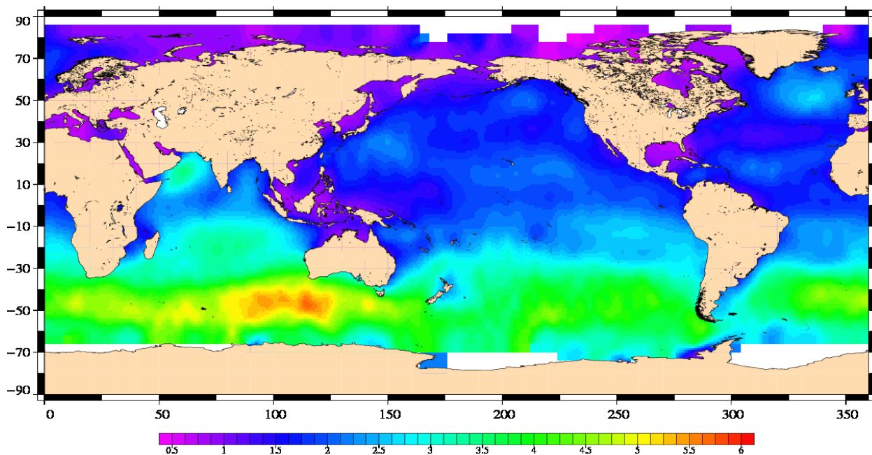
Significant Wave Height (m) Envisat Cycle 081 20/07/2009 – 24/08/2009
