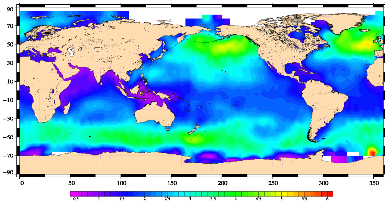
Significant Wave Height (m) Envisat Cycle 084 02/11/2009 – 07/12/2009
