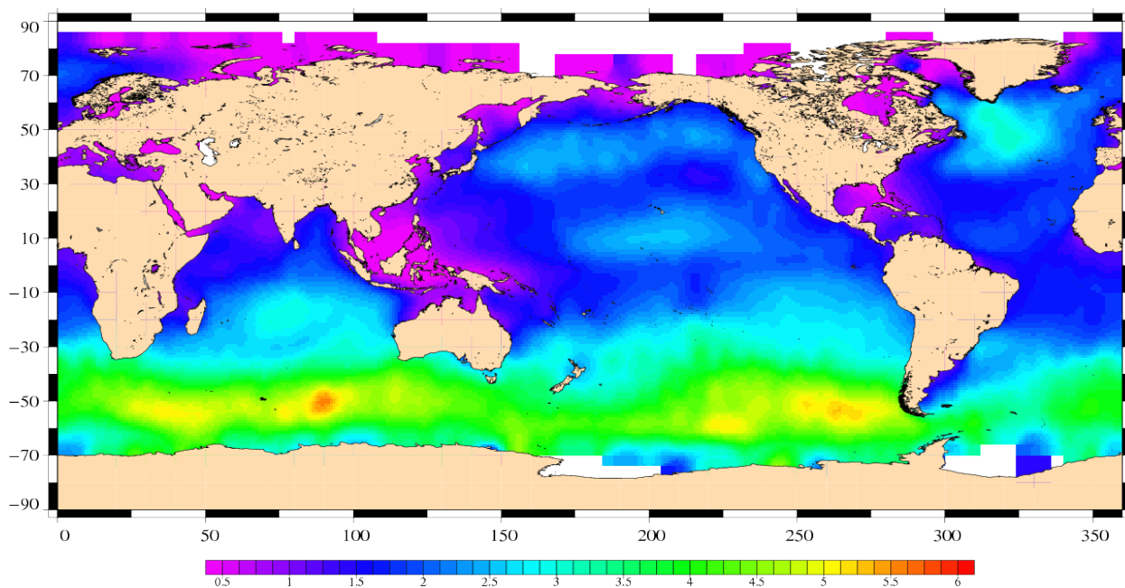
Significant Wave Height (m) Envisat Cycle 089 26/04/2010 – 31/05/2010
