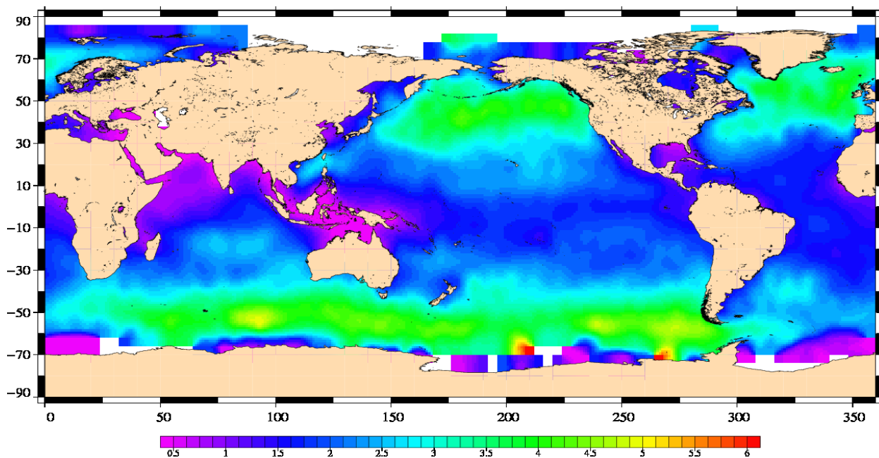
Significant Wave Height (m) Envisat Cycle 096 27/10/2010 – 26/11/2010
