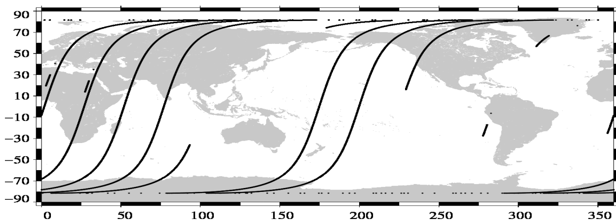
Missing measurements (Descending passes) Envisat Cycle 102 (25/04/2011 / 25/05/2011)
