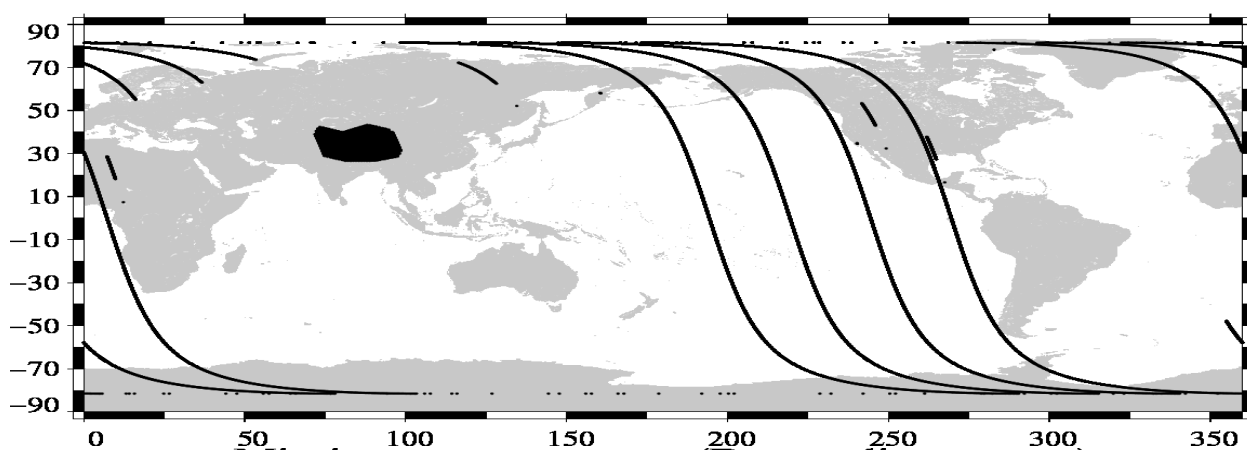
Missing measurements (Descending passes) Envisat Cycle 102 (25/04/2011 / 25/05/2011)
