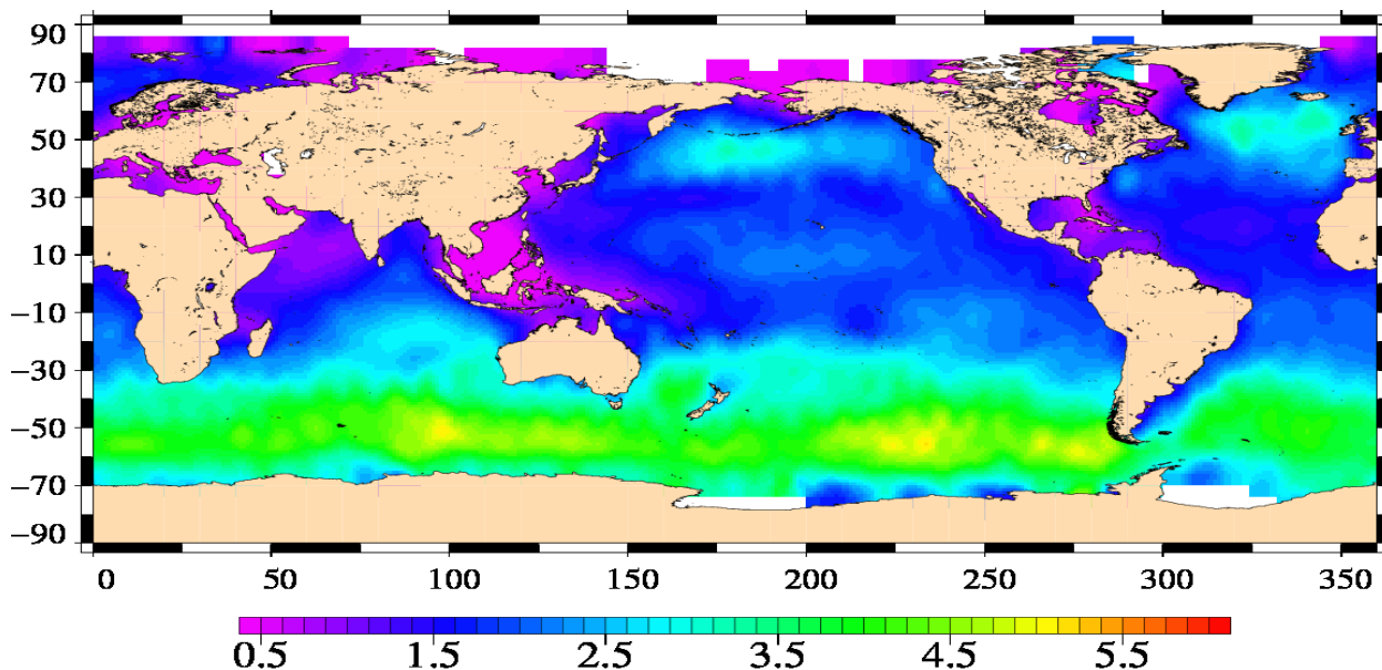
Significant Wave Height (m) Envisat Cycle 102 25/04/2011 – 25/05/2011
