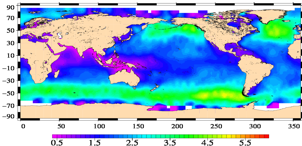
Significant Wave Height (m) Envisat Cycle 108 22/10/2011 – 21/11/2011
