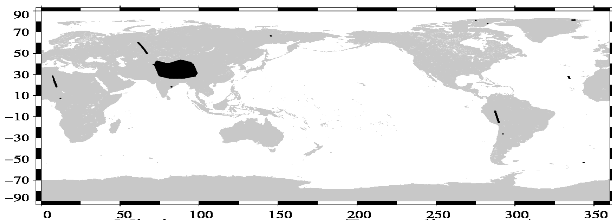
Missing measurements (Descending passes) Envisat Cycle 108 (22/10/2011 / 21/11/2011)
