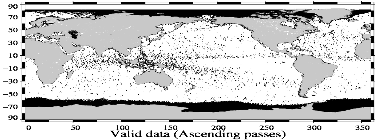
Valid data (Ascending passes) Envisat Cycle 108 (22/10/2011 / 21/11/2011)
