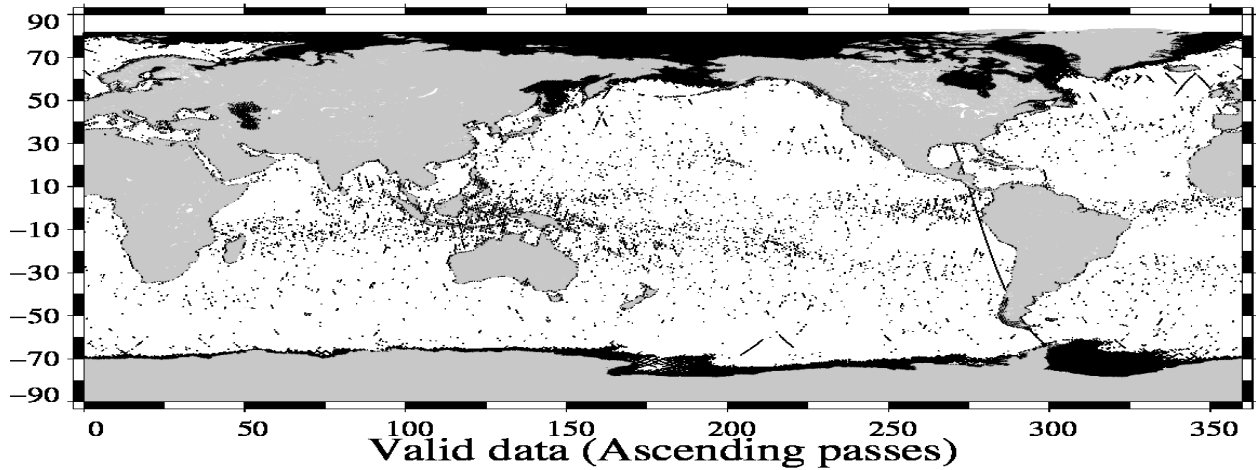
Valid data (Ascending passes) Envisat Cycle 112 (19/02/2012 / 20/03/2012)
