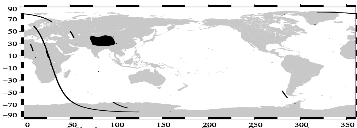
Missing measurements (Descending passes) Envisat Cycle 112 (19/02/2012 / 20/03/2012)
