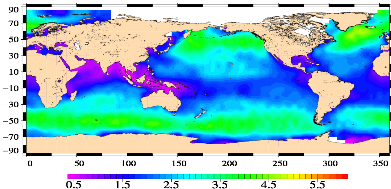
Significant Wave Height (m) Envisat Cycle 112 19/02/2012 – 20/03/2012
