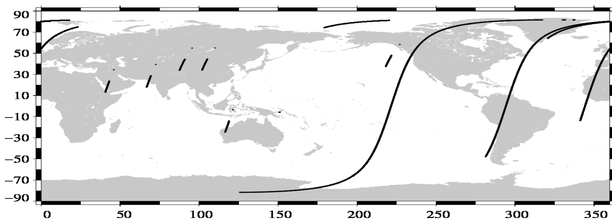
Missing measurements (Descending passes) Envisat Cycle 112 (19/02/2012 / 20/03/2012)
