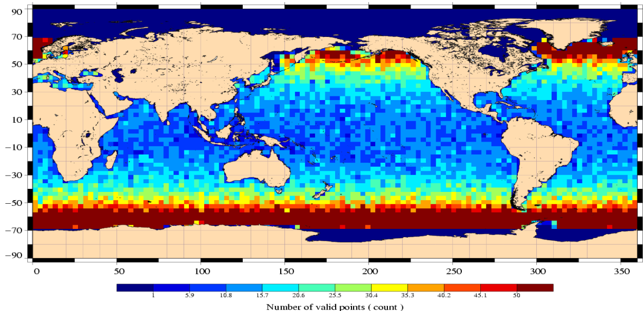
Number of Jason/Envisat 10 days cross-over points Cycle 045 (06/02/2006 – 13/03/2006)
