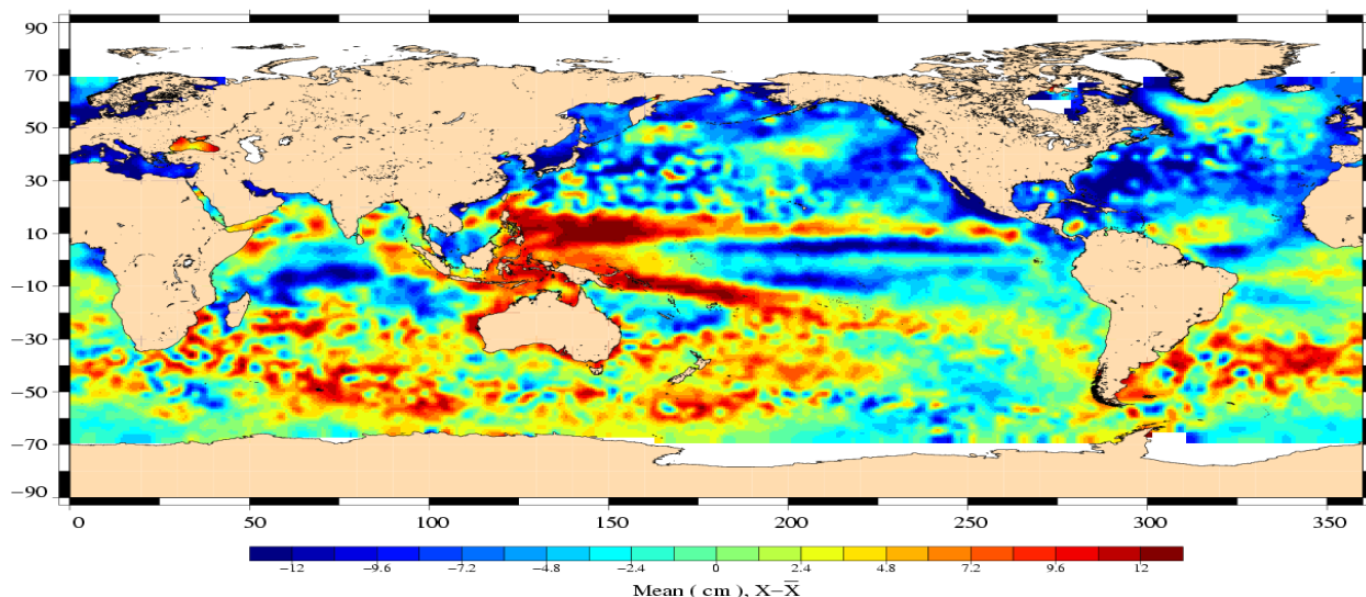
Variability relative to MSS (cm) Jason (17/04/2006 to 22/05/2006)
