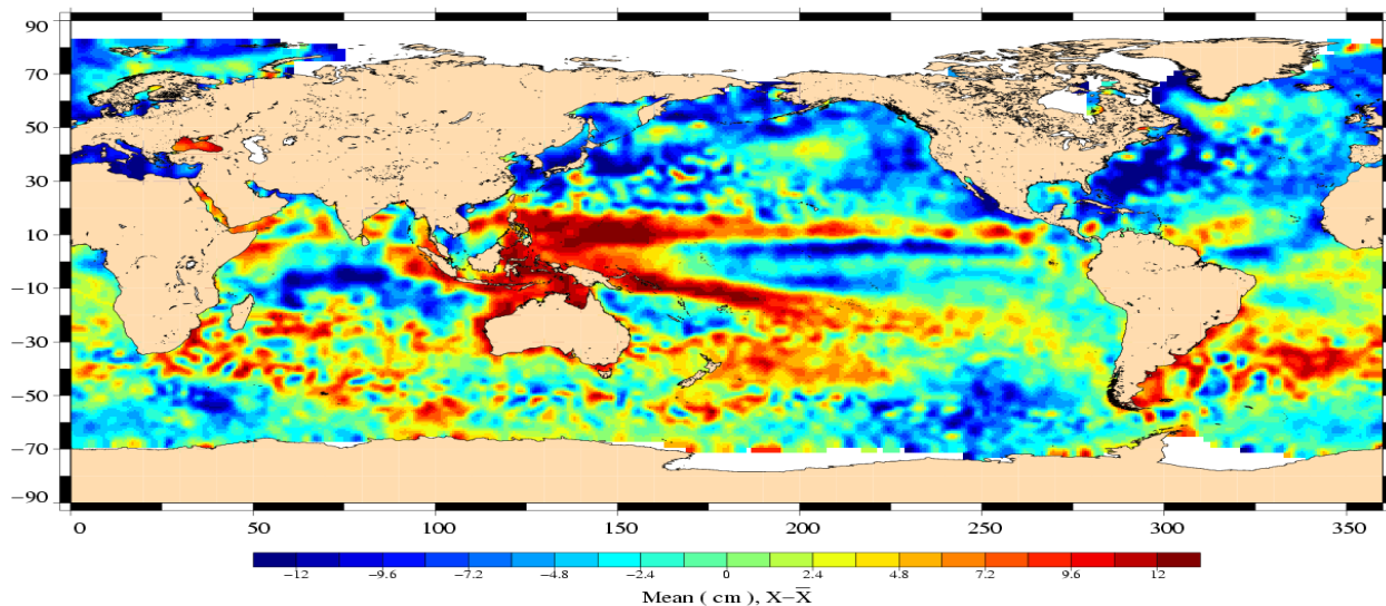
Variability relative to MSS (cm) Envisat Cycle 047 (17/04/2006 to 22/05/2006)
