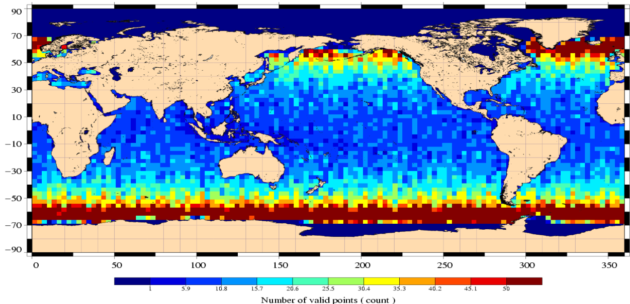
Number of Jason/Envisat 10 days cross-over points Cycle 047 (17/04/2006 – 22/05/2006)
