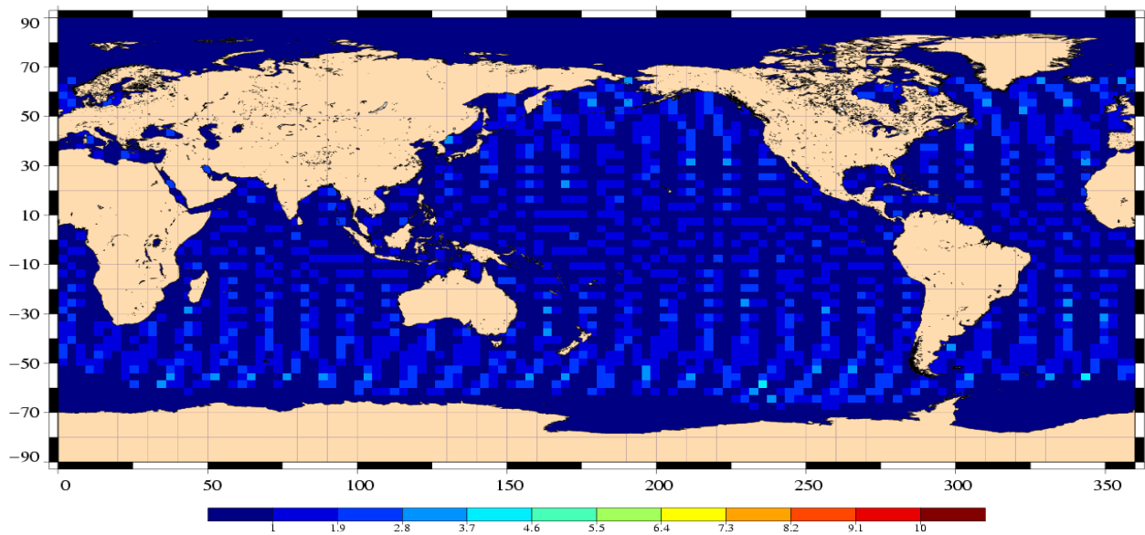
Number of Jason/Envisat 10 days cross-over points Cycle 061 (20/08/2007 – 24/09/2007)
