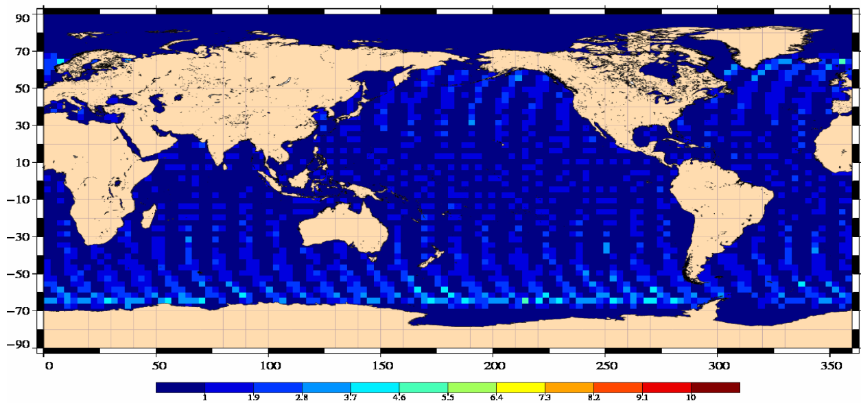
Number of Jason/Envisat 10 days cross-over points Cycle 065 (07/01/2008 – 11/02/2008)
