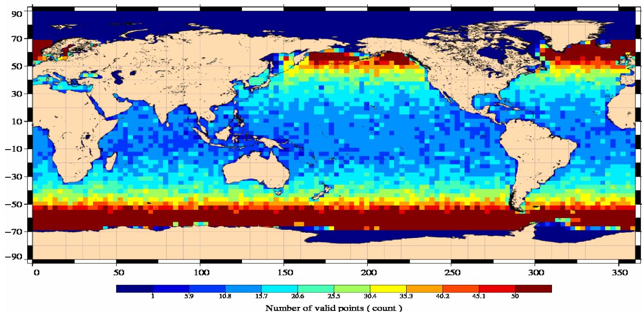
Number of Jason/Envisat 10 days cross-over points Cycle 065 (07/01/2008 – 11/02/2008)
