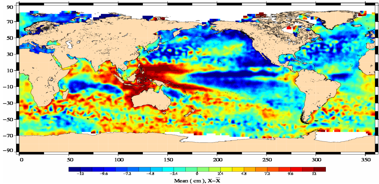
Variability relative to MSS with wave length error (cm) Envisat Cycle 068 (21/04/2008 to 26/05/2008)
