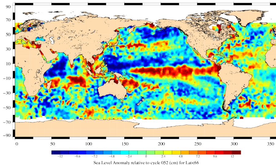
Variability relative to MSS (cm) Cycle 053 EN (09/12/2009 to 19/12/2009)
