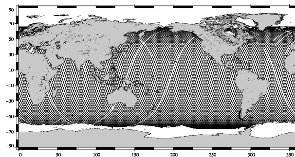
JASON 2 10-day coverage for Jason-2 cycle 1
