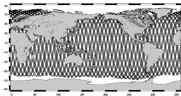
ENVISAT 10-day coverage for Jason-2 cycle 1
