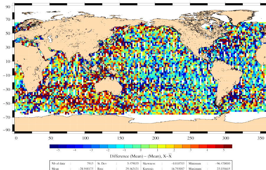
Differences of SLA before orbit error correction J2 – EN (09/12/2009 to 19/12/2009)
