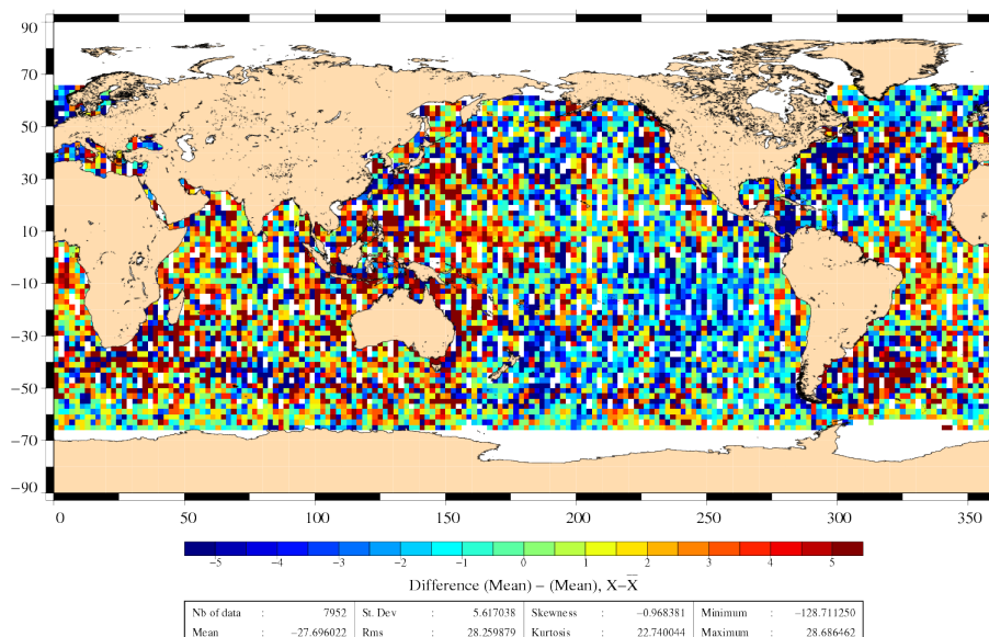
Differences of SLA before orbit error correction J2 – EN (08/01/2010 to 18/01/2010)
