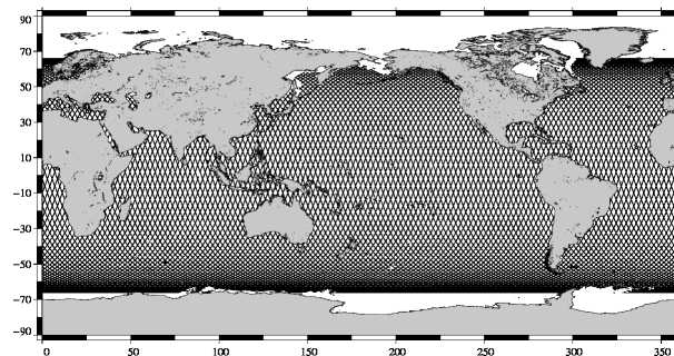
JASON 2 10-day coverage for Jason-2 cycle 57
