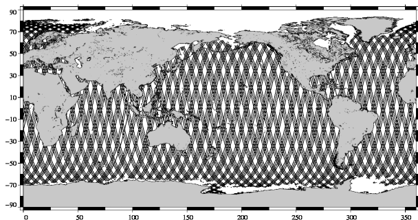
ENVISAT 10-day coverage for Jason-2 cycle 57
