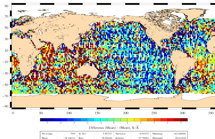
Differences of SLA before orbit error correction J2 – EN (18/01/2010 to 28/01/2010)
