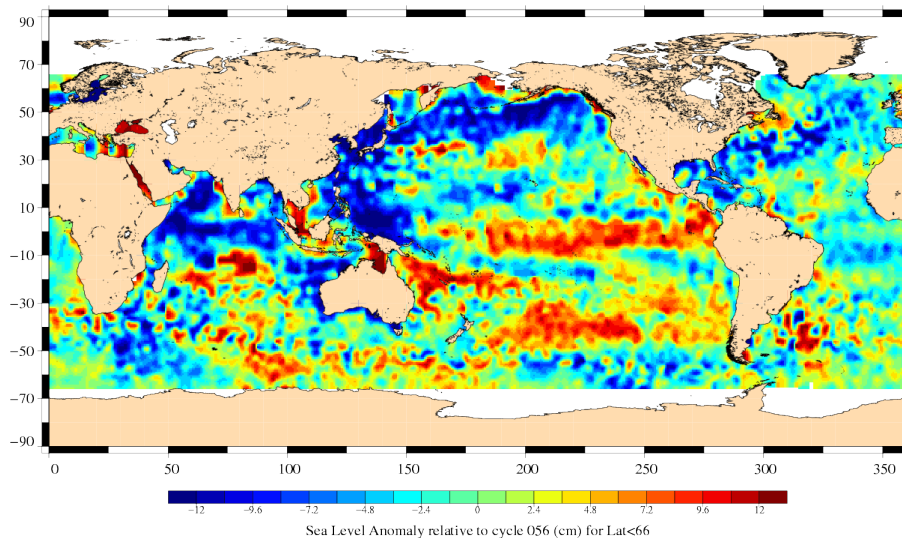
Variability relative to MSS (cm) Cycle 057 EN (18/01/2010 to 28/01/2010)
