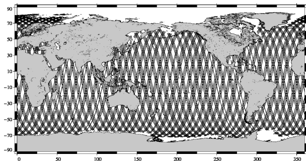
ENVISAT 10-day coverage for Jason-2 cycle 58
