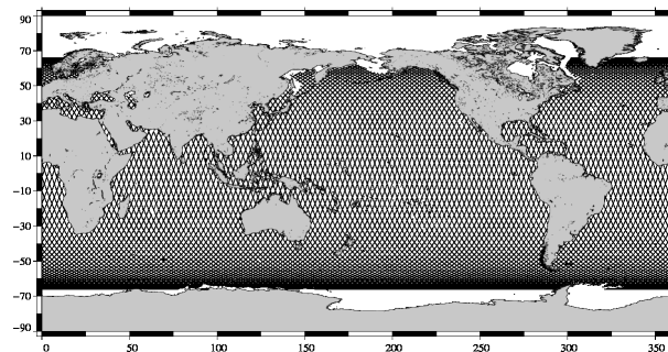
JASON 2 10-day coverage for Jason-2 cycle 58
