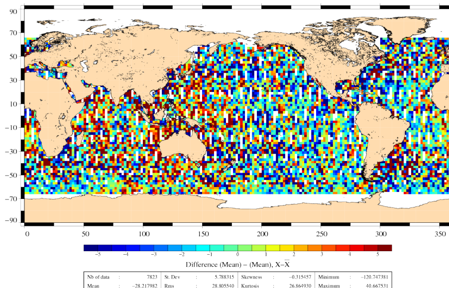
Differences of SLA before orbit error correction J2 – EN (28/01/2010 to 07/02/2010)
