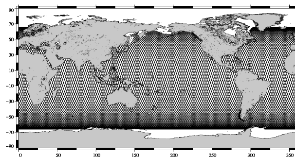
JASON 2 10-day coverage for Jason-2 cycle 59
