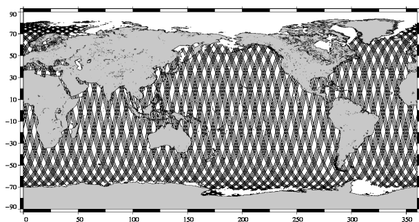
ENVISAT 10-day coverage for Jason-2 cycle 59
