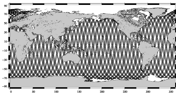
ENVISAT 10-day coverage for Jason-2 cycle 60
