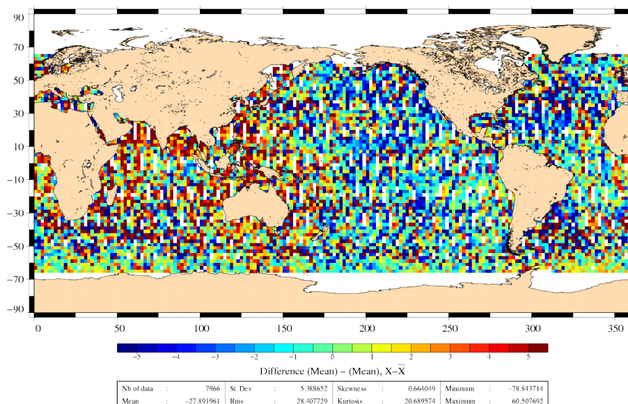
Differences of SLA before orbit error correction J2 – EN (07/02/2010 to 17/02/2010)
