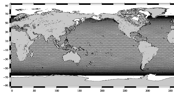
JASON 2 10-day coverage for Jason-2 cycle 60
