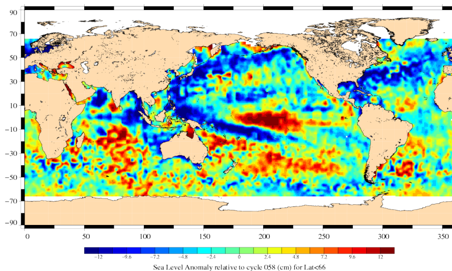
Variability relative to MSS (cm) Cycle 059 EN (07/02/2010 to 17/02/2010)
